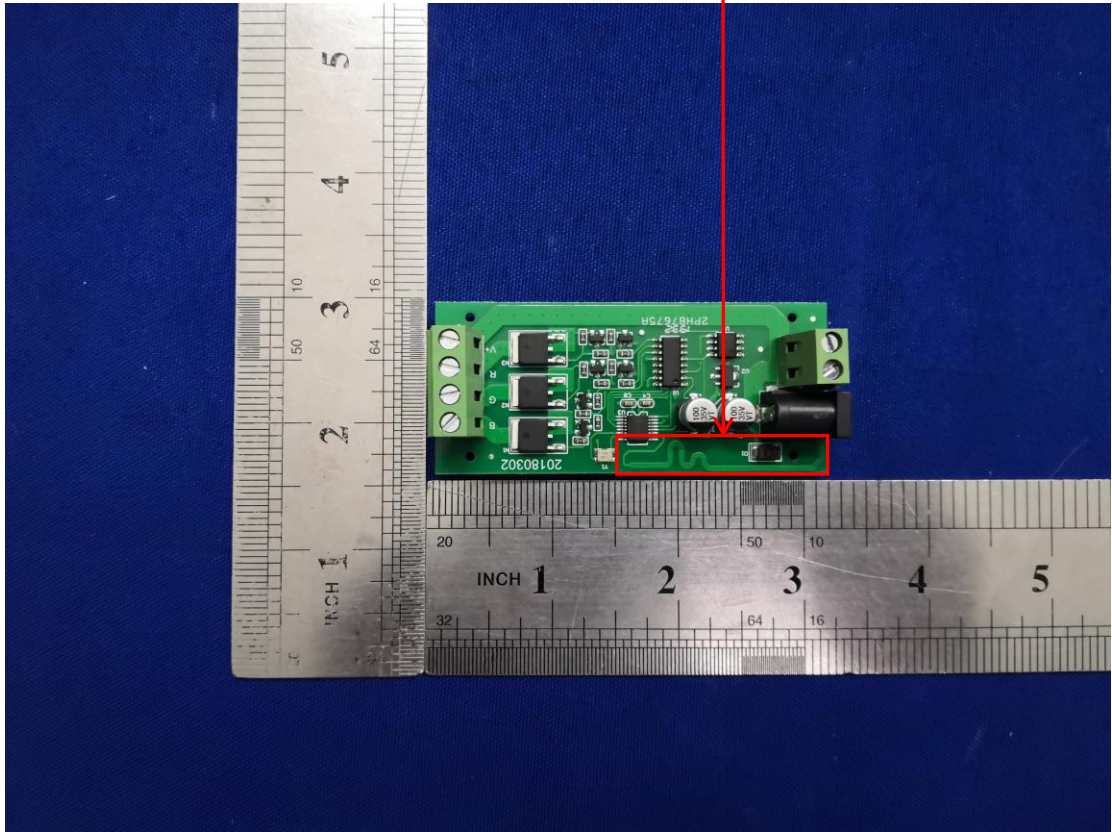
2.4G: PCB Antenna
