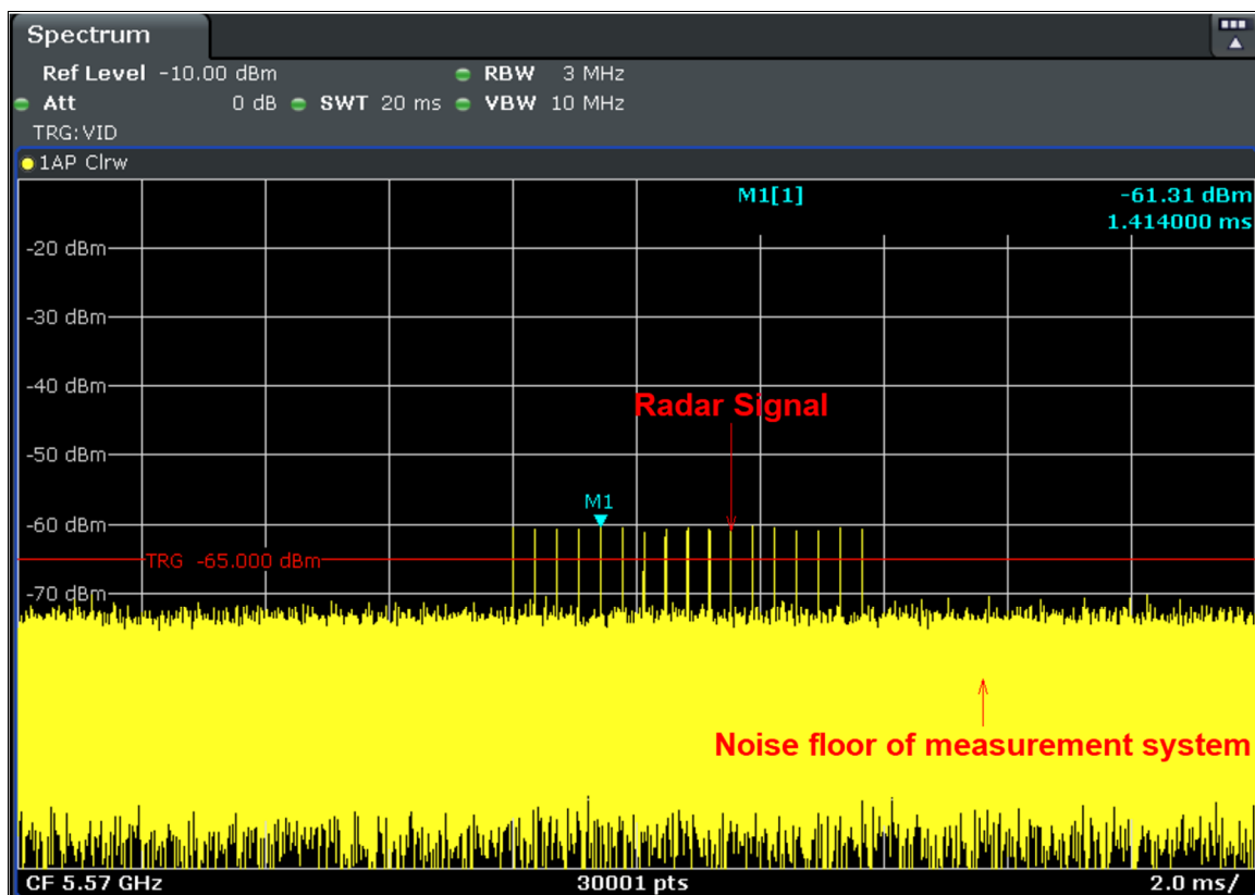
Radar Signal 3
