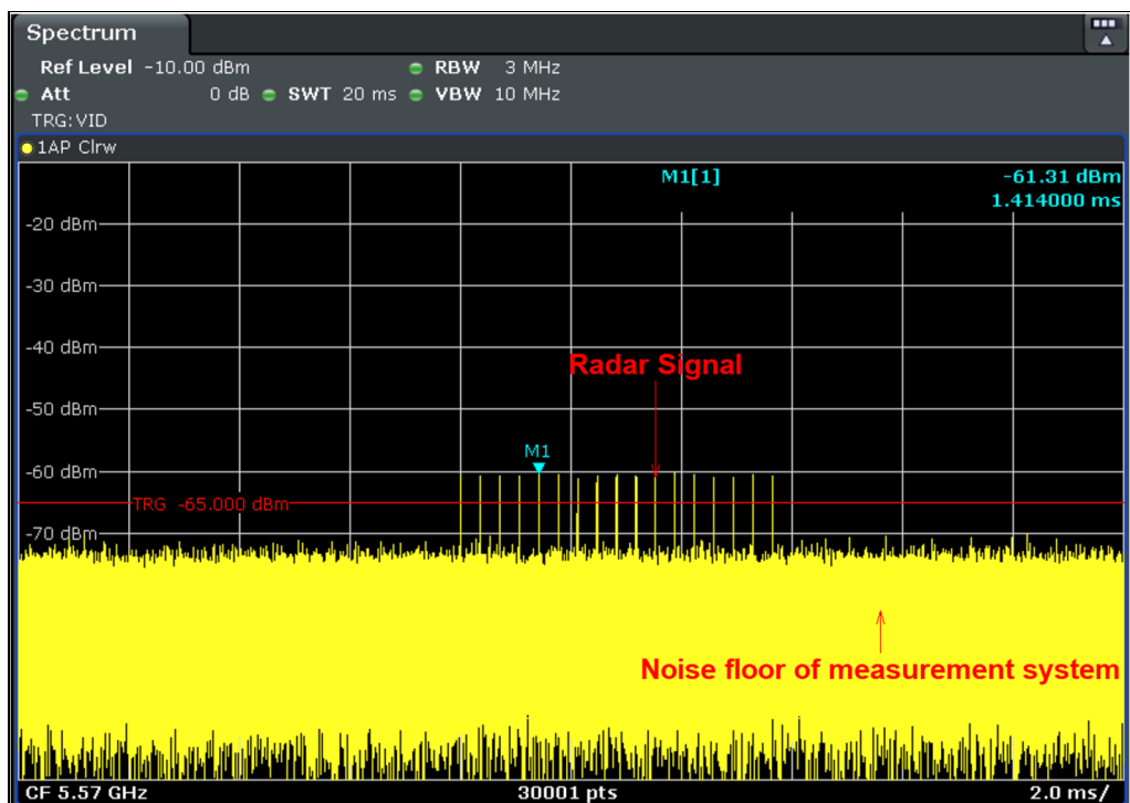
Radar Signal 3
