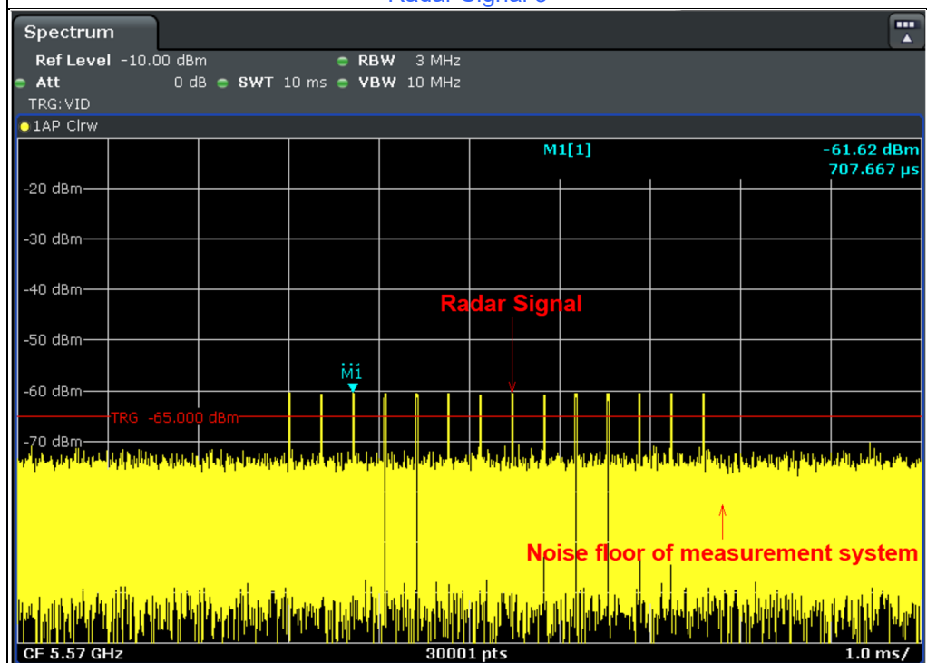
Radar Signal 4
