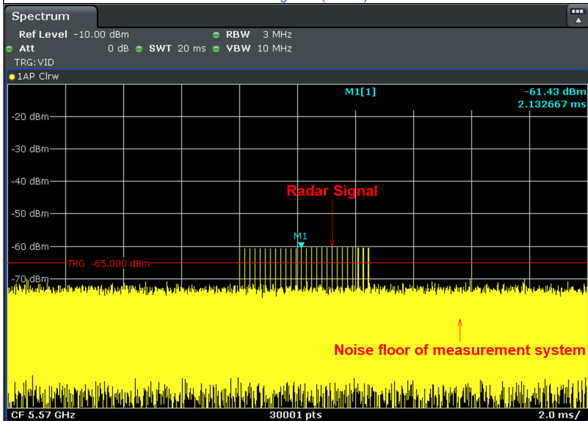
Radar Signal 2
