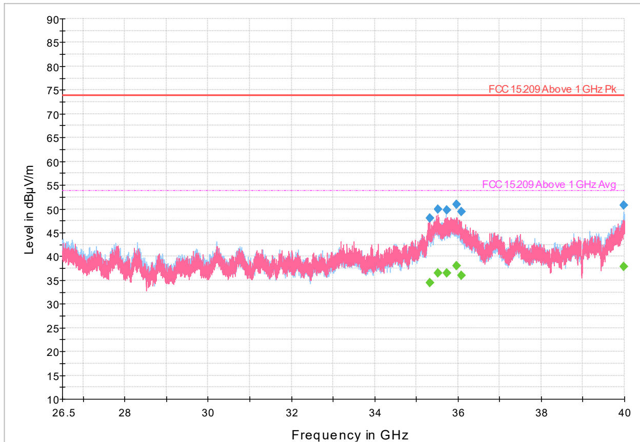
Figure 8.10-50: Radiated emissions spectral plot (26.5 GHz - 40 GHz), 5745 MHz operation
