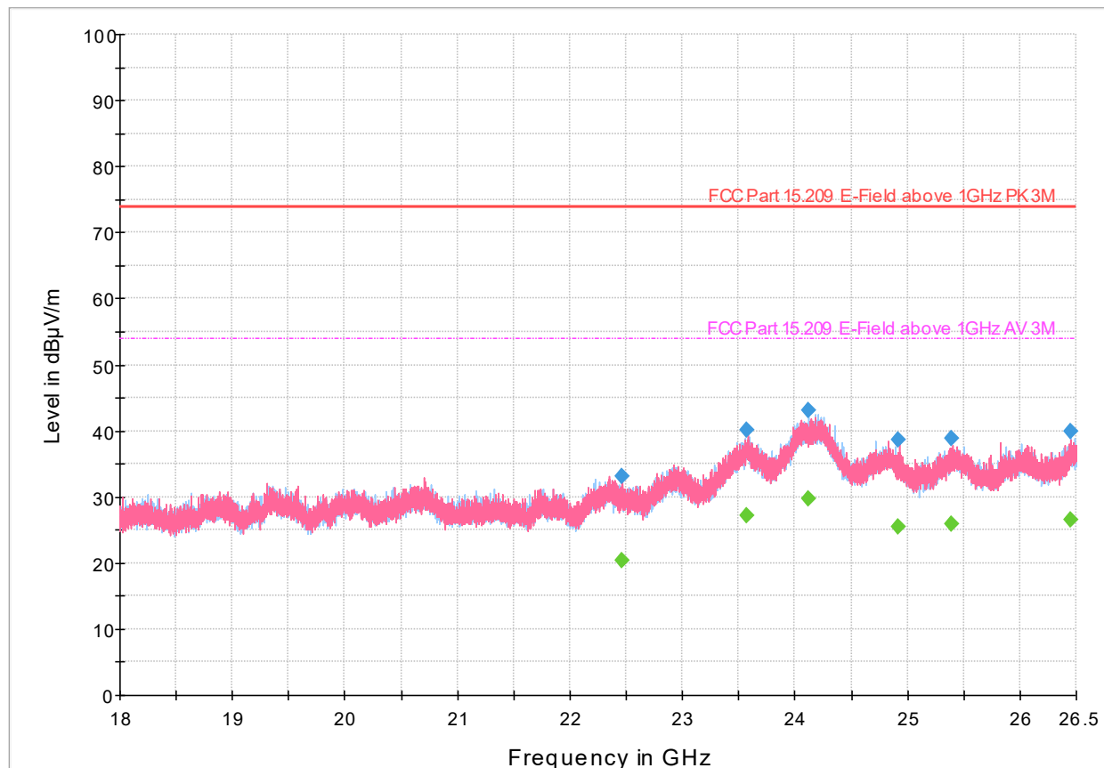
Figure 8.10-49: Radiated emissions spectral plot (18 GHz - 26.5 GHz), 5745 MHz operation
