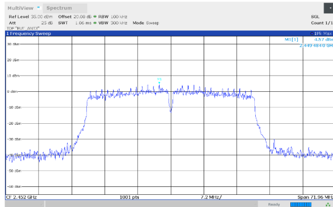
Figure 8.7-47: Authorized band-edge emissions, reference level, 2452 MHz, Antenna 3
