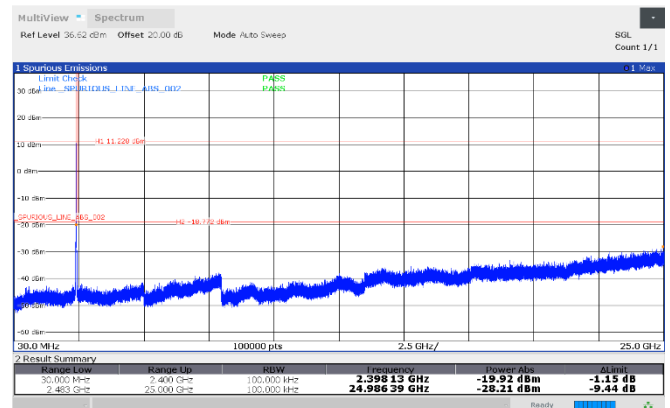
Figure 8.7-98: Conducted antenna port spurious emissions, 2412 MHz, Antenna 3
