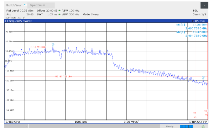
Figure 8.7-16: Authorized band-edge emissions, 2462 MHz, Antenna 1
