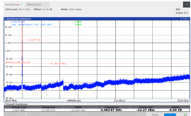
Figure 8.7-84: Conducted antenna port spurious emissions, 2462 MHz, Antenna 3
