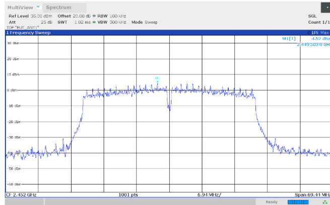
Figure 8.7-39: Authorized band-edge emissions, reference level, 2452 MHz, Antenna 1
