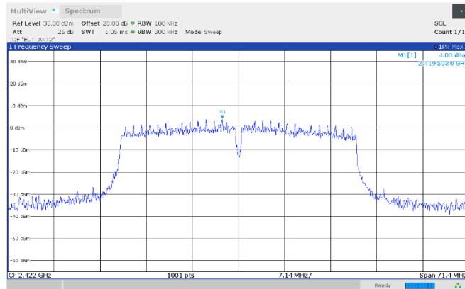
Figure 8.7-41: Authorized band-edge emissions, reference level, 2422 MHz, Antenna 2
