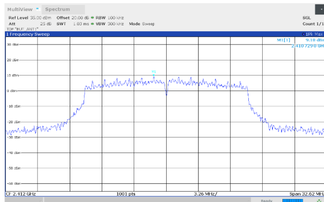
Figure 8.7-13: Authorized band-edge emissions, reference level, 2412 MHz, Antenna 1
