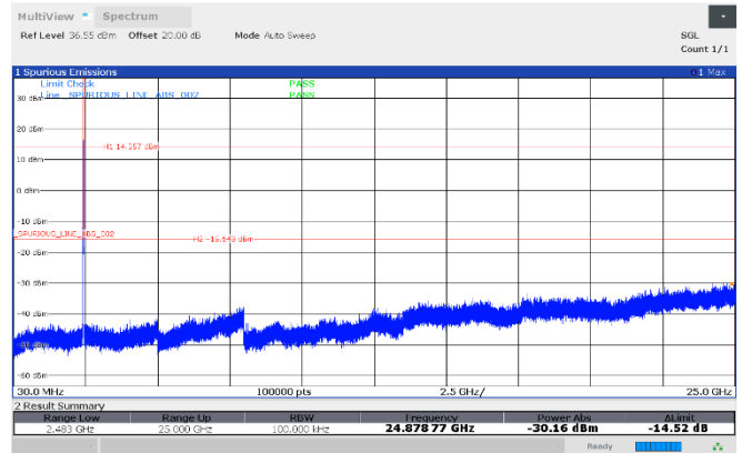
Figure 8.7-58: Conducted antenna port spurious emissions, 2442 MHz, Antenna 2
