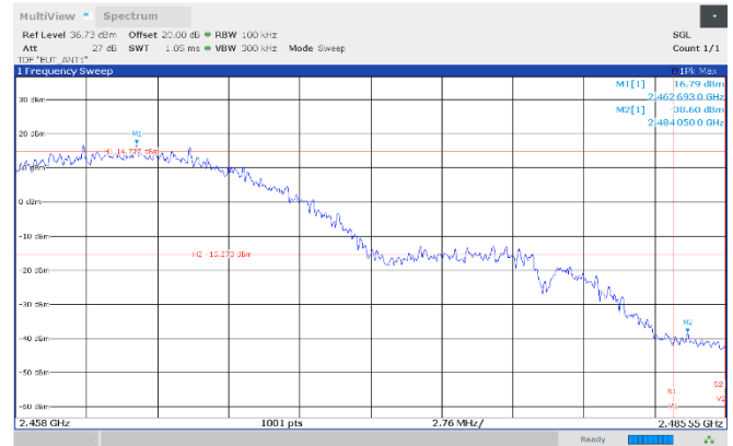
Figure 8.7-4: Authorized band-edge emissions, 2462 MHz, Antenna 1
