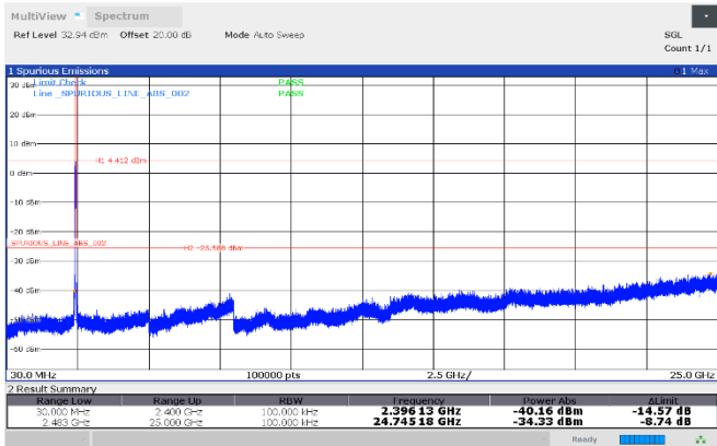
Figure 8.7-118: Conducted antenna port spurious emissions, 2437 MHz, Antenna 3
