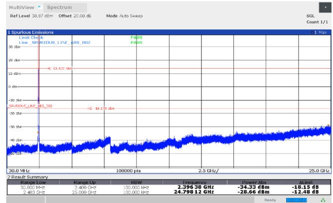
Figure 8.7-82: Conducted antenna port spurious emissions, 2442 MHz, Antenna 3
