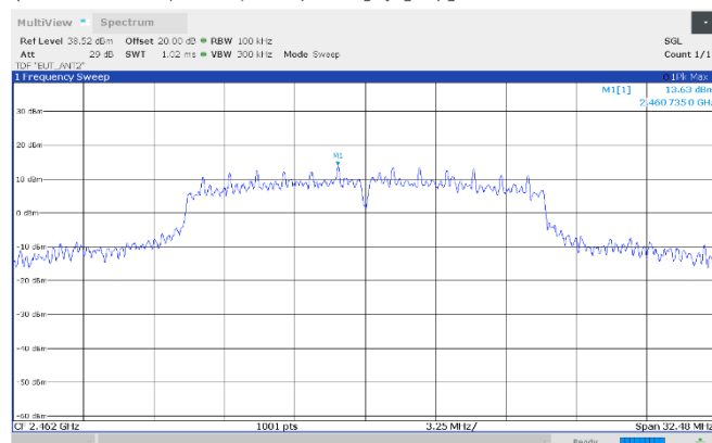
Figure 8.7-19: Authorized band-edge emissions, reference level, 2462 MHz, Antenna 2
