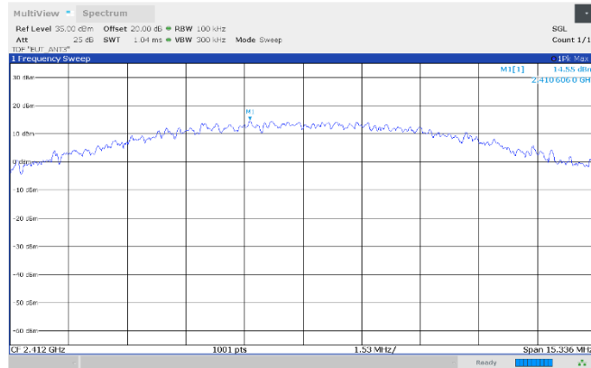
Figure 8.7-9: Authorized band-edge emissions, reference level, 2412 MHz, Antenna 3
