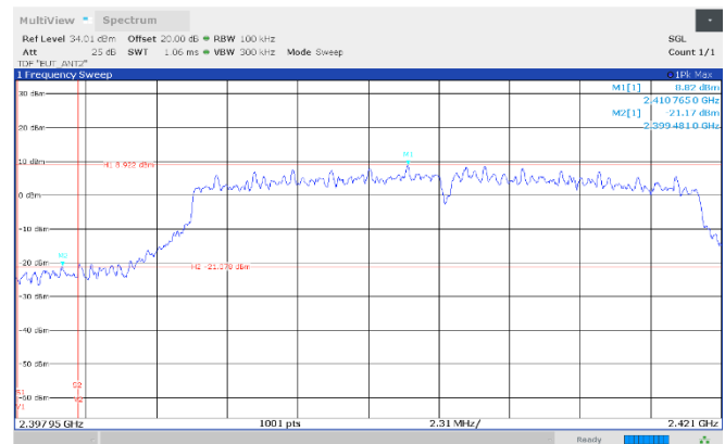
Figure 8.7-18: Authorized band-edge emissions, 2412 MHz, Antenna 2
