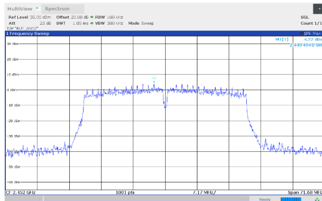
Figure 8.7-43: Authorized band-edge emissions, reference level, 2452 MHz, Antenna 2
