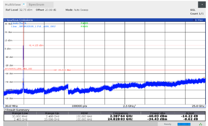
Figure 8.7-112: Conducted antenna port spurious emissions, 2437 MHz, Antenna 2
