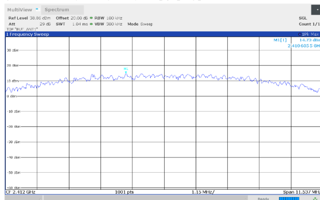
Figure 8.7-49: Conducted antenna port spurious emissions, reference level, 2412 MHz, Antenna 1
