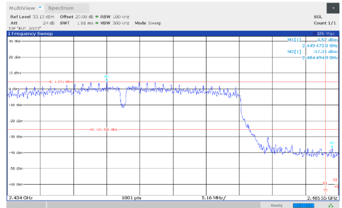
Figure 8.7-48: Authorized band-edge emissions, 2452 MHz, Antenna 3
