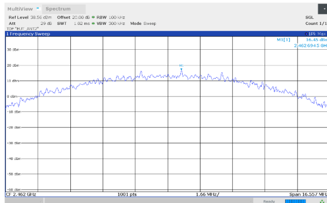
Figure 8.7-7: Authorized band-edge emissions, reference level, 2462 MHz, Antenna 2
