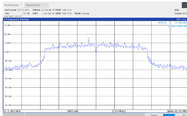
Figure 8.7-31: Authorized band-edge emissions, reference level, 2462 MHz, Antenna 2
