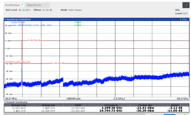
Figure 8.7-92: Conducted antenna port spurious emissions, 2412 MHz, Antenna 2
