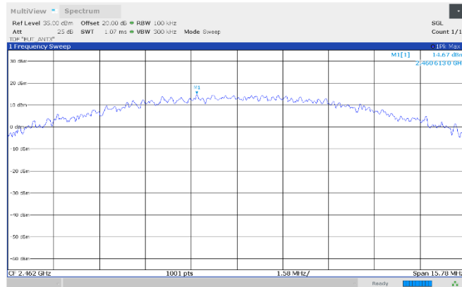
Figure 8.7-11: Authorized band-edge emissions, reference level, 2462 MHz, Antenna 3
