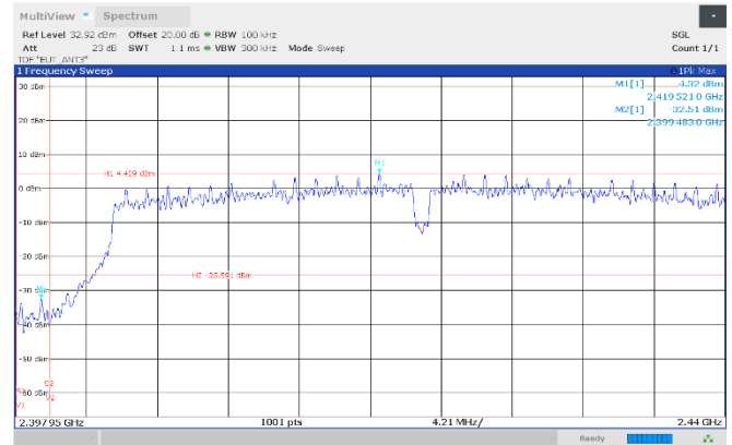
Figure 8.7-46: Authorized band-edge emissions, 2422 MHz, Antenna 3
