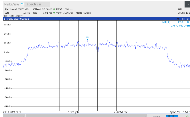
Figure 8.7-87: Conducted antenna port spurious emissions, reference level, 2442 MHz, Antenna 1
