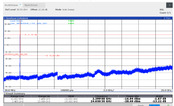
Figure 8.7-50: Conducted antenna port spurious emissions, 2412 MHz, Antenna 1
