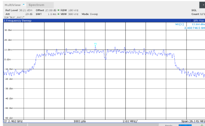
Figure 8.7-89: Conducted antenna port spurious emissions, reference level, 2462 MHz, Antenna 1
