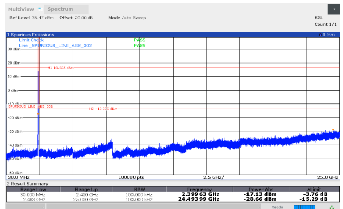
Figure 8.7-62: Conducted antenna port spurious emissions, 2412 MHz, Antenna 3
