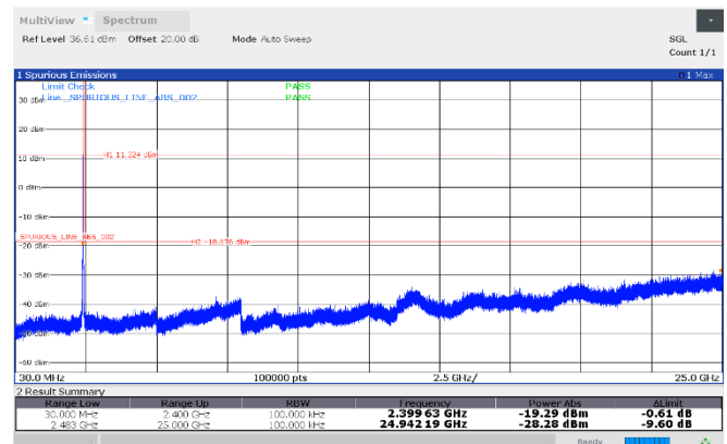
Figure 8.7-86: Conducted antenna port spurious emissions, 2412 MHz, Antenna 1
