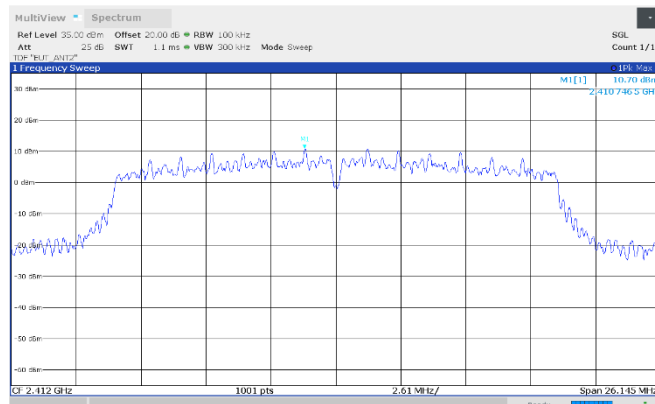
Figure 8.7-91: Conducted antenna port spurious emissions, reference level, 2412 MHz, Antenna 2
