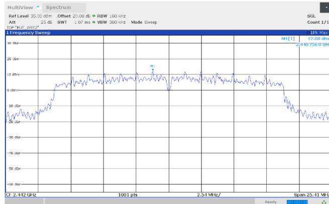
Figure 8.7-93: Conducted antenna port spurious emissions, reference level, 2442 MHz, Antenna 2
