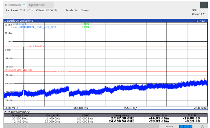
Figure 8.7-114: Conducted antenna port spurious emissions, 2452 MHz, Antenna 2
