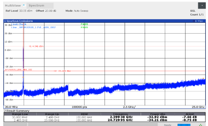
Figure 8.7-116: Conducted antenna port spurious emissions, 2422 MHz, Antenna 3
