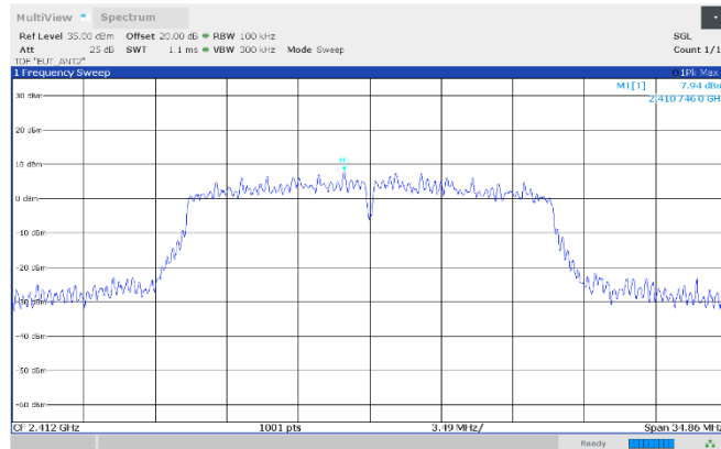
Figure 8.7-29: Authorized band-edge emissions, reference level, 2412 MHz, Antenna 2
