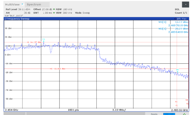
Figure 8.7-24: Authorized band-edge emissions, 2462 MHz, Antenna 3
