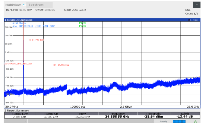
Figure 8.7-54: Conducted antenna port spurious emissions, 2462 MHz, Antenna 1
