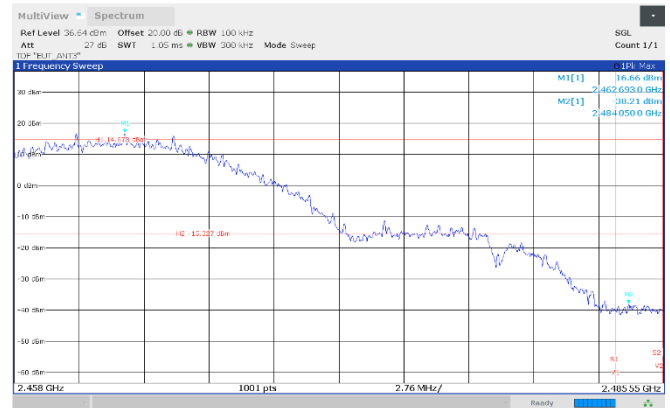
Figure 8.7-12: Authorized band-edge emissions, 2462 MHz, Antenna 3
