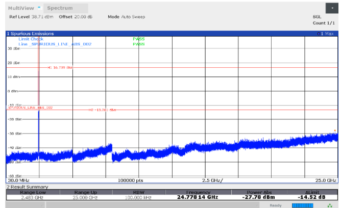
Figure 8.7-60: Conducted antenna port spurious emissions, 2462 MHz, Antenna 2
