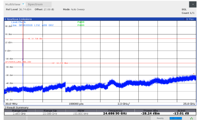
Figure 8.7-52: Conducted antenna port spurious emissions, 2442 MHz, Antenna 1
