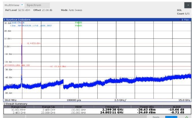
Figure 8.7-110: Conducted antenna port spurious emissions, 2422 MHz, Antenna 2
