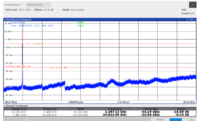
Figure 8.7-108: Conducted antenna port spurious emissions, 2452 MHz, Antenna 1
