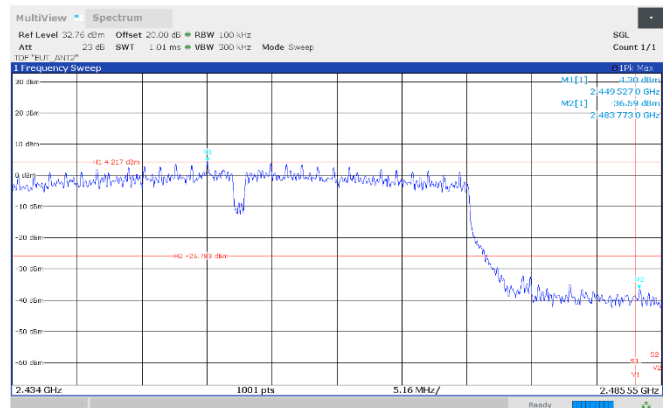
Figure 8.7-44: Authorized band-edge emissions, 2452 MHz, Antenna 2
