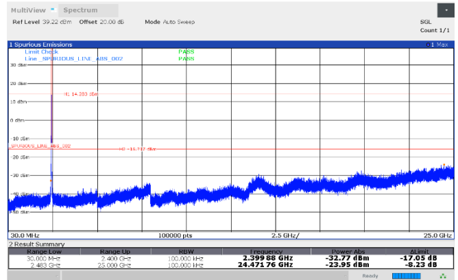
Figure 8.7-70: Conducted antenna port spurious emissions, 2442 MHz, Antenna 1
