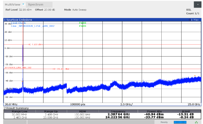
Figure 8.7-106: Conducted antenna port spurious emissions, 2437 MHz, Antenna 1
