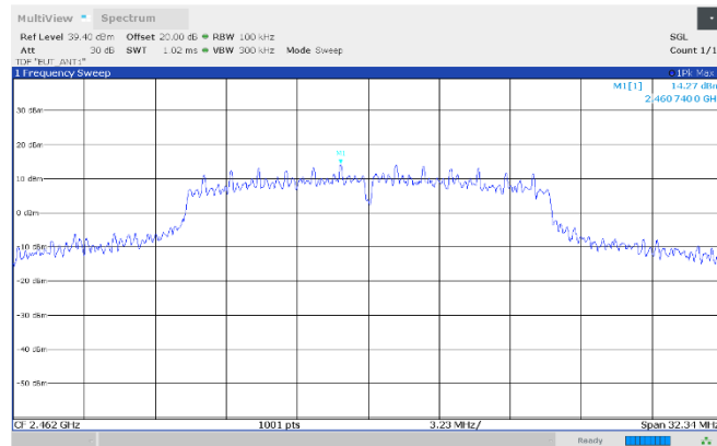
Figure 8.7-15: Authorized band-edge emissions, reference level, 2462 MHz, Antenna 1
