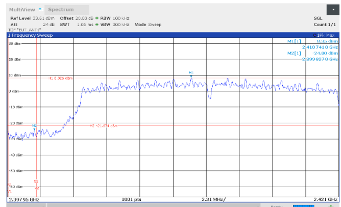
Figure 8.7-26: Authorized band-edge emissions, 2412 MHz, Antenna 1
