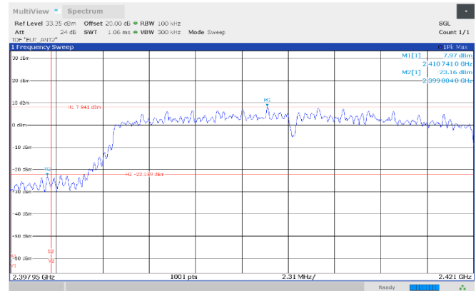
Figure 8.7-30: Authorized band-edge emissions, 2412 MHz, Antenna 2
