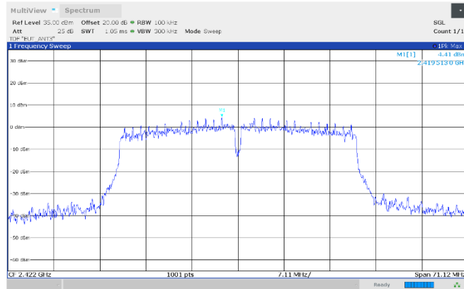
Figure 8.7-45: Authorized band-edge emissions, reference level, 2422 MHz, Antenna 3
