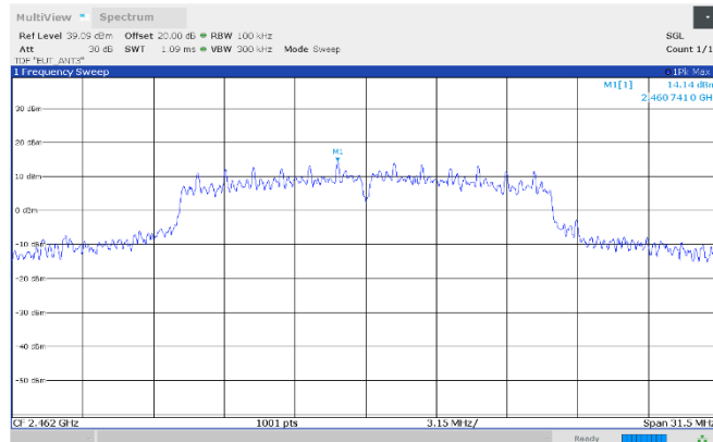
Figure 8.7-23: Authorized band-edge emissions, reference level, 2462 MHz, Antenna 3
