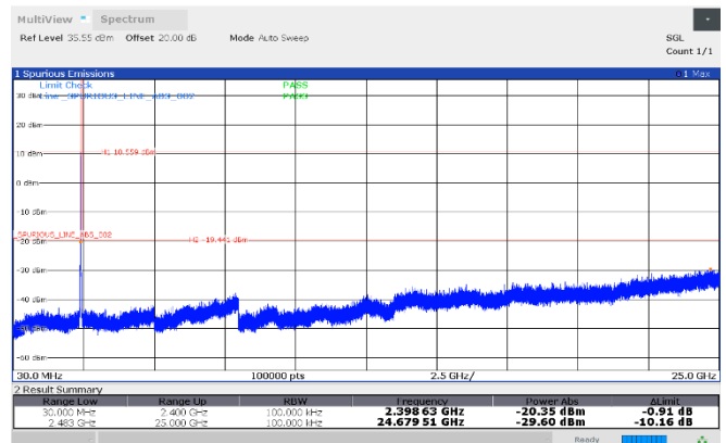
Figure 8.7-80: Conducted antenna port spurious emissions, 2412 MHz, Antenna 3
