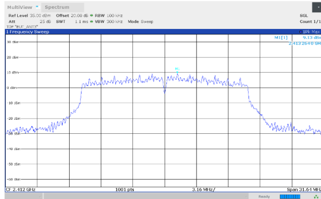
Figure 8.7-21: Authorized band-edge emissions, reference level, 2412 MHz, Antenna 3
