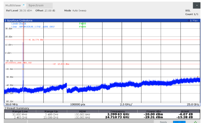
Figure 8.7-56: Conducted antenna port spurious emissions, 2412 MHz, Antenna 2
