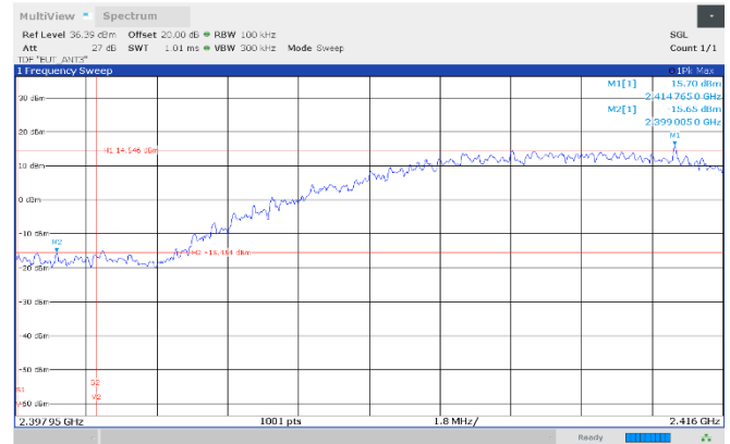
Figure 8.7-10: Authorized band-edge emissions, 2412 MHz, Antenna 3
