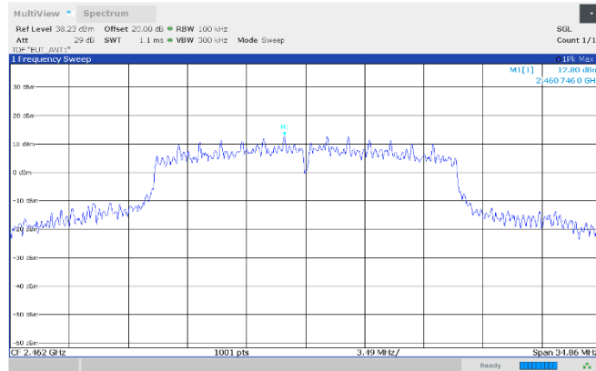
Figure 8.7-27: Authorized band-edge emissions, reference level, 2462 MHz, Antenna 1
