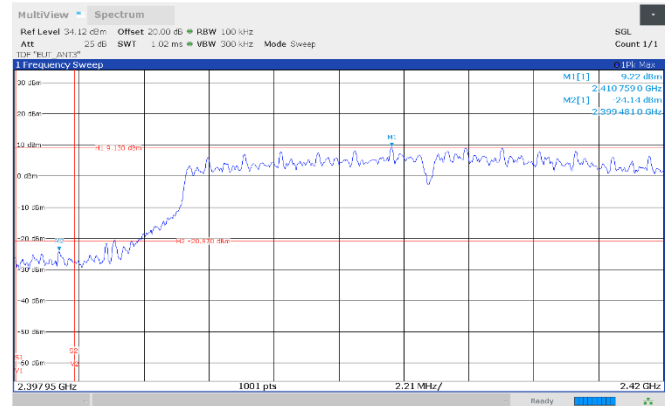
Figure 8.7-22: Authorized band-edge emissions, 2412 MHz, Antenna 3
