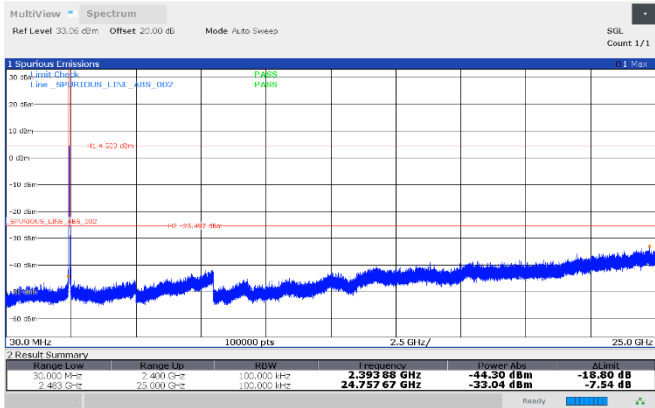
Figure 8.7-120: Conducted antenna port spurious emissions, 2452 MHz, Antenna 3
