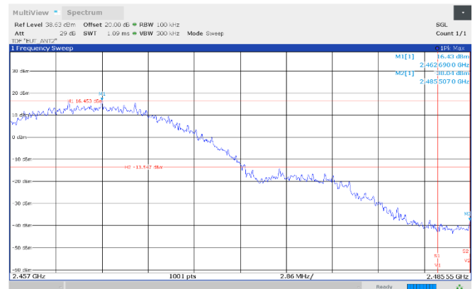
Figure 8.7-8: Authorized band-edge emissions, 2462 MHz, Antenna 2
