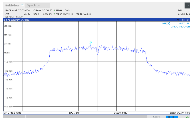
Figure 8.7-17: Authorized band-edge emissions, reference level, 2412 MHz, Antenna 2
