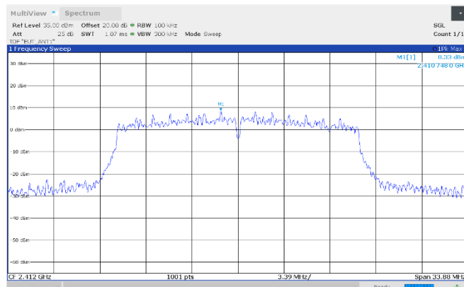
Figure 8.7-25: Authorized band-edge emissions, reference level, 2412 MHz, Antenna 1
