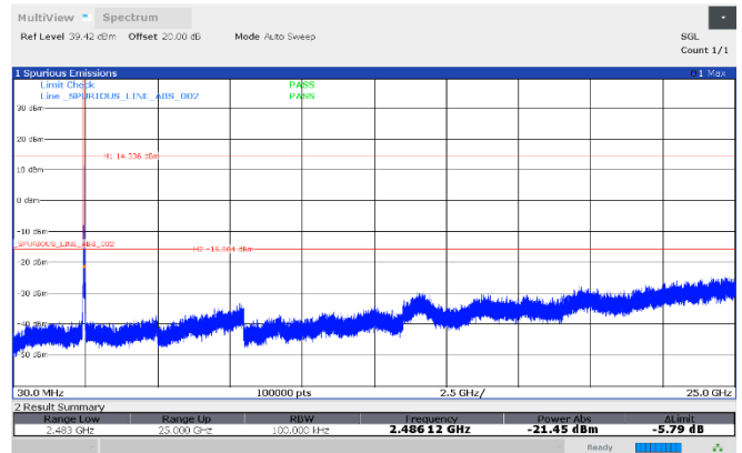
Figure 8.7-72: Conducted antenna port spurious emissions, 2462 MHz, Antenna 1
