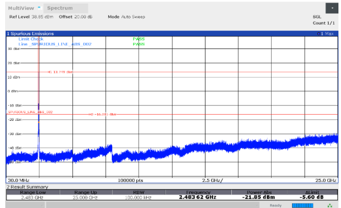
Figure 8.7-78: Conducted antenna port spurious emissions, 2462 MHz, Antenna 2
