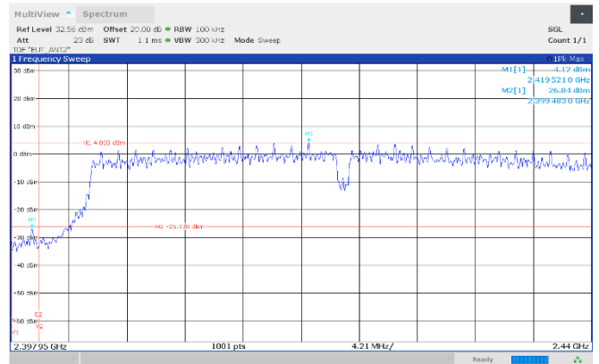
Figure 8.7-42: Authorized band-edge emissions, 2422 MHz, Antenna 2
