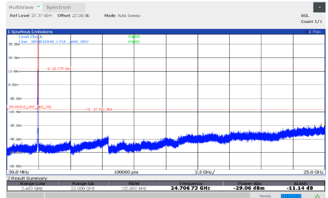
Figure 8.7-94: Conducted antenna port spurious emissions, 2442 MHz, Antenna 2
