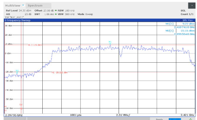
Figure 8.7-14: Authorized band-edge emissions, 2412 MHz, Antenna 1
