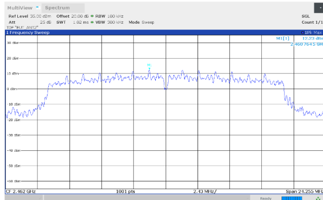
Figure 8.7-95: Conducted antenna port spurious emissions, reference level, 2462 MHz, Antenna 2
