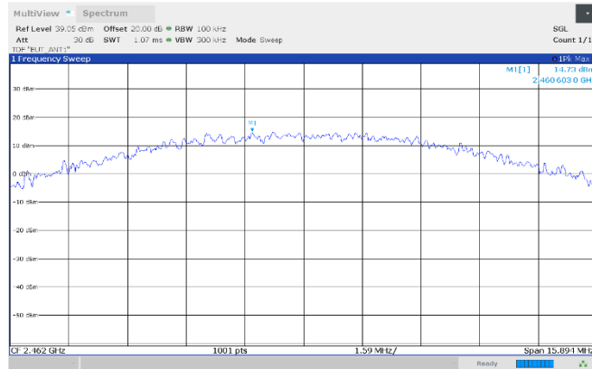
Figure 8.7-3: Authorized band-edge emissions, reference level, 2462 MHz, Antenna 1
