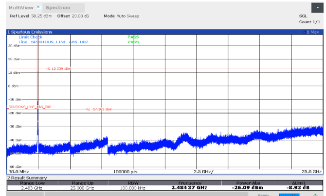
Figure 8.7-90: Conducted antenna port spurious emissions, 2462 MHz, Antenna 1
