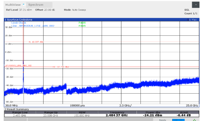
Figure 8.7-96: Conducted antenna port spurious emissions, 2462 MHz, Antenna 2
