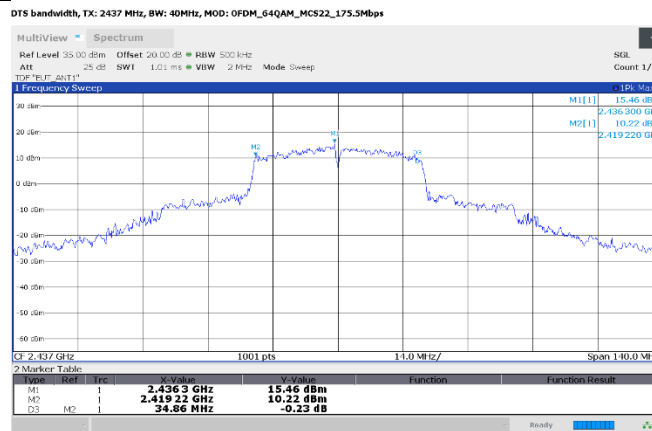
Figure 8.5-4: Minimum 6 dB bandwidth, IEEE 802.11n HT40 (CDD mode), minimum measured DTS bandwidth
