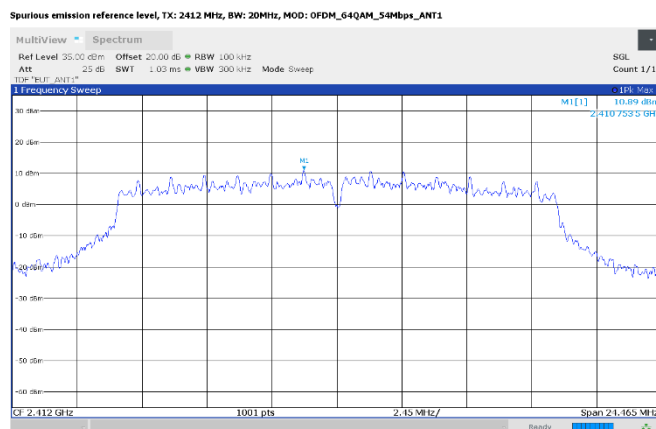
Figure 8.7-67: Conducted antenna port spurious emissions, reference level, 2412 MHz, Antenna 1
