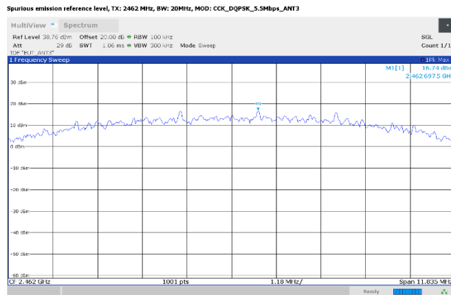
Figure 8.7-65: Conducted antenna port spurious emissions, reference level, 2462 MHz, Antenna 3
