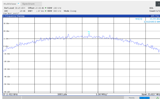
Figure 8.7-5: Authorized band-edge emissions, reference level, 2412 MHz, Antenna 2
