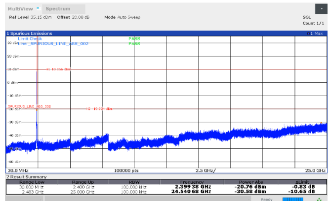
Figure 8.7-74: Conducted antenna port spurious emissions, 2412 MHz, Antenna 2
