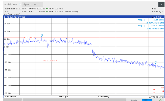
Figure 8.7-32: Authorized band-edge emissions, 2462 MHz, Antenna 2
