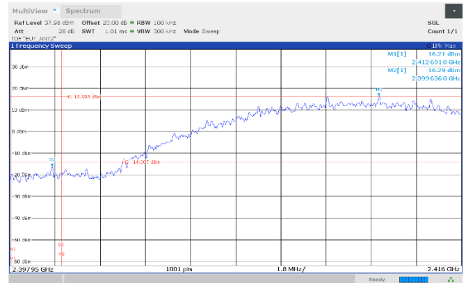
Figure 8.7-6: Authorized band-edge emissions, 2412 MHz, Antenna 2
