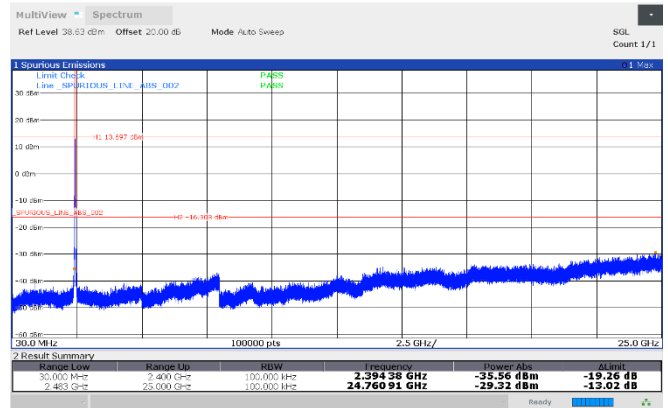
Figure 8.7-76: Conducted antenna port spurious emissions, 2442 MHz, Antenna 2
