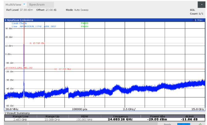
Figure 8.7-88: Conducted antenna port spurious emissions, 2442 MHz, Antenna 1
