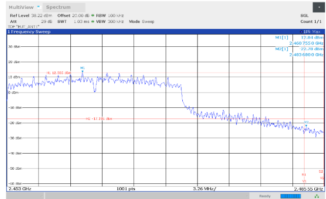
Figure 8.7-28: Authorized band-edge emissions, 2462 MHz, Antenna 1
