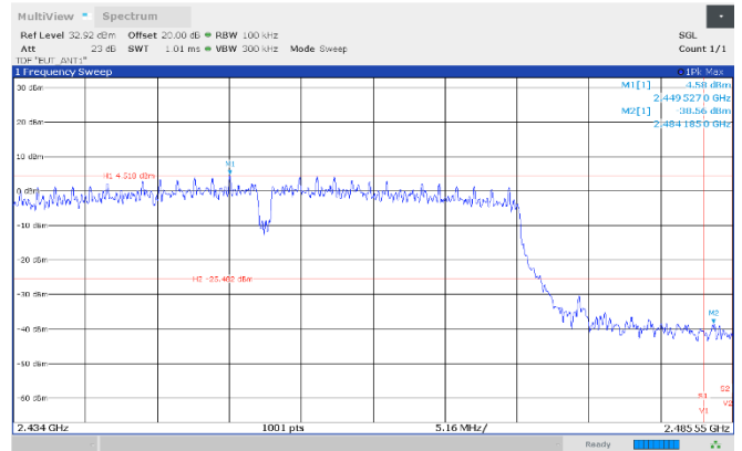
Figure 8.7-40: Authorized band-edge emissions, 2452 MHz, Antenna 1
