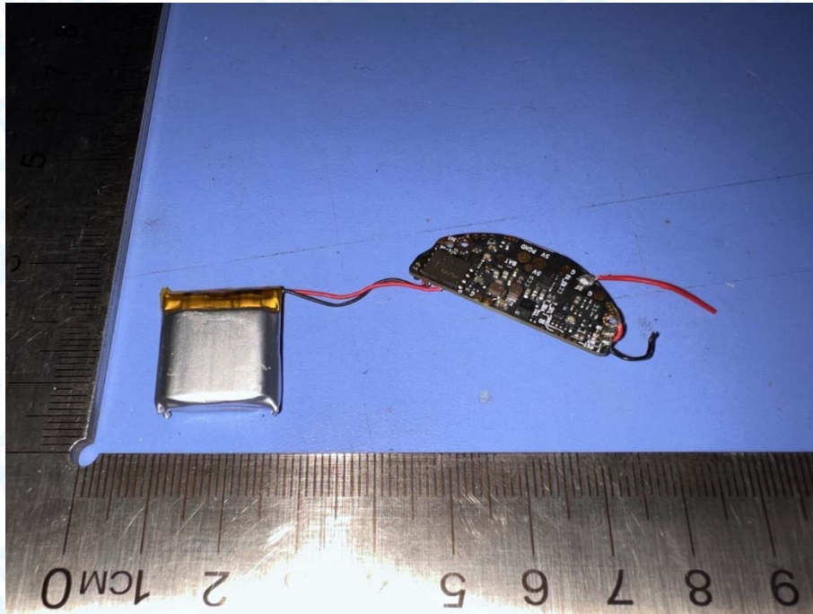
Photo 8 Internal of PCB&Battery
