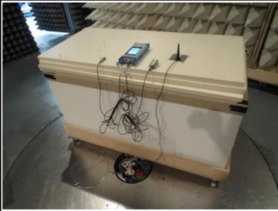
TEST SETUP - Radiated emissions - 1-13GHz - Mode 2 Configuration 2 - table setup
