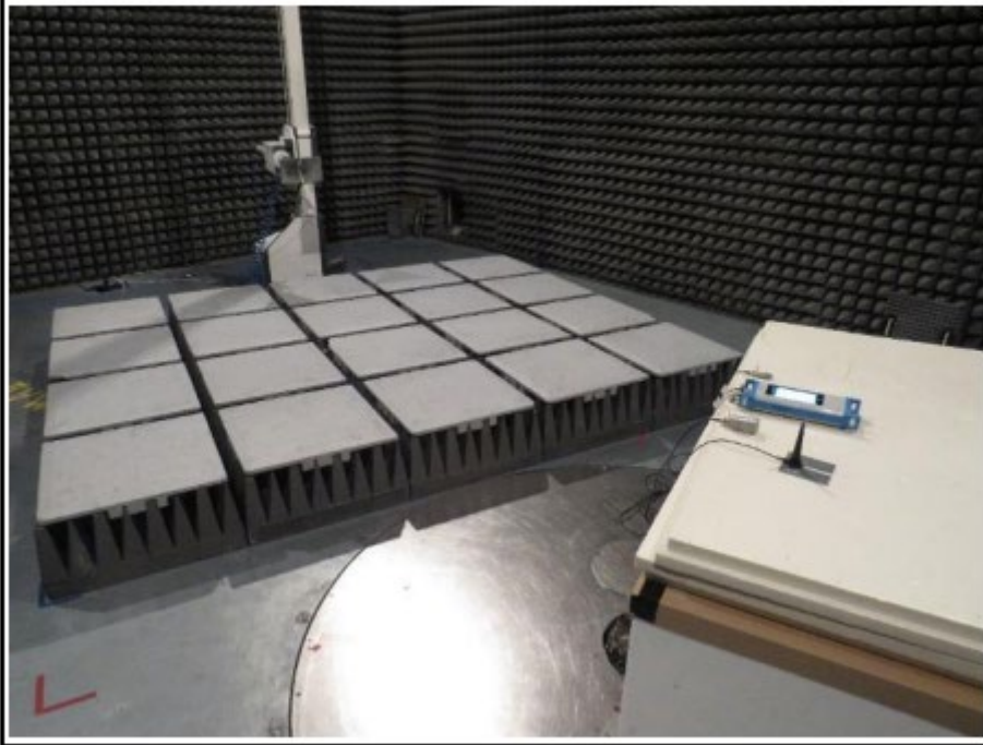
TEST SETUP - Radiated emissions - 1-13GHz - Mode 2 Configuration 2
