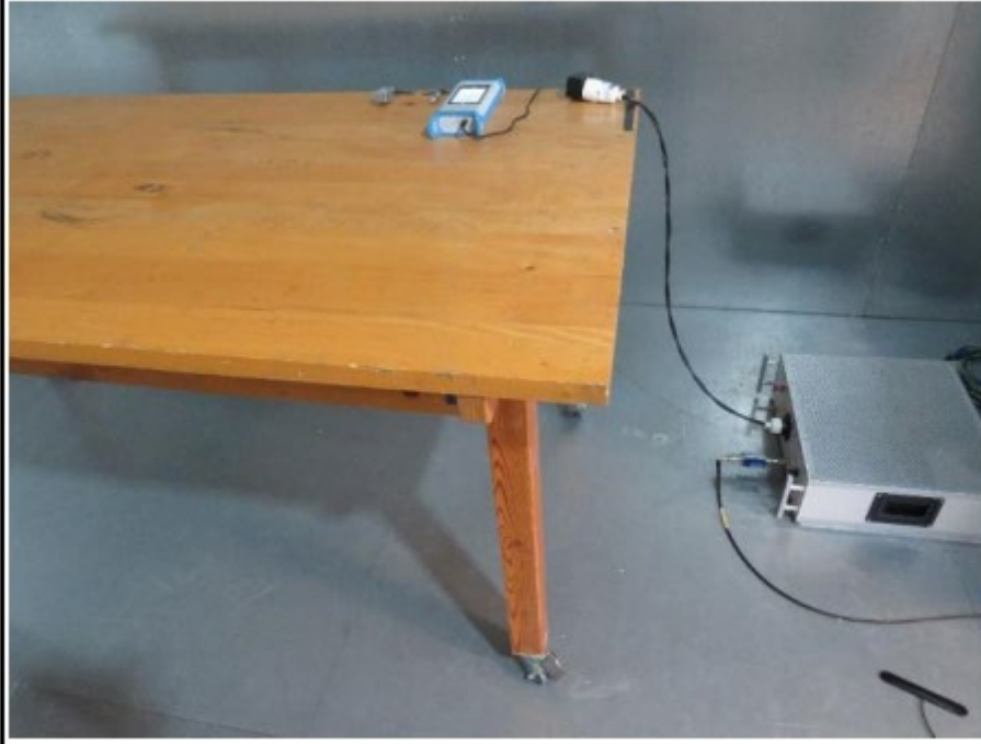
TEST SETUP - Conducted emission
