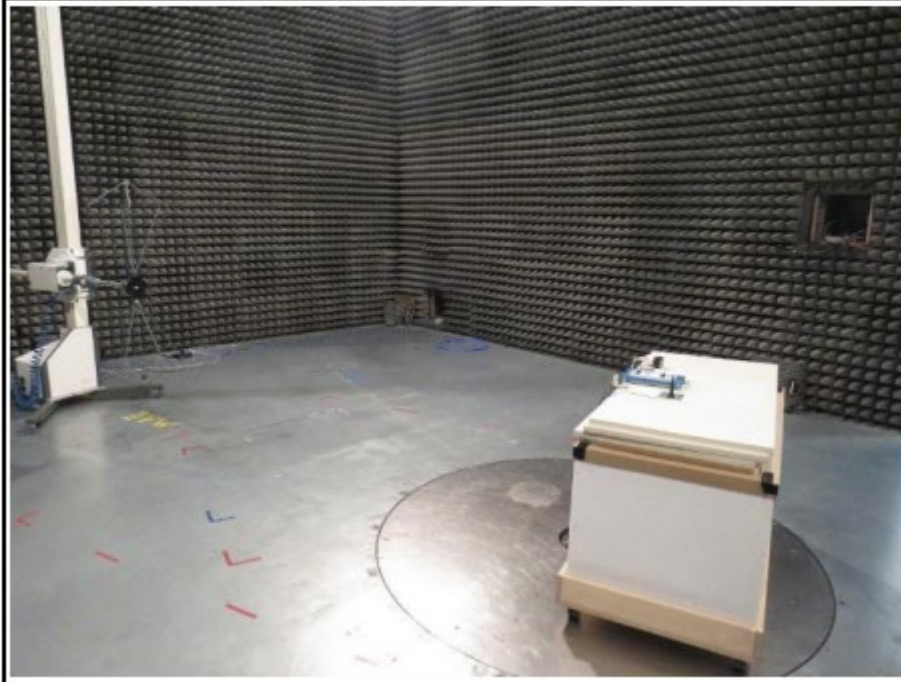
TEST SETUP - Radiated emission - 30-200MHz - Mode 1 Configuration 1
