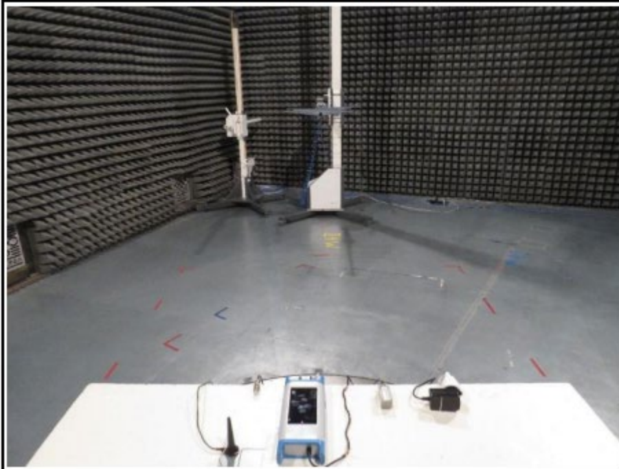
TEST SETUP - Radiated emission - 200MHz-1GHz - Mode 1 Configuration 1 - Table setup
