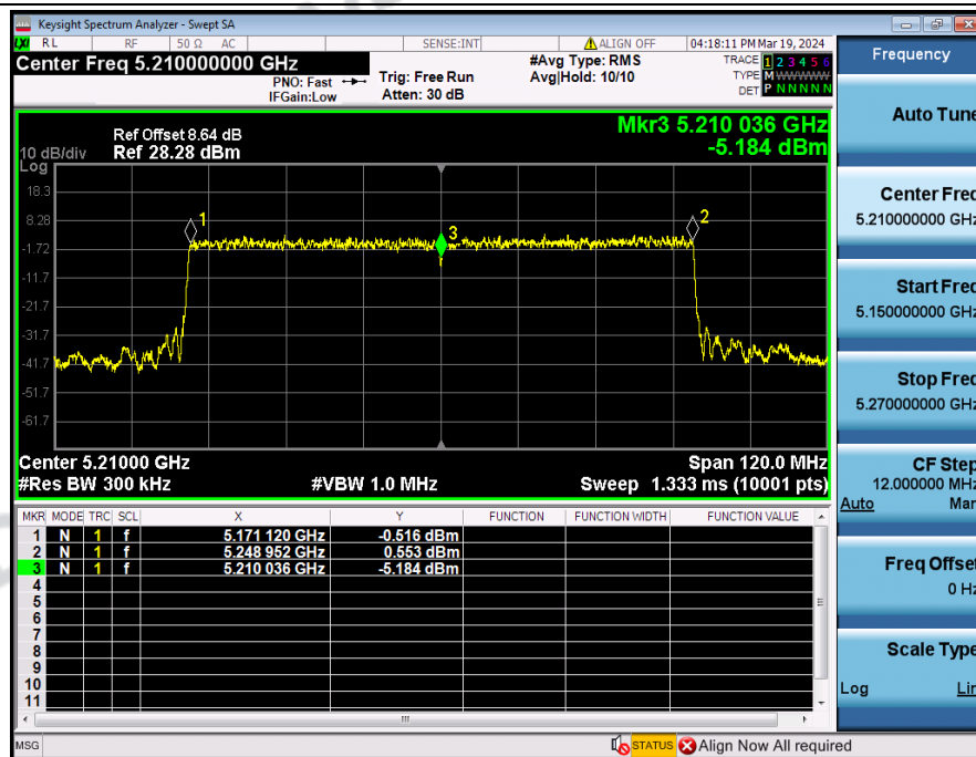
Frequency_Stability_NVNT_ANT3_802_11ax(HE80)_5210
