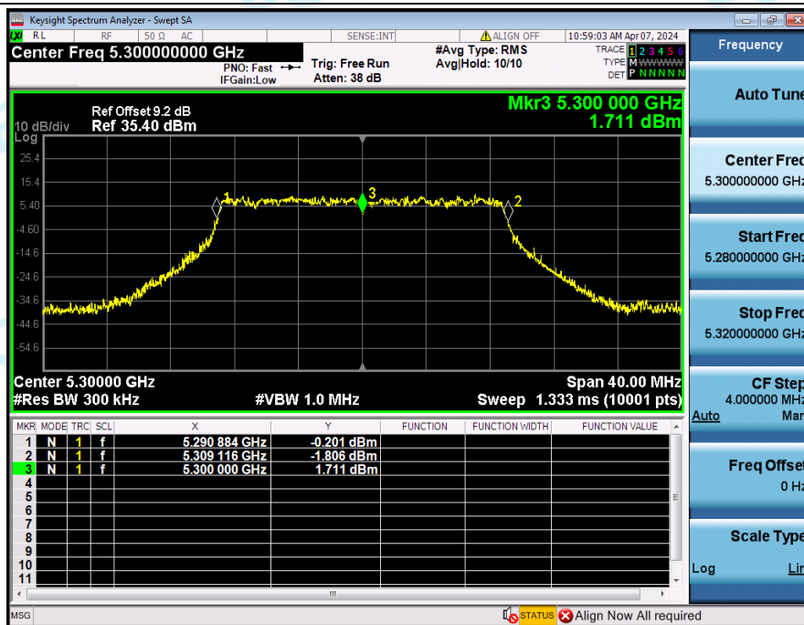
Frequency_Stability_NVNT_ANT3_802_11ac(VHT20)_5300
