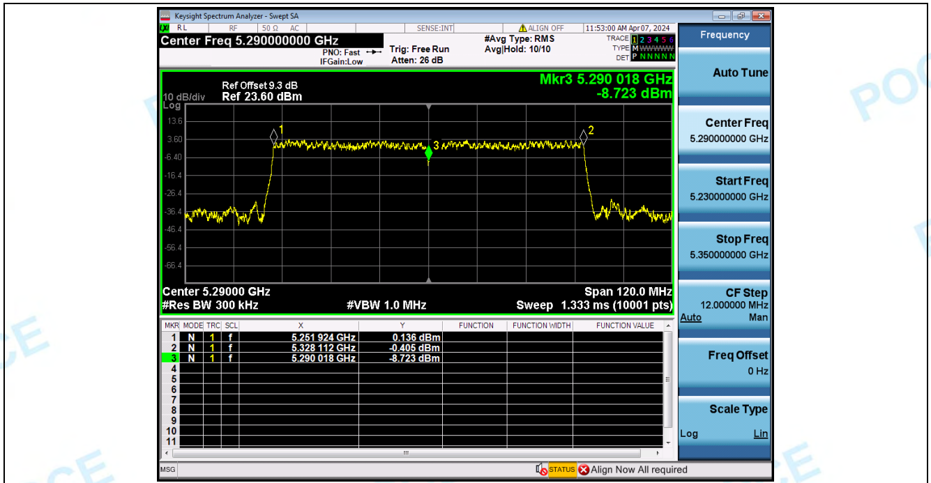
Frequency_Stability_NVNT_ANT1_802_11ax(HE80)_5290
