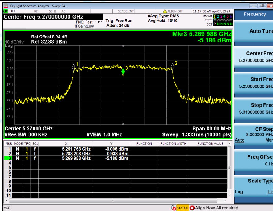
Frequency_Stability_NVNT_ANT3_802_11n(HT40)_5270
