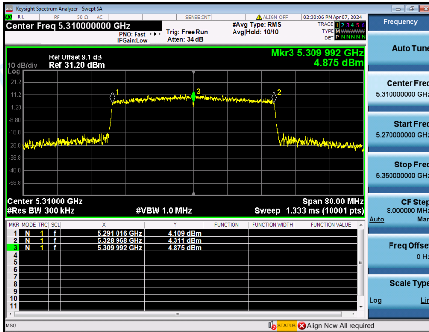
Frequency_Stability_NVNT_ANT3_802_11ax(HE40)_5310
