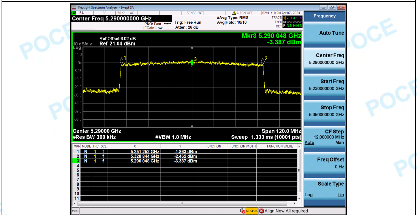
Frequency_Stability_NVNT_ANT2_802_11ax(HE80)_5290
