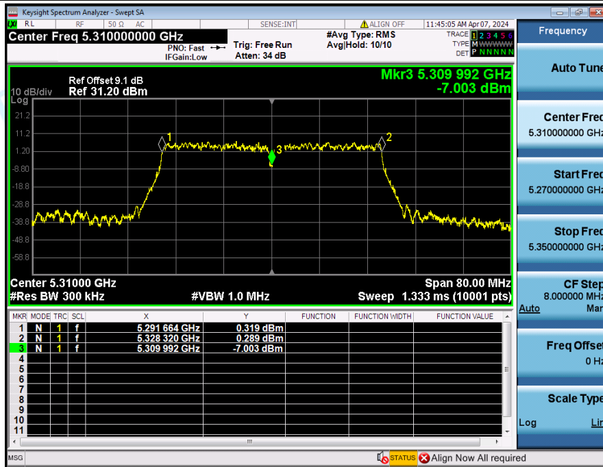
Frequency_Stability_NVNT_ANT3_802_11ac(VHT40)_5310
