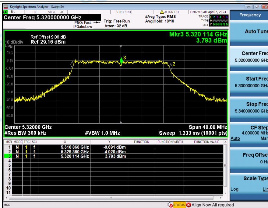
Frequency_Stability_NVNT_ANT3_802_11ac(VHT20)_5320
