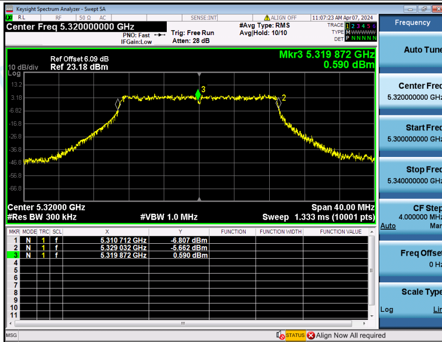
Frequency_Stability_NVNT_ANT2_802_11ac(VHT20)_5320
