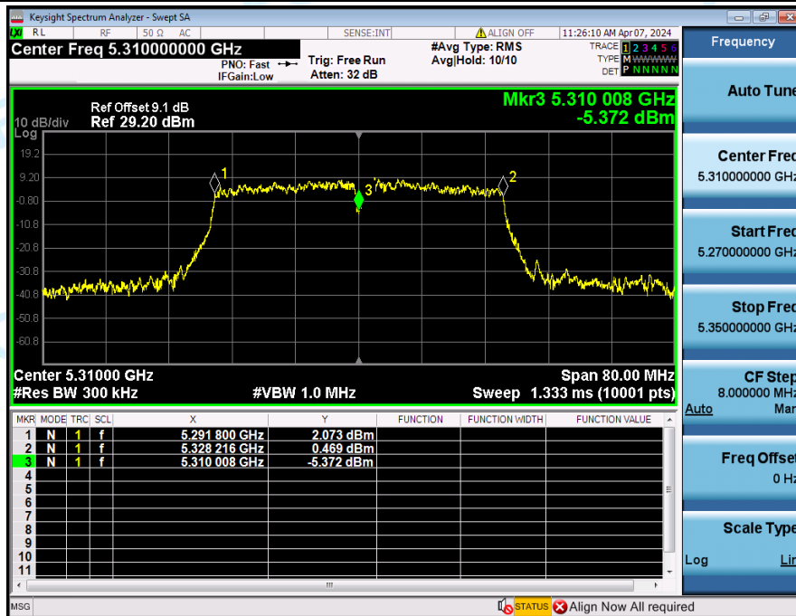
Frequency_Stability_NVNT_ANT3_802_11n(HT40)_5310
