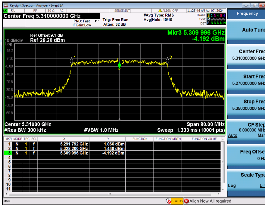
Frequency_Stability_NVNT_ANT3_802_11n(HT40)_5310
