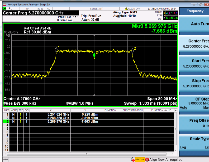
Frequency_Stability_NVNT_ANT3_802_11ac(VHT40)_5270
