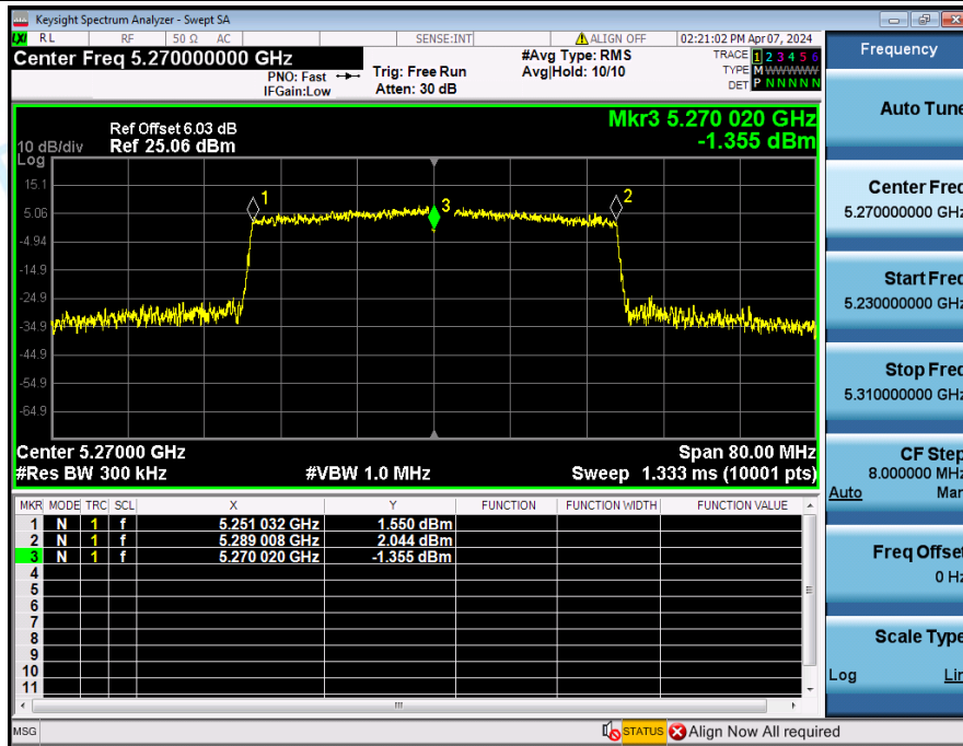
Frequency_Stability_NVNT_ANT2_802_11ax(HE40)_5270
