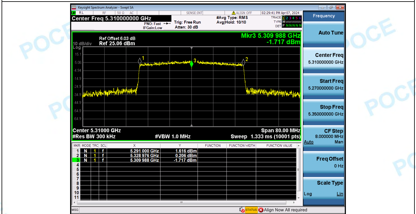
Frequency_Stability_NVNT_ANT2_802_11ax(HE40)_5310
