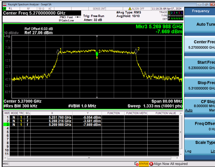
Frequency_Stability_NVNT_ANT2_802_11n(HT40)_5270
