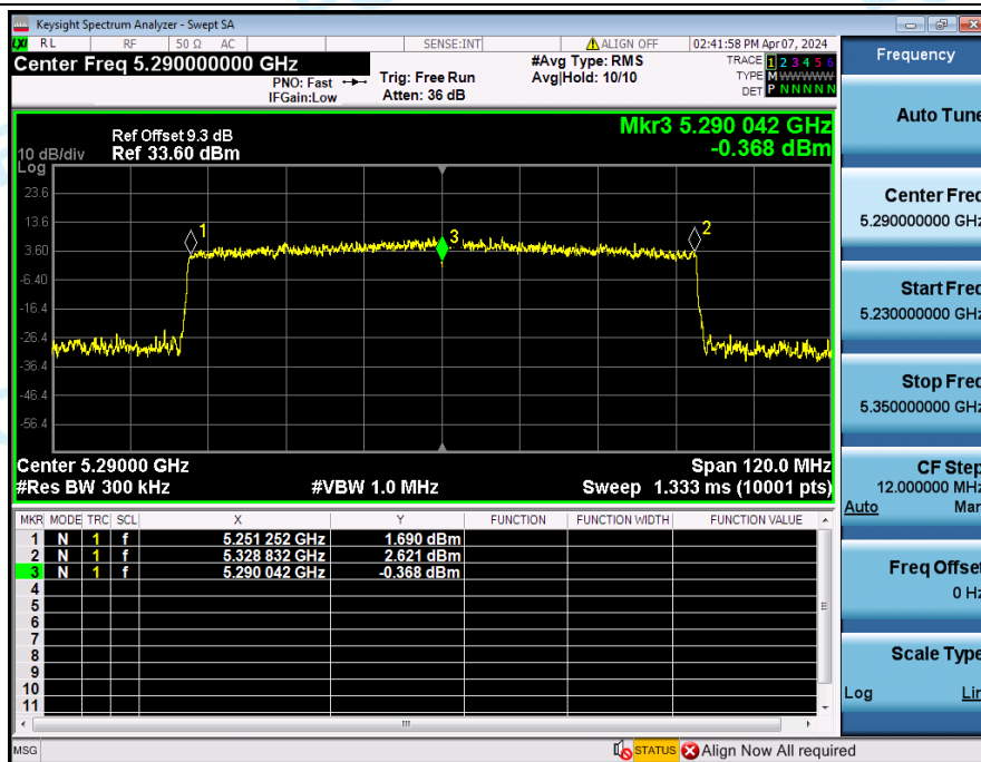
Frequency_Stability_NVNT_ANT3_802_11ax(HE80)_5290
