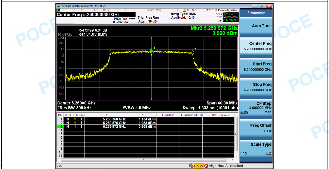
Frequency_Stability_NVNT_ANT2_802_11ax(HE20)_5260
