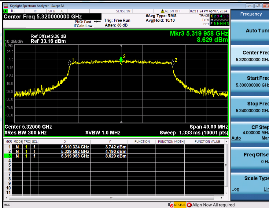
Frequency_Stability_NVNT_ANT3_802_11ax(HE20)_5320
