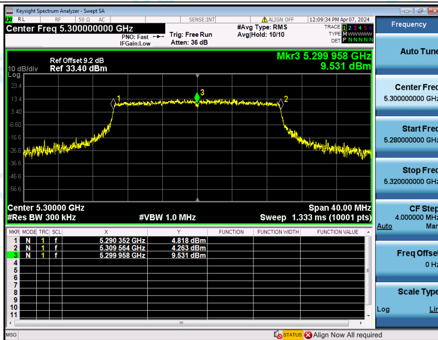
Frequency_Stability_NVNT_ANT3_802_11ax(HE20)_5300
