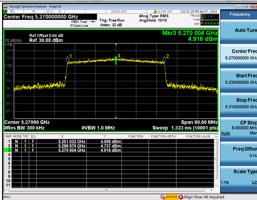
Frequency_Stability_NVNT_ANT3_802_11ax(HE40)_5270
