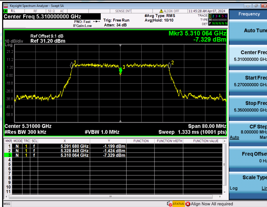
Frequency_Stability_NVNT_ANT3_802_11ac(VHT40)_5310
