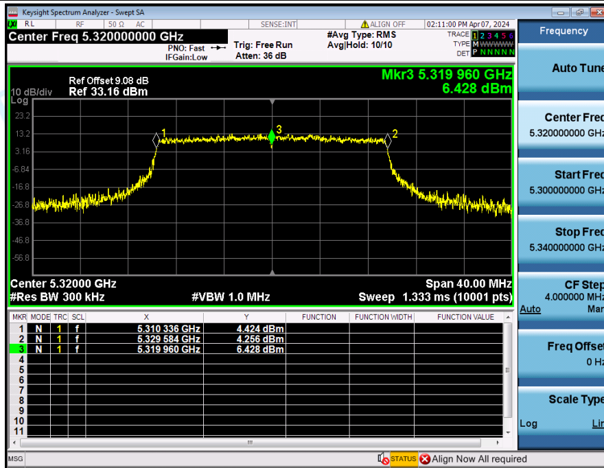
Frequency_Stability_NVNT_ANT3_802_11ax(HE20)_5320
