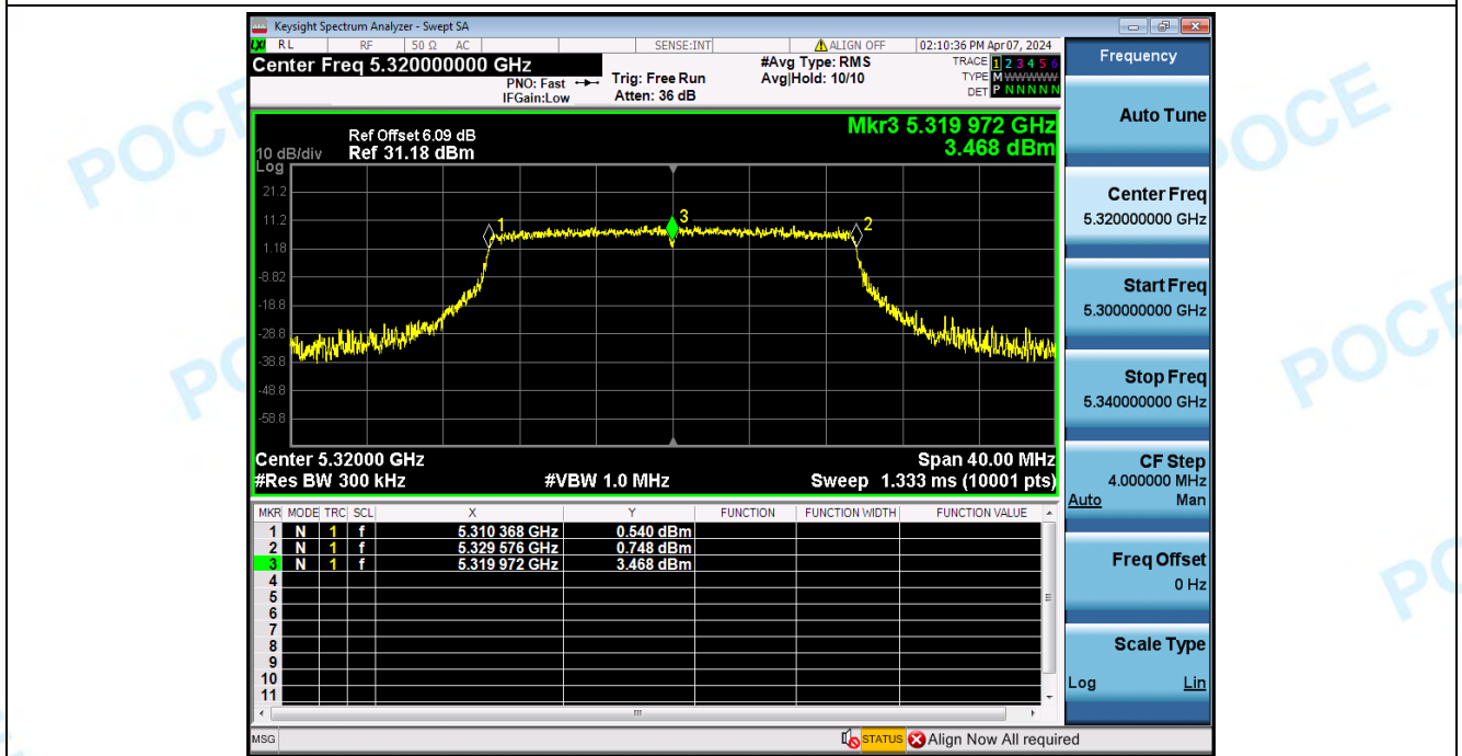
Frequency_Stability_NVNT_ANT2_802_11ax(HE20)_5320
