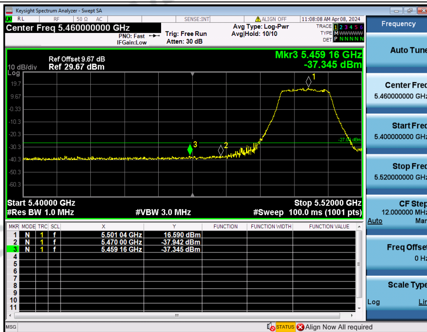
Bandedge_NVNT_ANT3_802_11n(HT20)_5500
