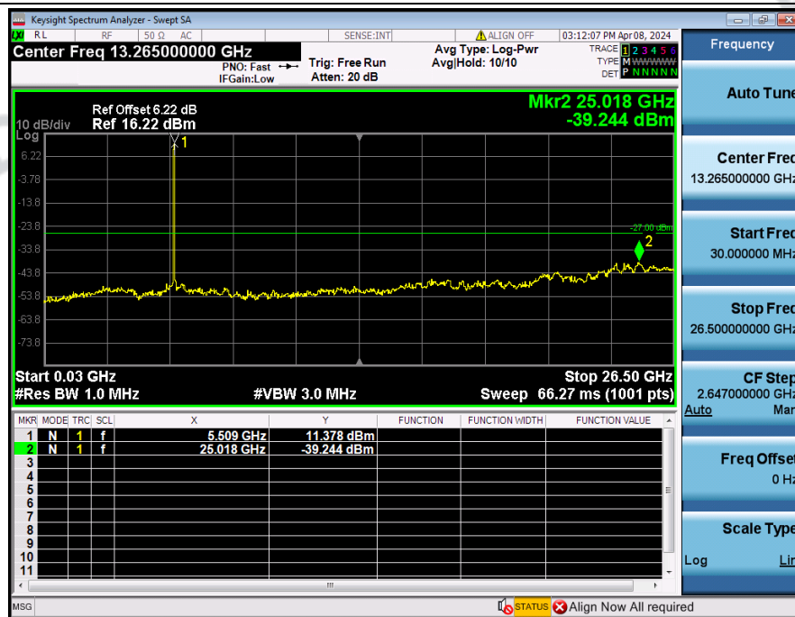
Spurious_Emission_NVNT_ANT2_802_11a_5500
