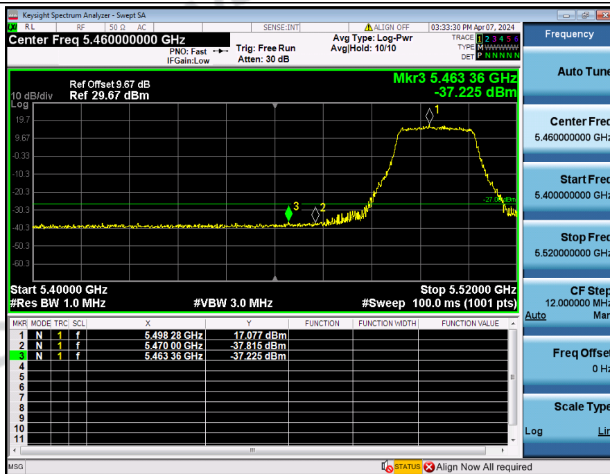
Bandedge_NVNT_ANT3_802_11ax(HE20)_5500
