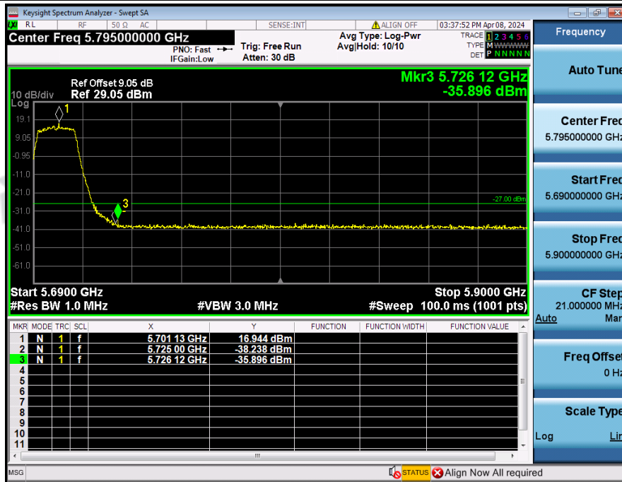
Bandedge_NVNT_ANT3_802_11a_5700
