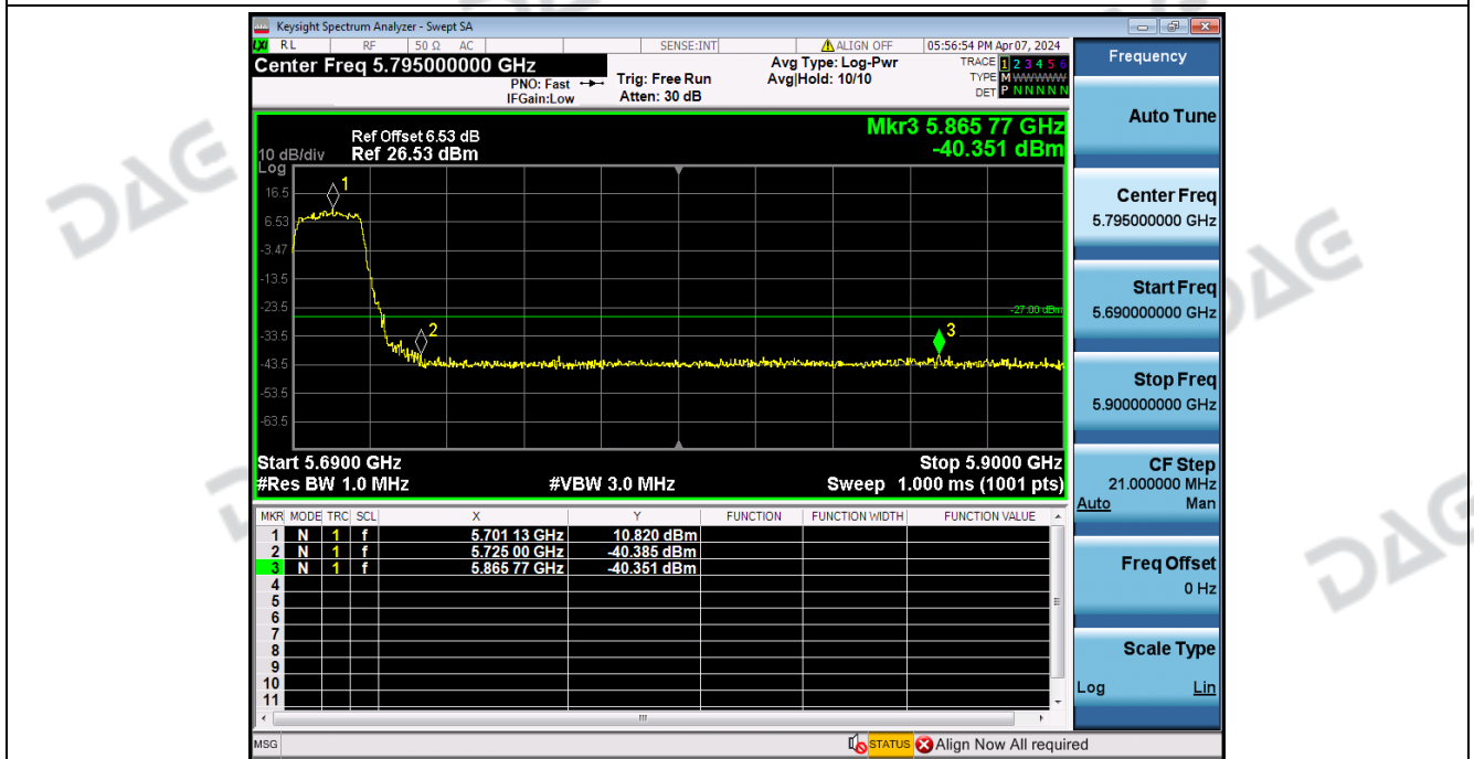
Bandedge_NVNT_ANT2_802_11ac(VHT20)_5700
