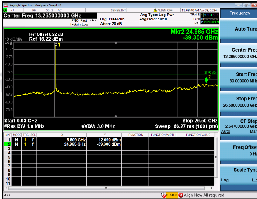
Spurious_Emission_NVNT_ANT2_802_11n(HT20)_5500
