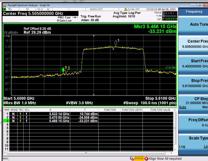
Bandedge_NVNT_ANT3_802_11ac(VHT80)_5530
