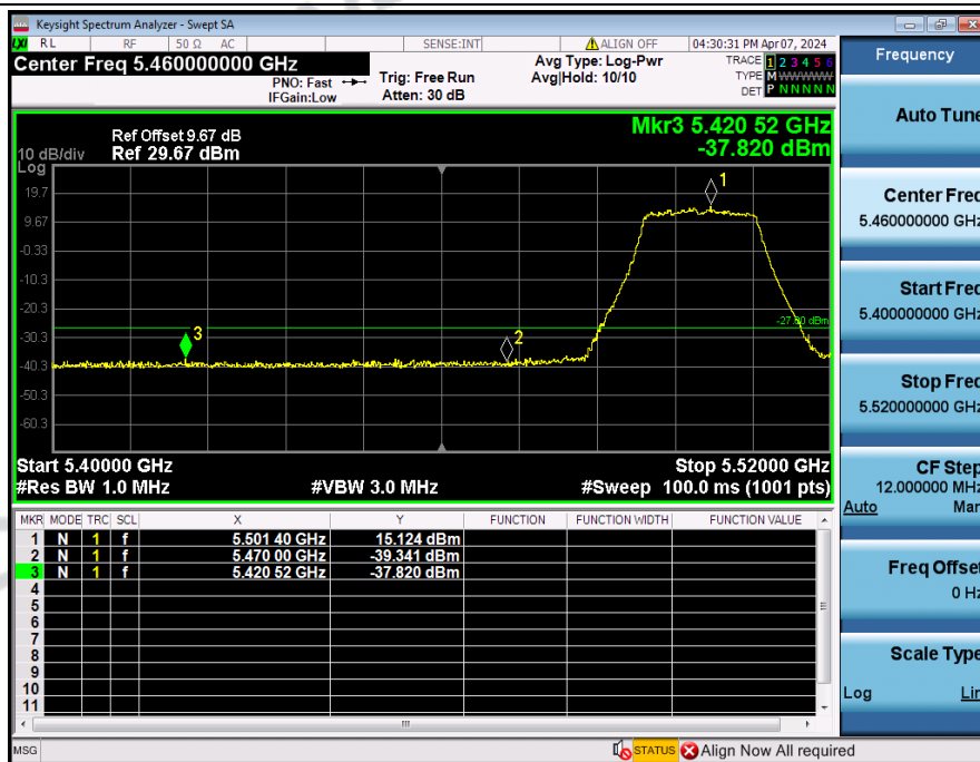
Bandedge_NVNT_ANT3_802_11ac(VHT20)_5500
