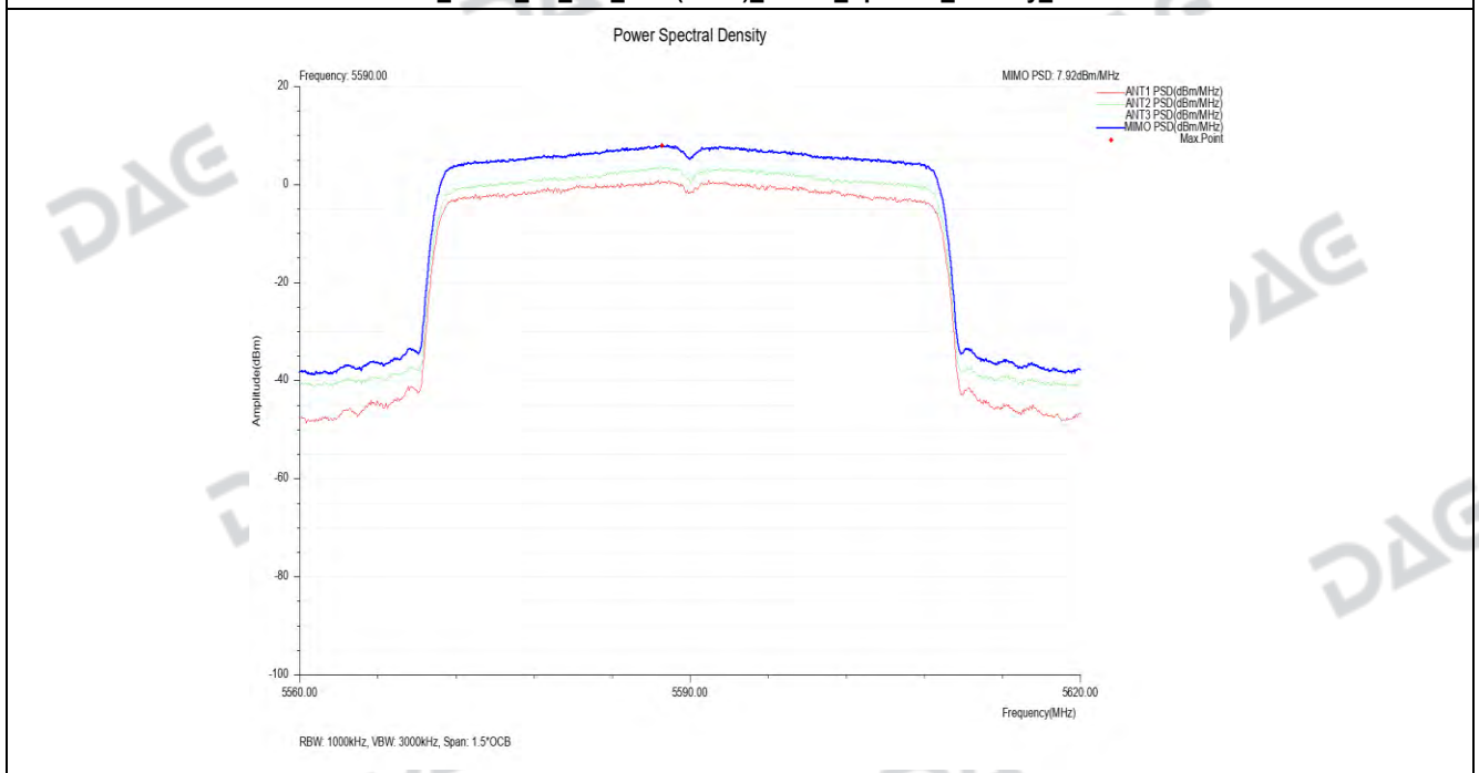
NVNT_MIMO_TX_802_11ax(HE40)_Power_Spectral_Density_5590
