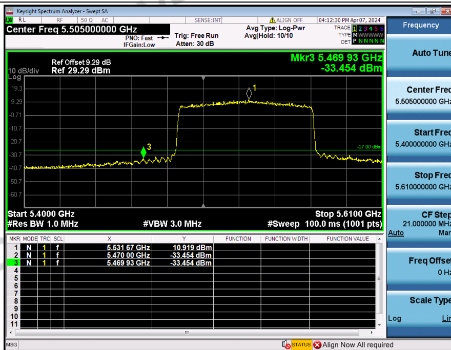
Bandedge_NVNT_ANT3_802_11ax(HE80)_5530
