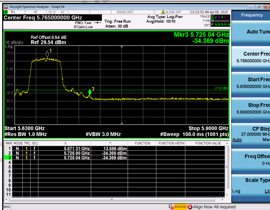
Bandedge_NVNT_ANT3_802_11ac(VHT40)_5670
