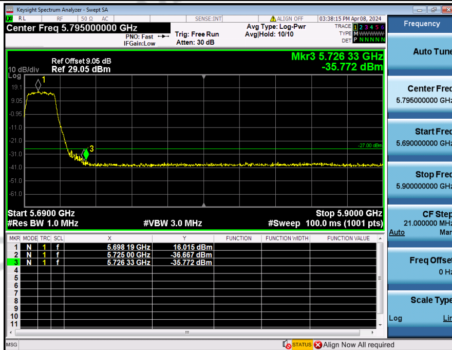
Bandedge_NVNT_ANT3_802_11a_5700
