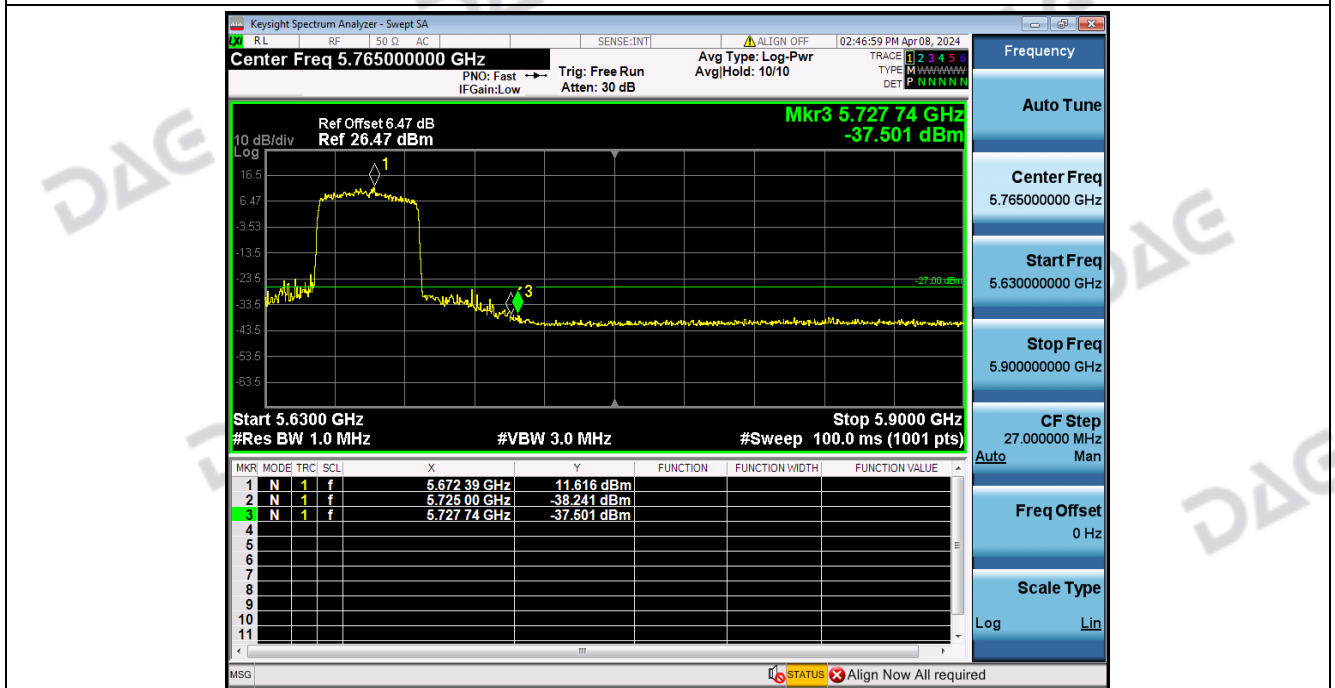
Bandedge_NVNT_ANT2_802_11ax(HE40)_5670
