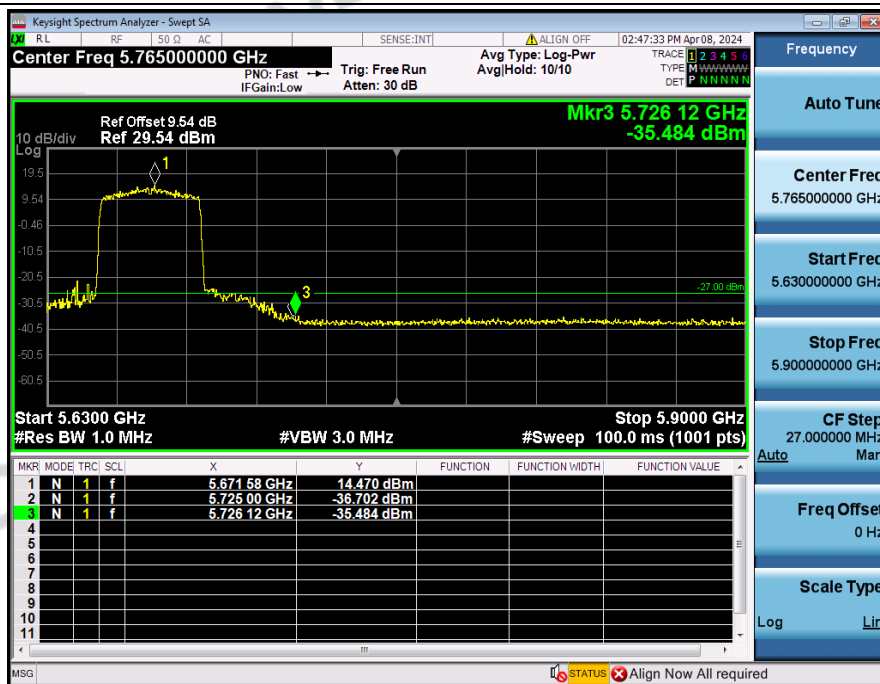
Bandedge_NVNT_ANT3_802_11ac(HE40)_5670
