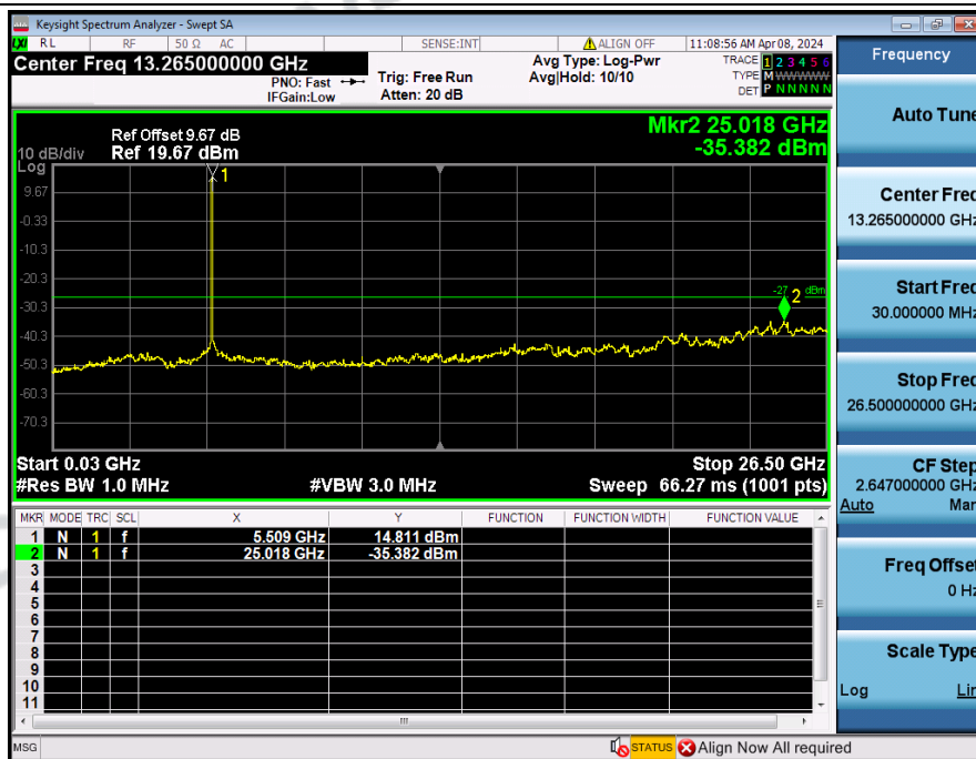
Spurious_Emission_NVNT_ANT3_802_11n(HT20)_5500
