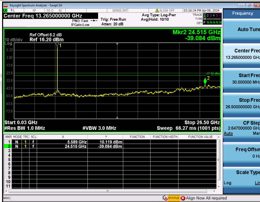
Spurious_Emission_NVNT_ANT2_802_11a_5600
