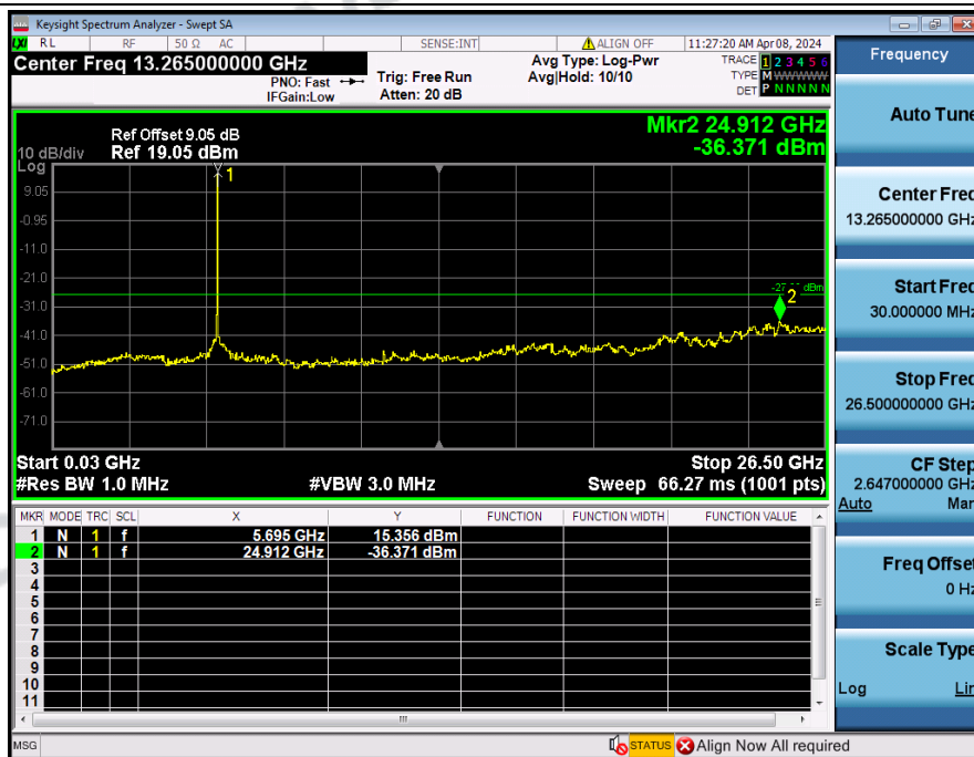
Spurious_Emission_NVNT_ANT3_802_11n(HT20)_5700
