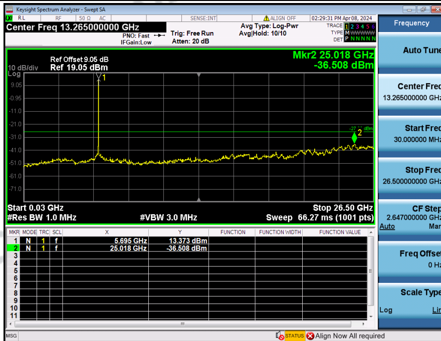
Spurious_Emission_NVNT_ANT3_802_11ax(HE20)_5700
