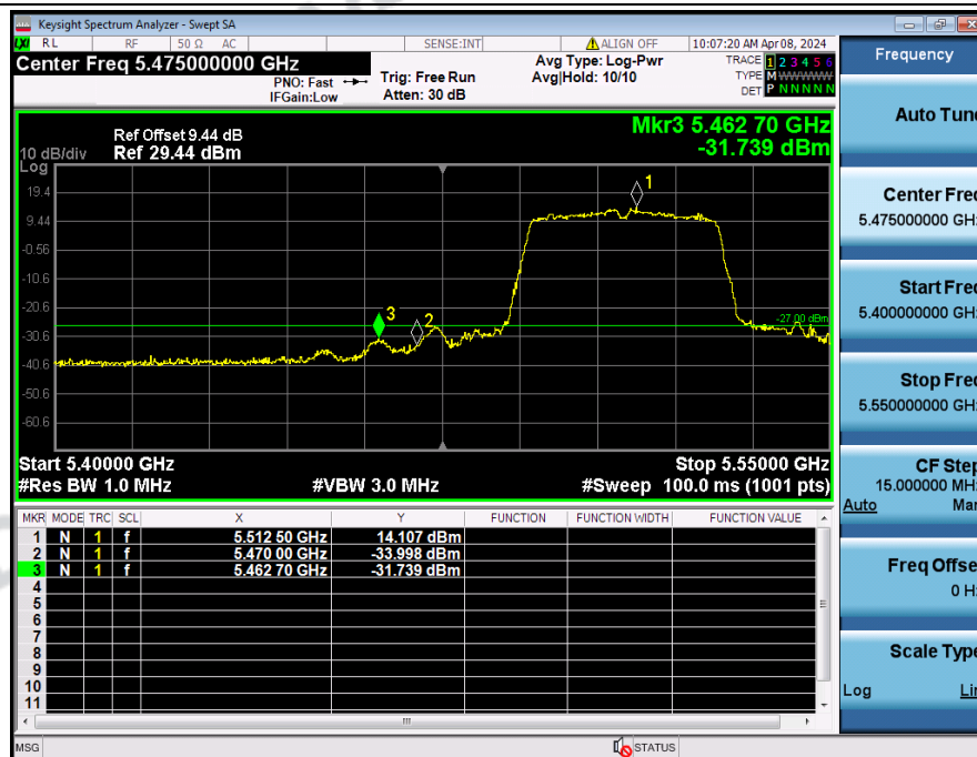
Bandedge_NVNT_ANT3_802_11ac(VHT40)_5510
