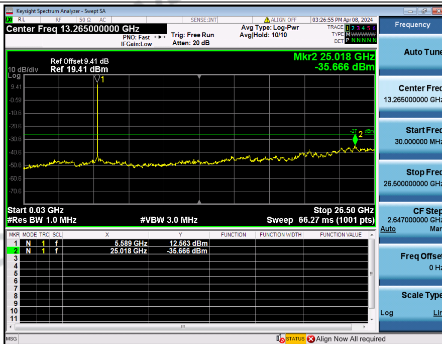
Spurious_Emission_NVNT_ANT3_802_11a_5600
