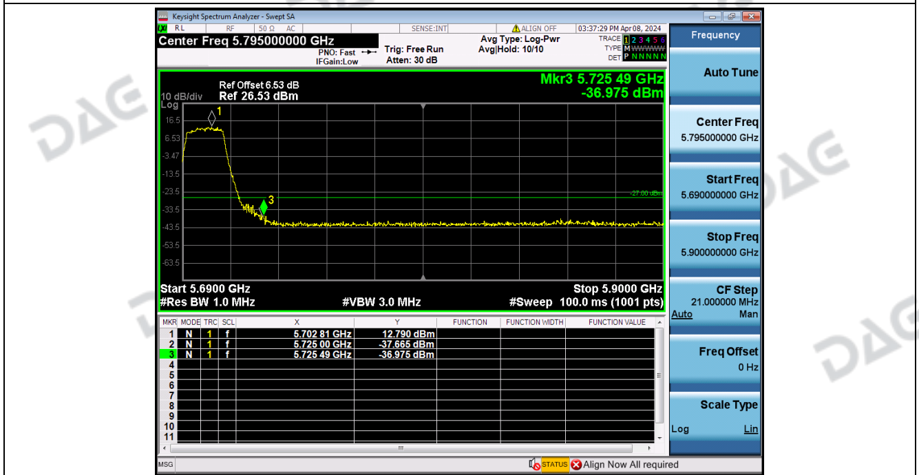
Bandedge_NVNT_ANT2_802_11a_5700
