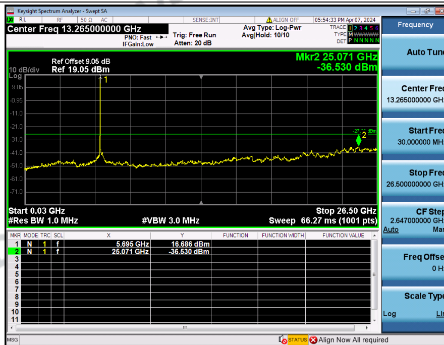
Spurious_Emission_NVNT_ANT3_802_11ac(VHT20)_5700
