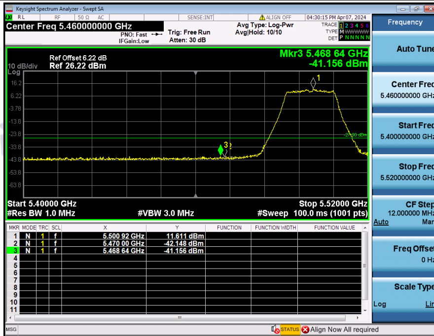
Bandedge_NVNT_ANT2_802_11ac(VHT20)_5500
