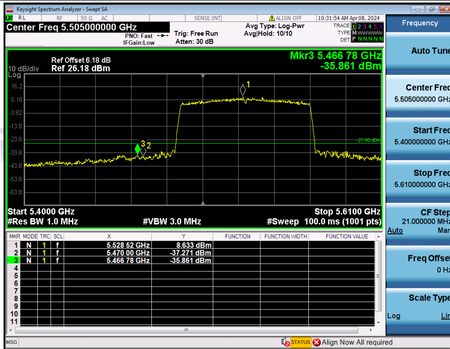
Bandedge_NVNT_ANT2_802_11ac(VHT80)_5530
