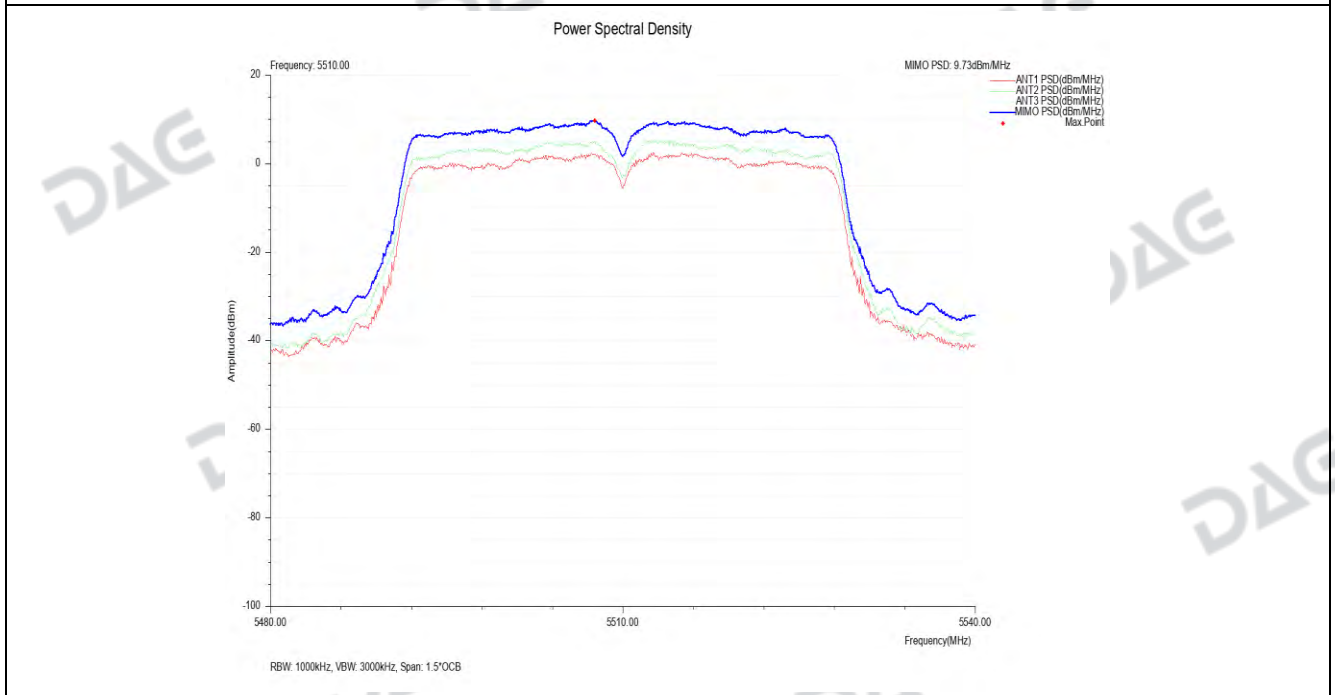
NVNT_MIMO_TX_802_11ac(VHT40)_Power_Spectral_Density_5510
