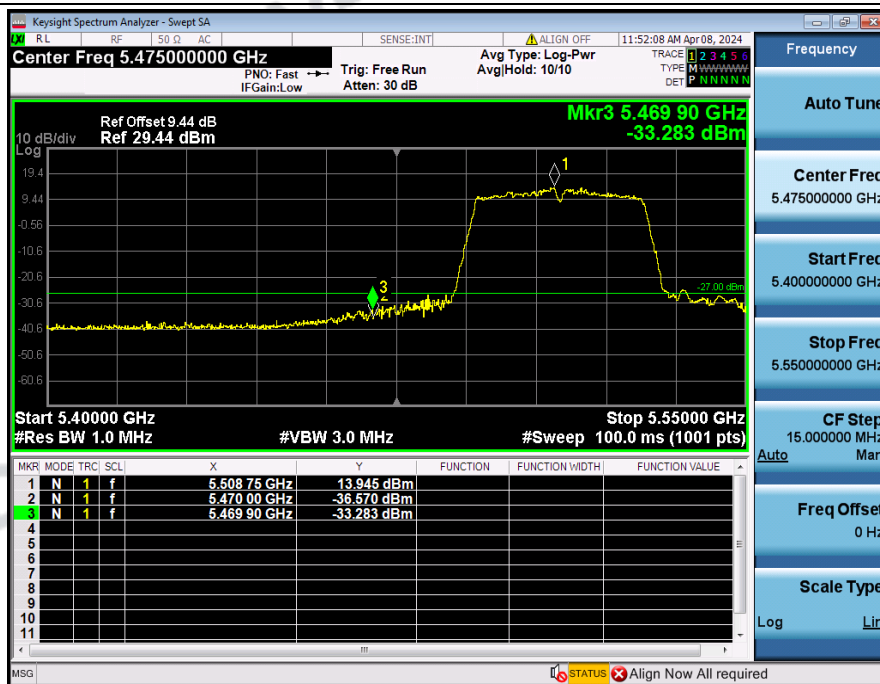
Bandedge_NVNT_ANT3_802_11n(HT40)_5510
