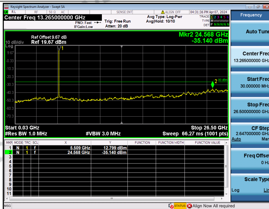
Spurious_Emission_NVNT_ANT3_802_11ac(VHT20)_5500
