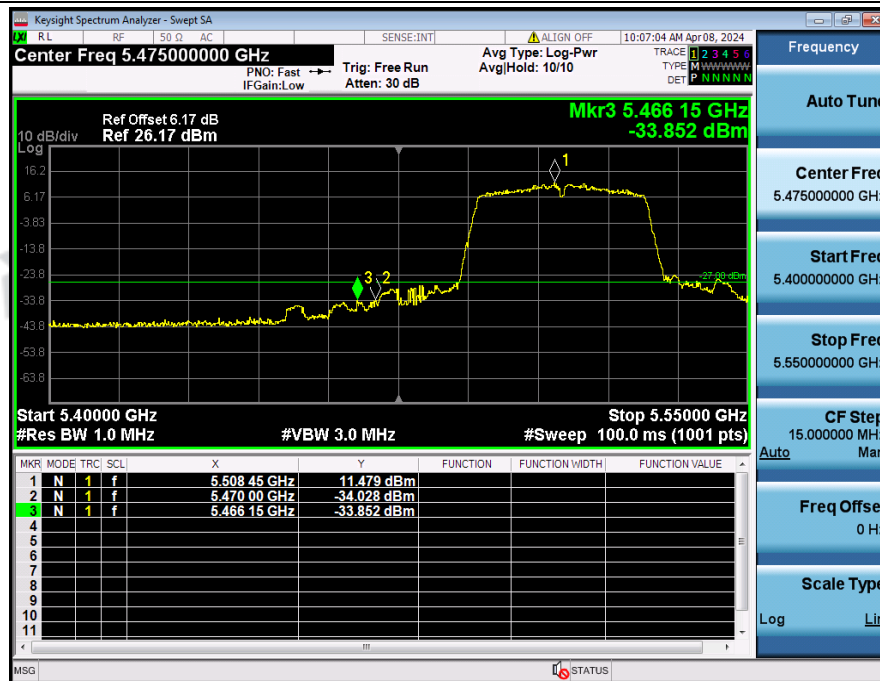
Bandedge_NVNT_ANT2_802_11ac(VHT40)_5510
