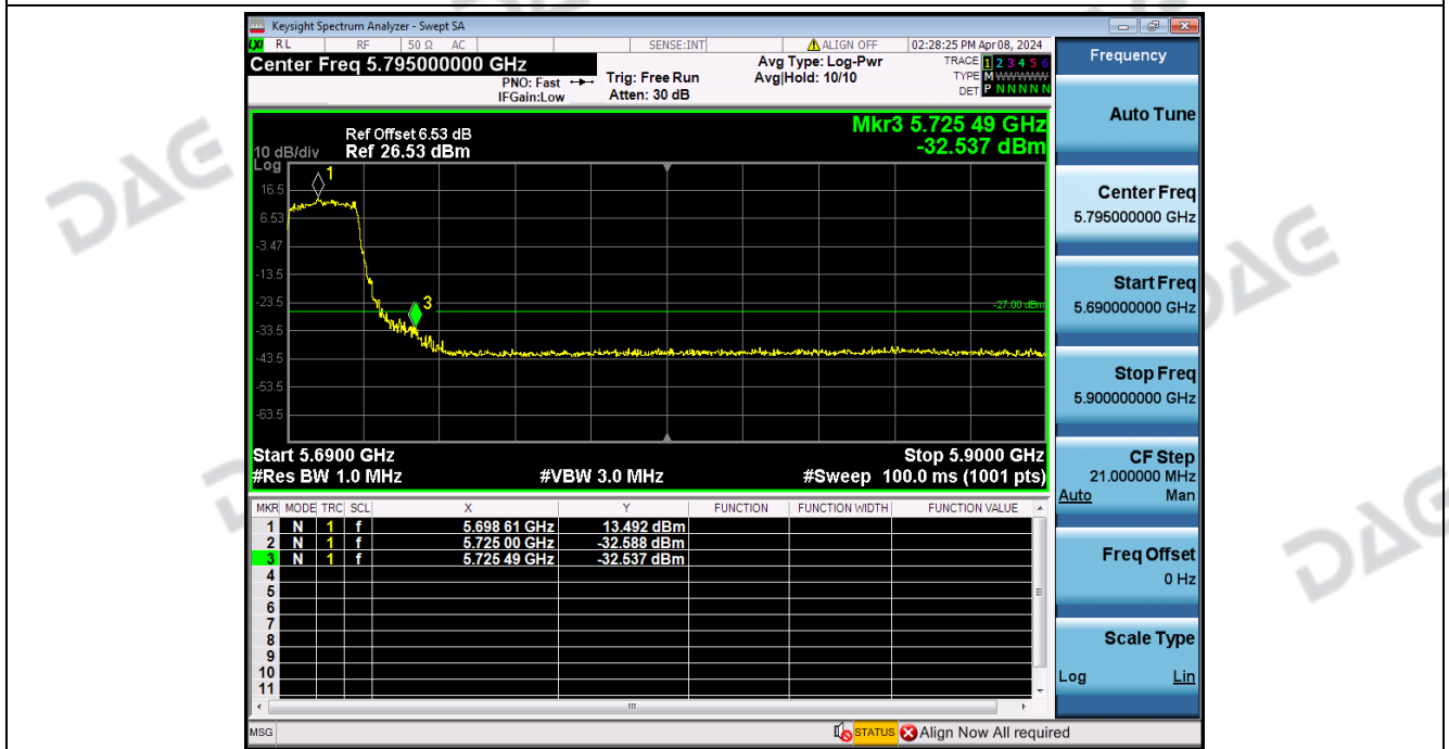
Bandedge_NVNT_ANT2_802_11ax(HE20)_5700
