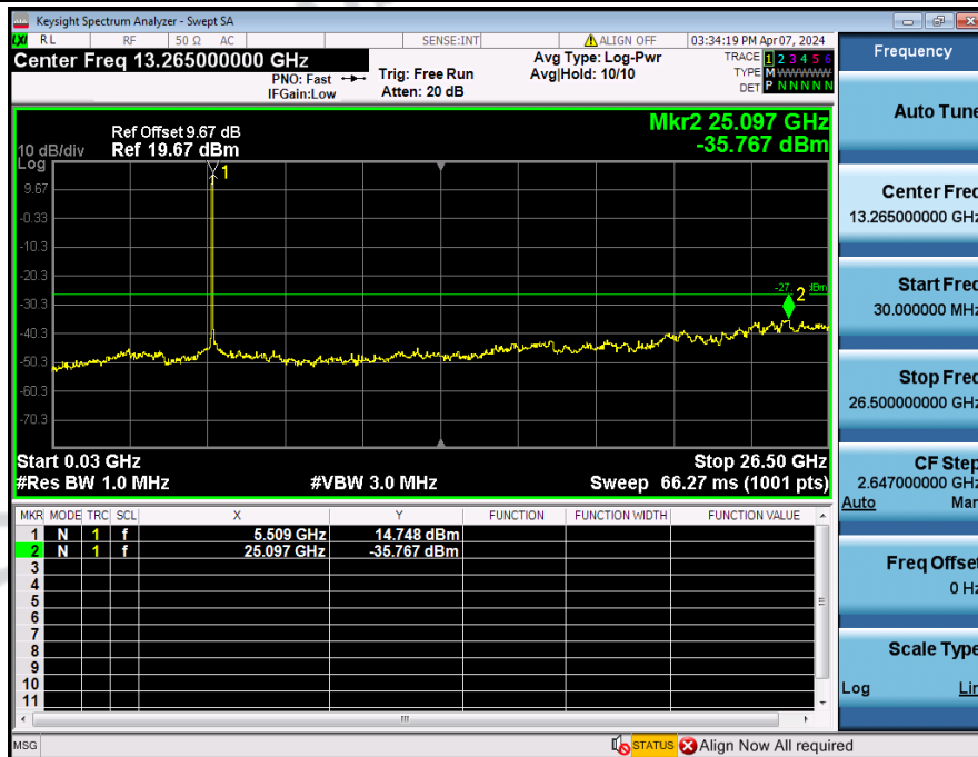
Spurious_Emission_NVNT_ANT3_802_11ax(HE20)_5500
