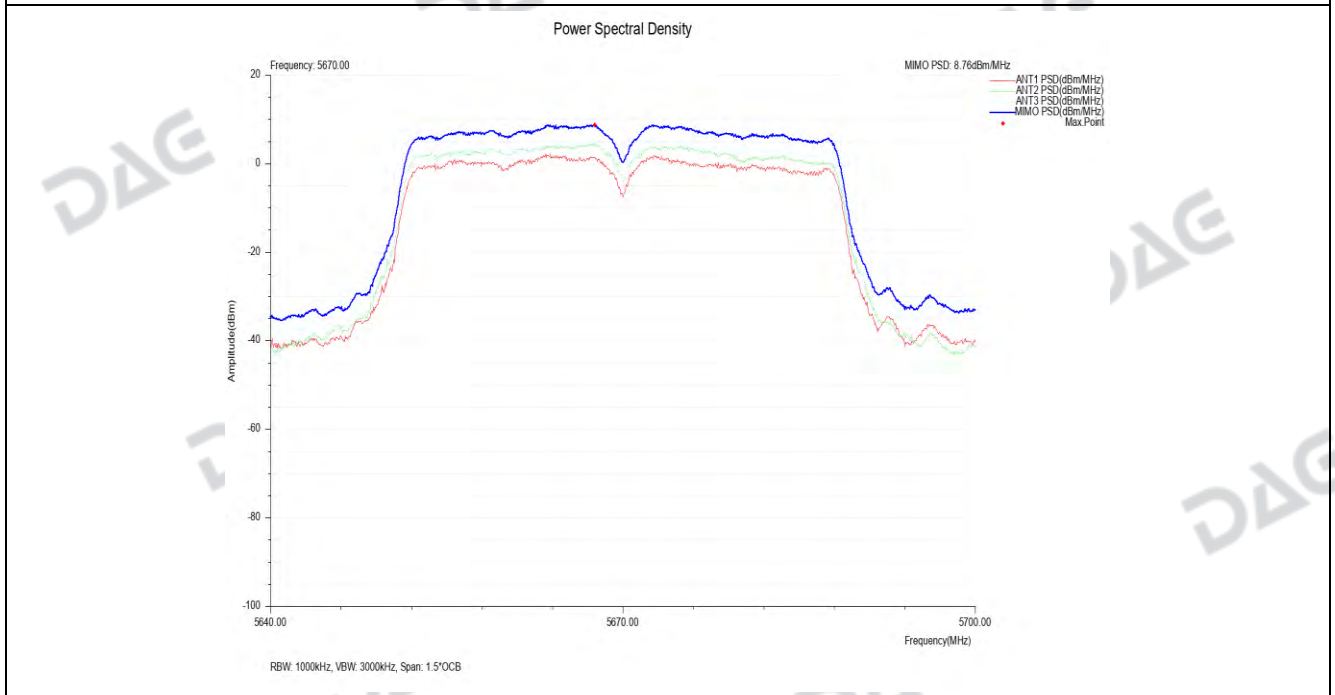
NVNT_MIMO_TX_802_11ac(VHT40)_Power_Spectral_Density_5670
