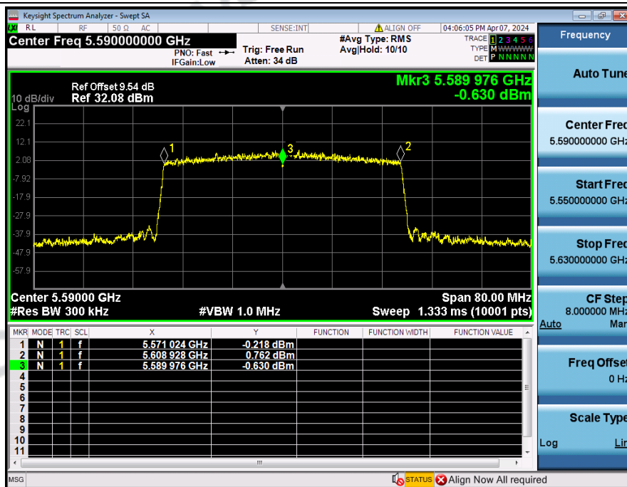
Frequency_Stability_NVNT_ANT3_802_11ax(HE40)_5590
