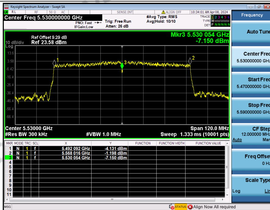
Frequency_Stability_NVNT_ANT3_802_11ac(VHT80)_5530
