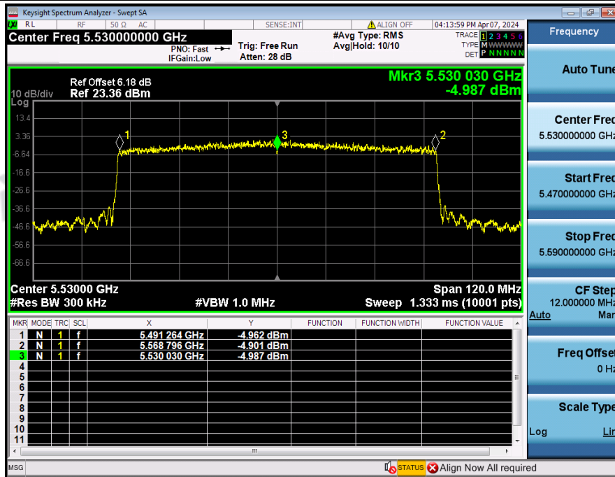
Frequency_Stability_NVNT_ANT2_802_11ax(HE80)_5530
