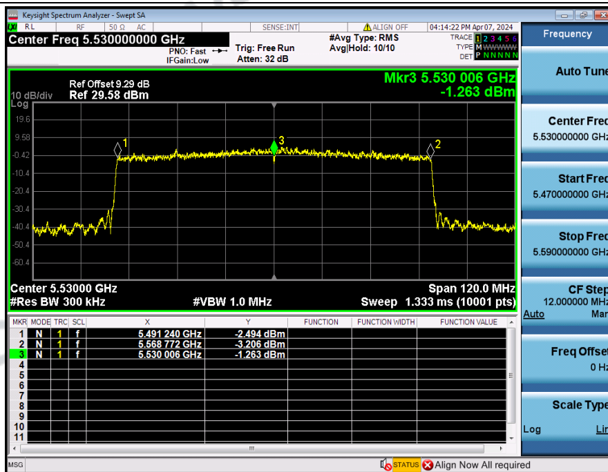
Frequency_Stability_NVNT_ANT3_802_11ax(HE80)_5530
