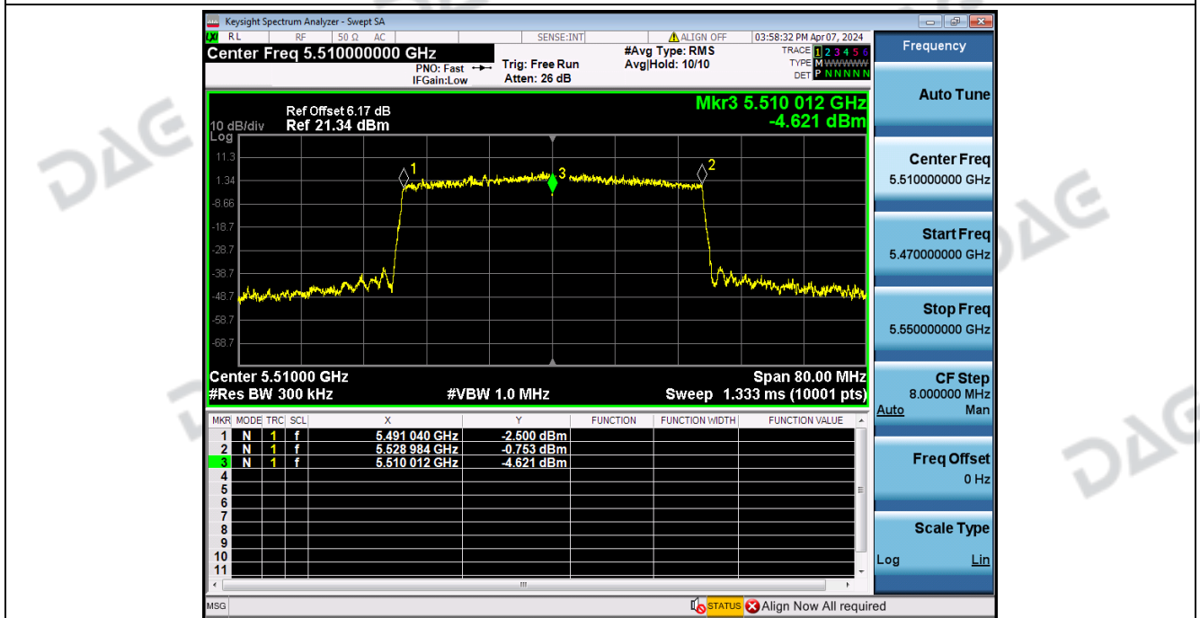
Frequency_Stability_NVNT_ANT2_802_11ax(HE40)_5510
