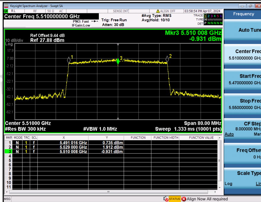
Frequency_Stability_NVNT_ANT3_802_11ax(HE40)_5510
