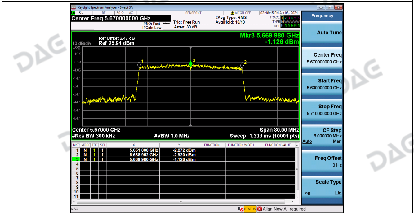
Frequency_Stability_NVNT_ANT2_802_11ax(HE40)_5670
