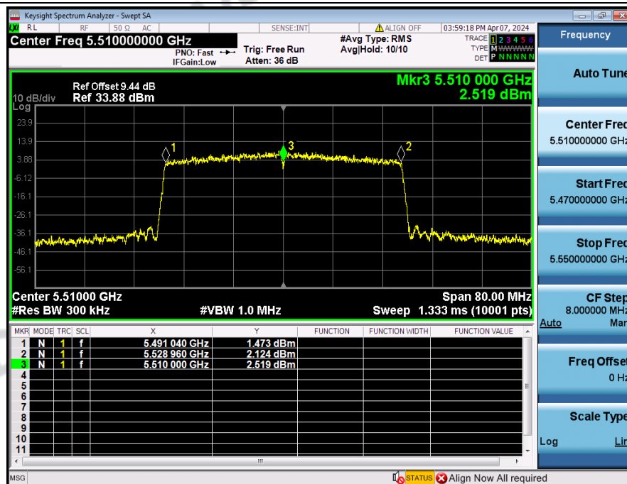
Frequency_Stability_NVNT_ANT3_802_11ax(HE40)_5510
