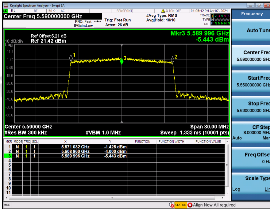
Frequency_Stability_NVNT_ANT2_802_11ax(HE40)_5590
