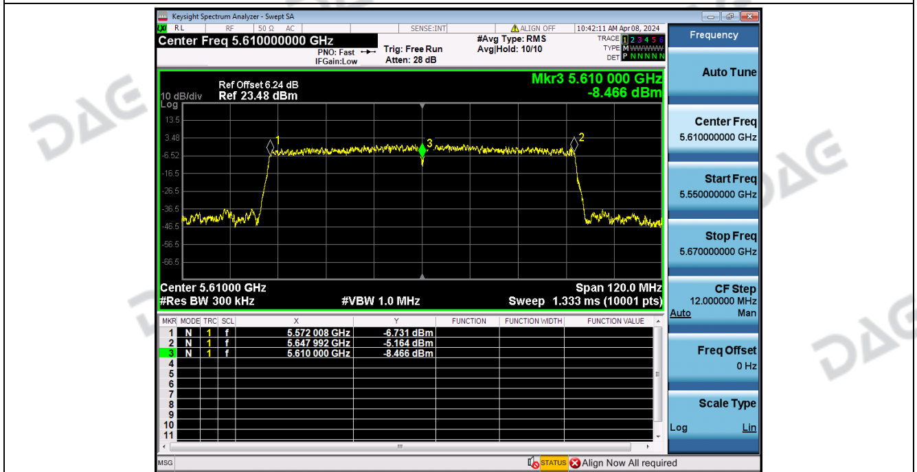
Frequency_Stability_NVNT_ANT2_802_11ac(VHT80)_5610
