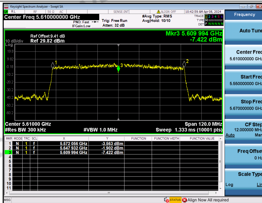
Frequency_Stability_NVNT_ANT3_802_11ac(VHT80)_5610
