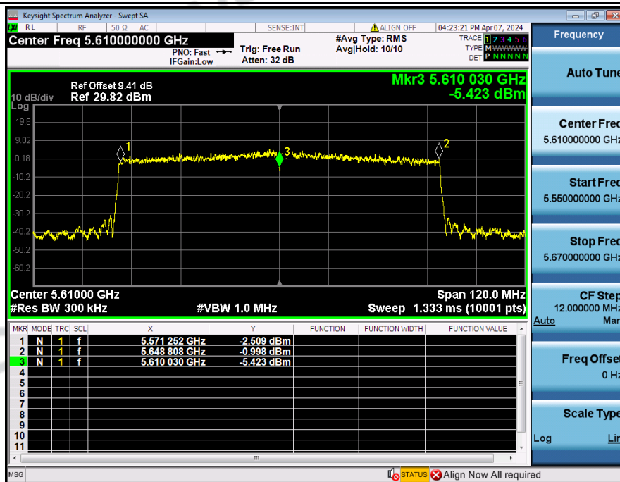
Frequency_Stability_NVNT_ANT3_802_11ax(HE80)_5610
