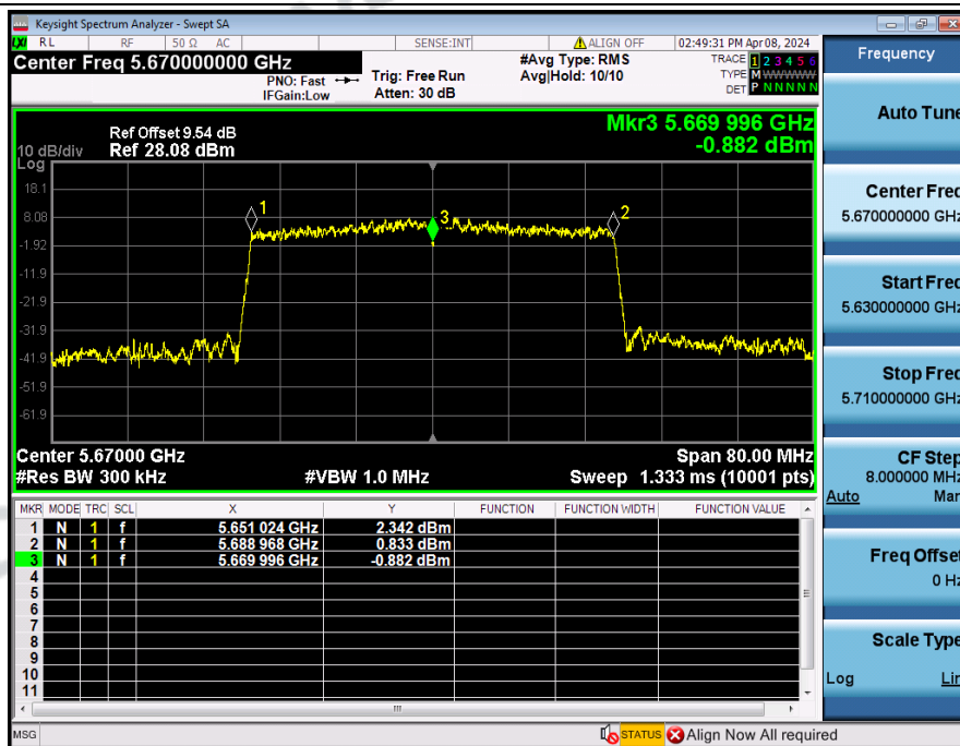
Frequency_Stability_NVNT_ANT3_802_11ax(HE40)_5670
