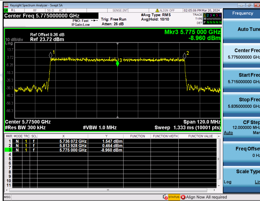
Frequency_Stability_NVNT_ANT3_802_11ax(HE80)_5775
