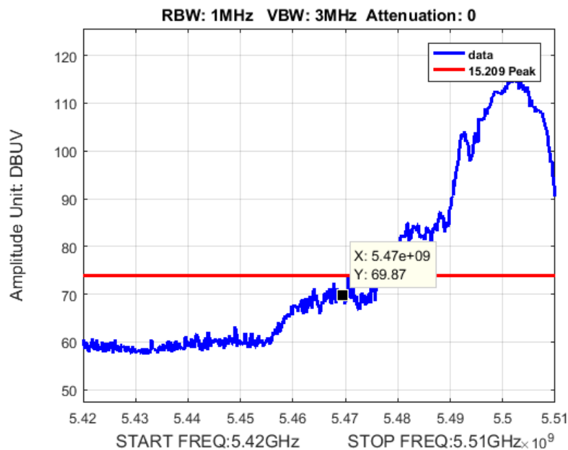
Figure 28: Band Edge BW 20M Ch 5500M 80211a Peak
