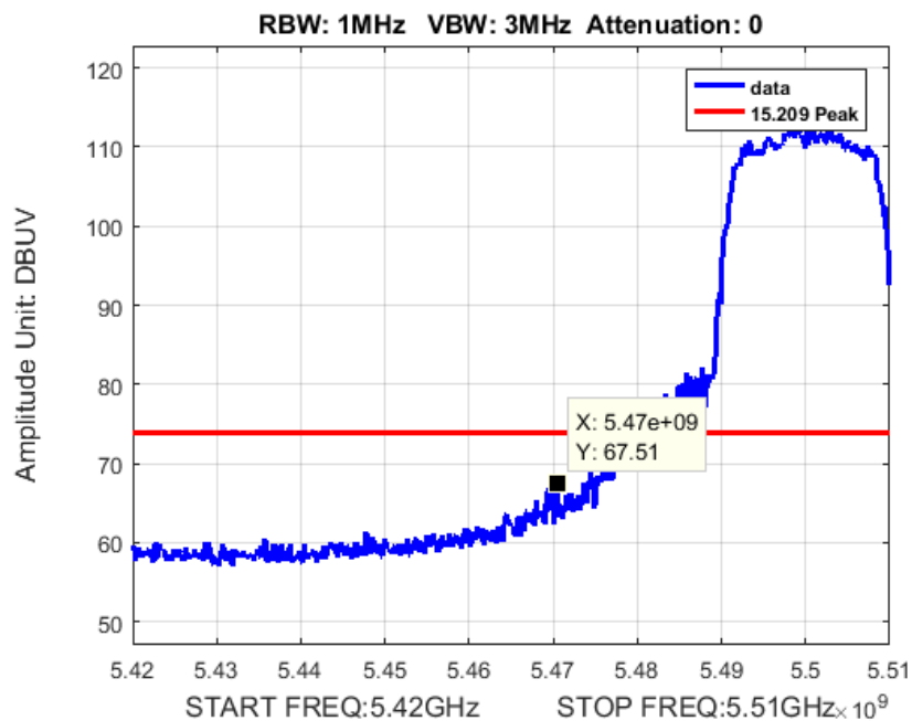
Figure 30: Band Edge BW 20M Ch 5500M 80211n Peak
