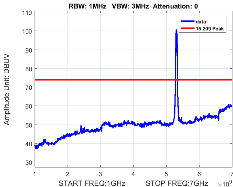
Figure 6: Radiated Spurious Emission 1-7GHz BW 40M Ch 5310M 80211n Peak
