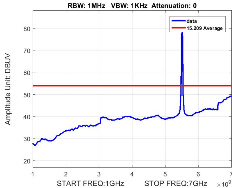
Figure 13: Radiated Spurious Emission 1-7GHz BW 40M Ch 5510M 80211n Average
