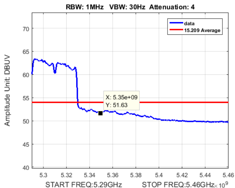
Figure 25: Band Edge BW 80M Ch 5290M 80211ac Average
