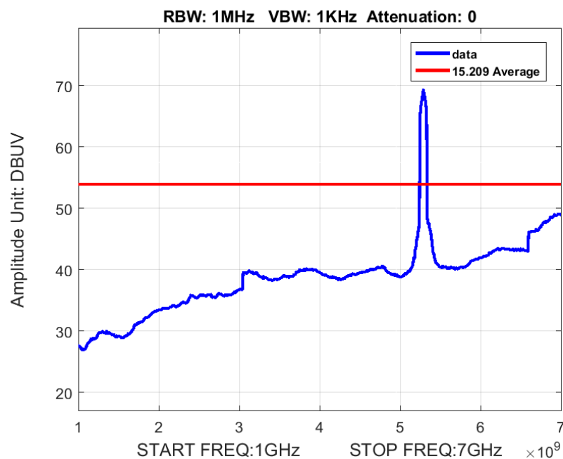
Figure 7: Radiated Spurious Emission 1-7GHz BW 80M Ch 5290M 80211ac Average
