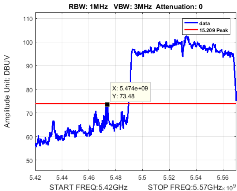
Figure 34: Band Edge BW 80M Ch 5530M 80211ac Peak
