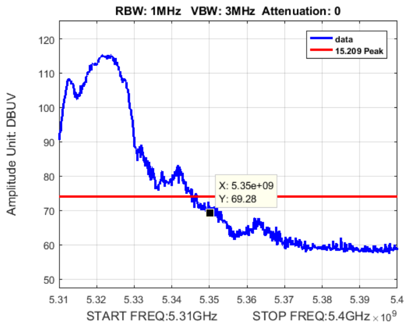
Figure 20: Band Edge BW 20M Ch 5320M 80211a Peak
