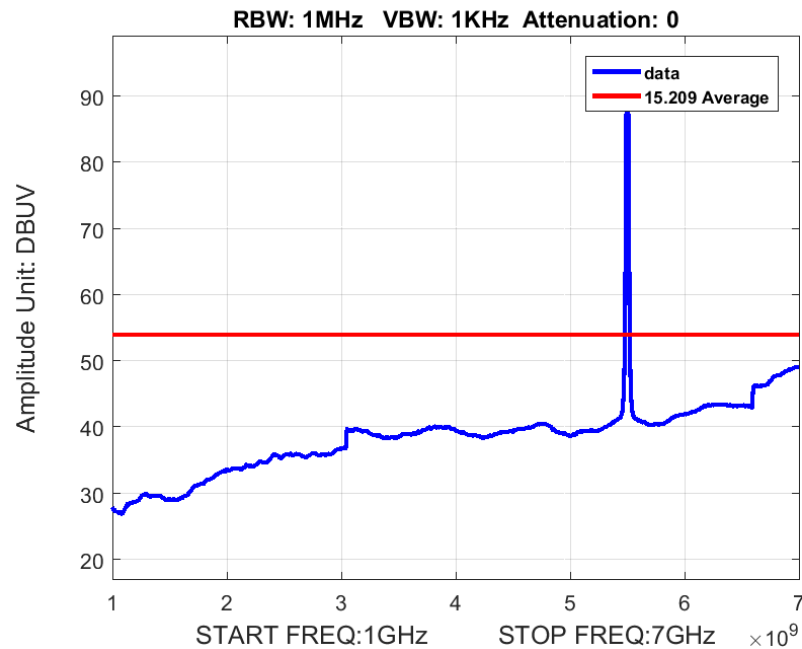
Figure 11: Radiated Spurious Emission 1-7GHz BW 20M Ch 5500M 80211n Average
