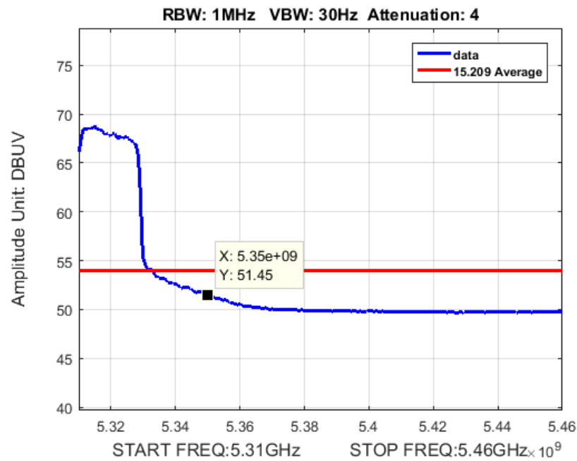
Figure 23: Band Edge BW 40M Ch 5310M 80211n Average
