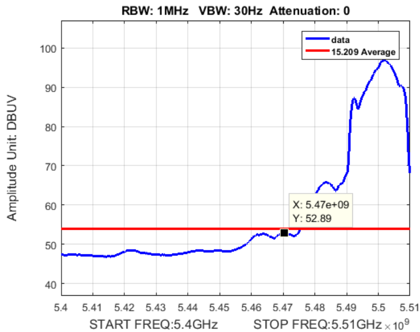
Figure 27: Band Edge BW 20M Ch 5500M 80211a Average
