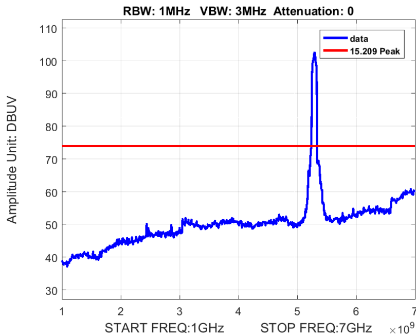
Figure 8: Radiated Spurious Emission 1-7GHz BW 80M Ch 5290M 80211ac Peak
