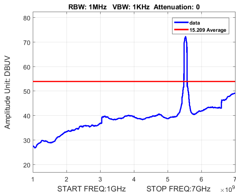
Figure 15: Radiated Spurious Emission 1-7GHz BW 80M Ch 5530M 80211ac Average
