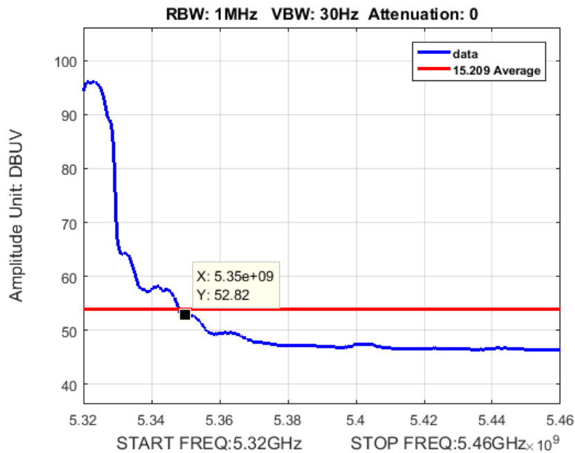
Figure 19: Band Edge BW 20M Ch 5320M 80211a Average
