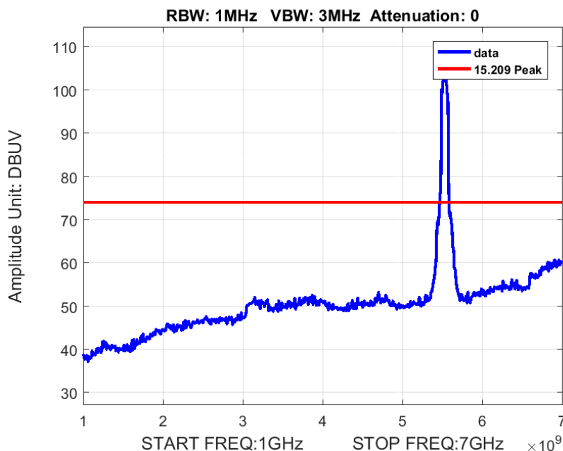
Figure 16: Radiated Spurious Emission 1-7GHz BW 80M Ch 5530M 80211ac Peak
