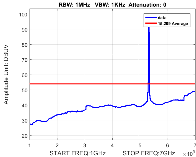
Figure 3: Radiated Spurious Emission 1-7GHz BW 20M Ch 5320M 80211n Average
