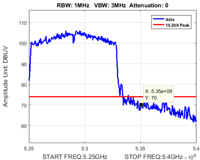
Figure 26: Band Edge BW 80M Ch 5290M 80211ac Peak
