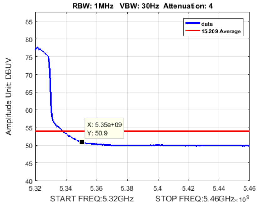
Figure 21: Band Edge BW 20M Ch 5320M 80211n Average
