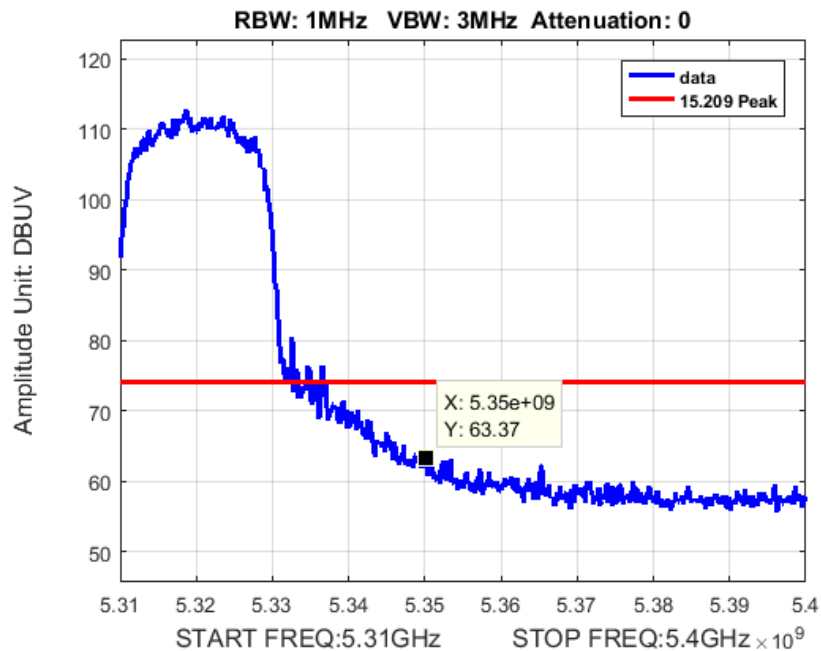
Figure 22: Band Edge BW 20M Ch 5320M 80211n Peak
