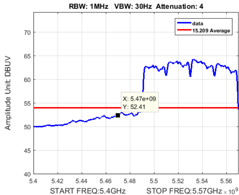
Figure 33: Band Edge BW 80M Ch 5530M 80211ac Average
