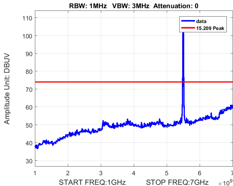
Figure 12: Radiated Spurious Emission 1-7GHz BW 20M Ch 5500M 80211n Peak
