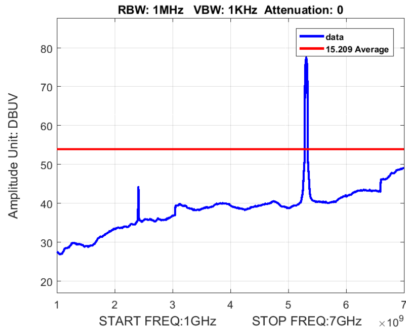
Figure 5: Radiated Spurious Emission 1-7GHz BW 40M Ch 5310M 80211n Average
