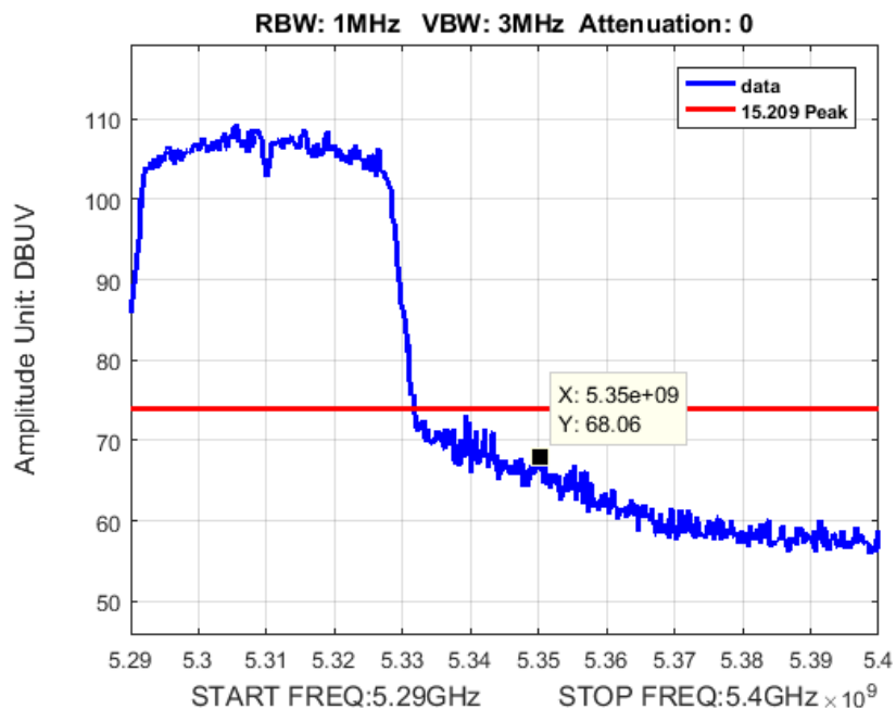
Figure 24: Band Edge BW 40M Ch 5310M 80211n Peak
