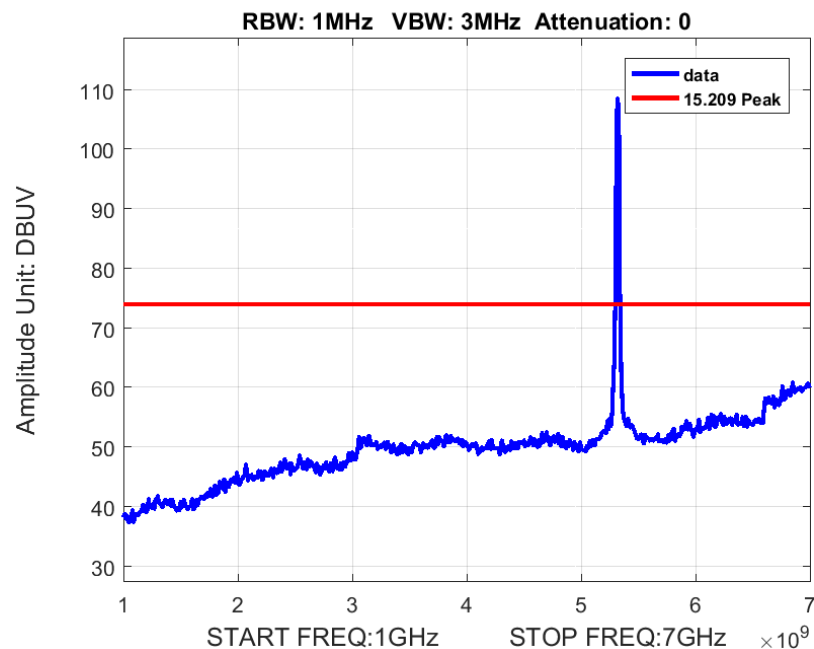
Figure 4: Radiated Spurious Emission 1-7GHz BW 20M Ch 5320M 80211n Peak
