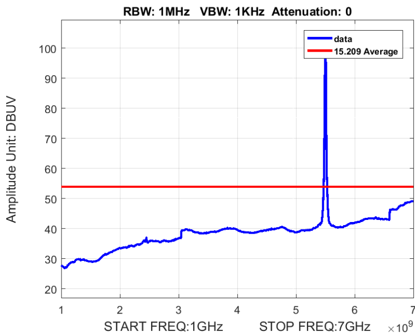
Figure 9: Radiated Spurious Emission 1-7GHz BW 20M Ch 5500M 80211a Average
