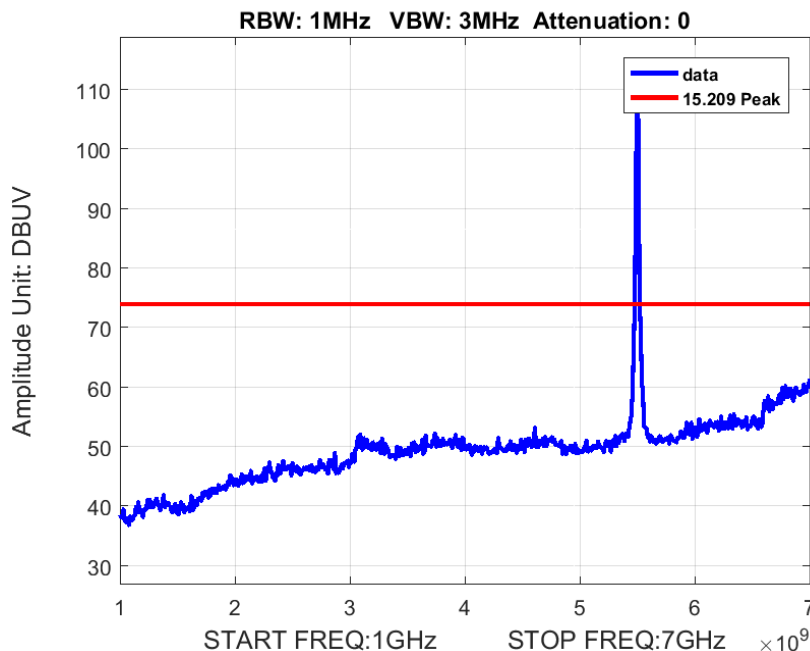
Figure 10: Radiated Spurious Emission 1-7GHz BW 20M Ch 5500M 80211a Peak
