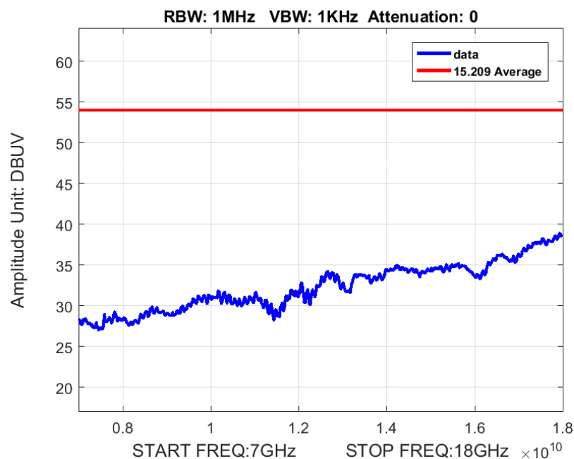
Figure 17: Radiated Spurious Emission 7-18GHz Worst Case Average
