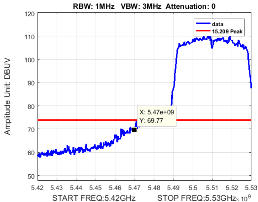
Figure 32: Band Edge BW 40M Ch 5510M 80211n Peak
