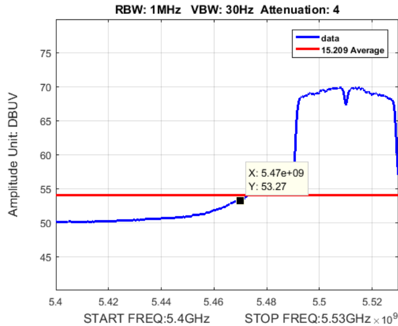
Figure 31: Band Edge BW 40M Ch 5510M 80211n Average
