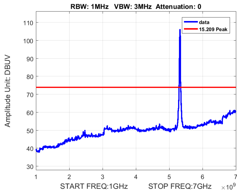
Figure 2: Radiated Spurious Emission 1-7GHz BW 20M Ch 5320M 80211a Peak
