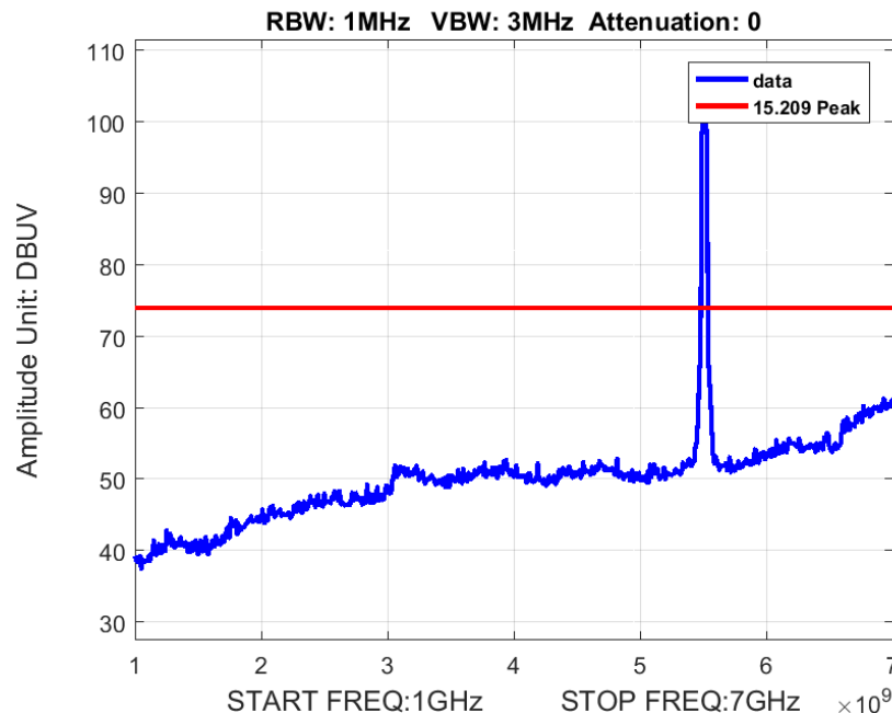
Figure 14: Radiated Spurious Emission 1-7GHz BW 40M Ch 5510M 80211n Peak
