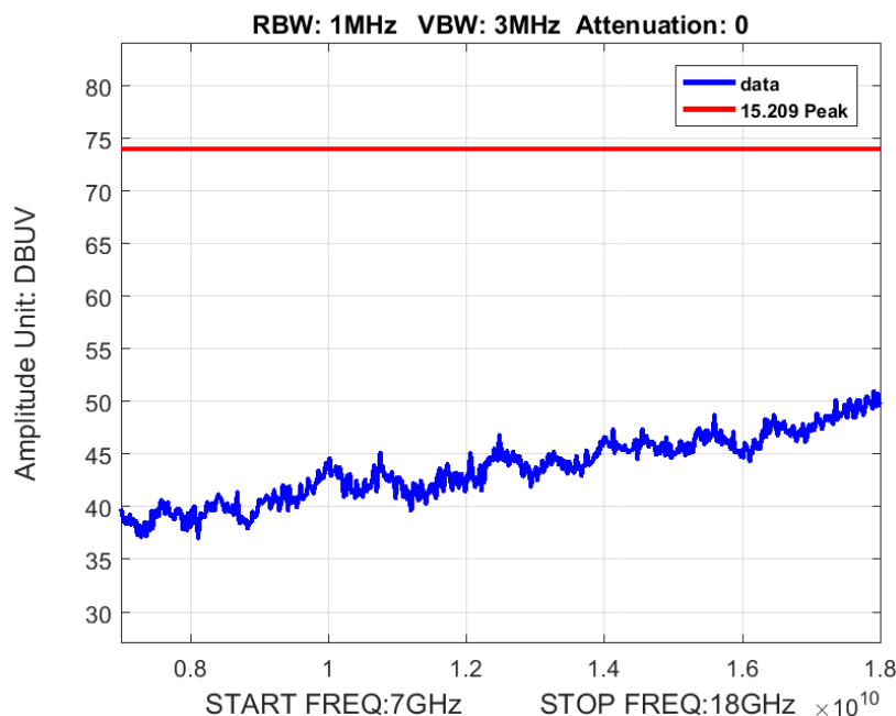
Figure 18: Radiated Spurious Emission 7-18GHz Worst Case Peak
