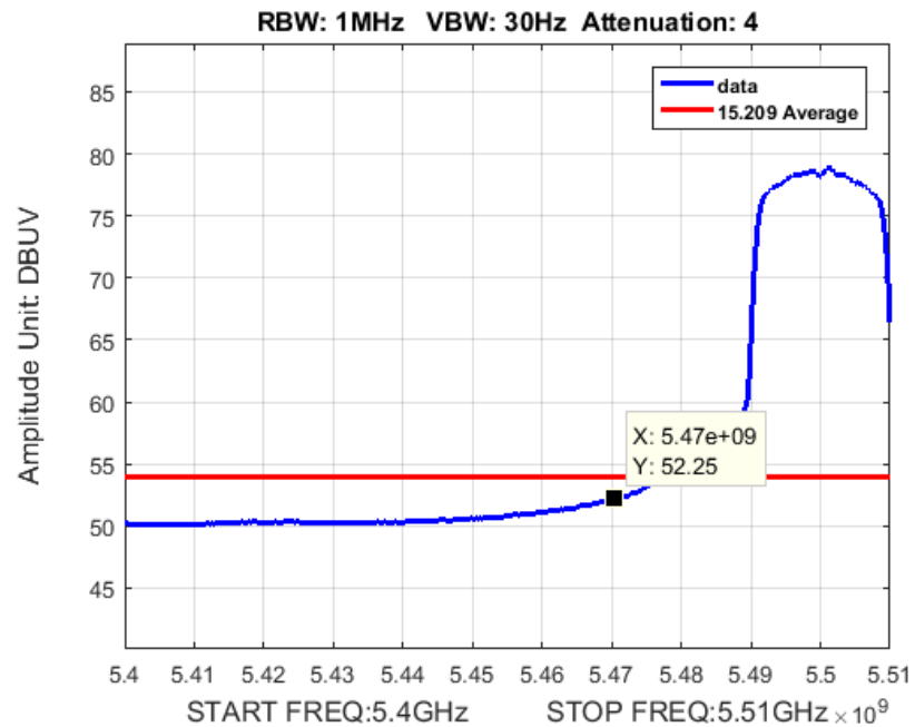
Figure 29: Band Edge BW 20M Ch 5500M 80211n Average
