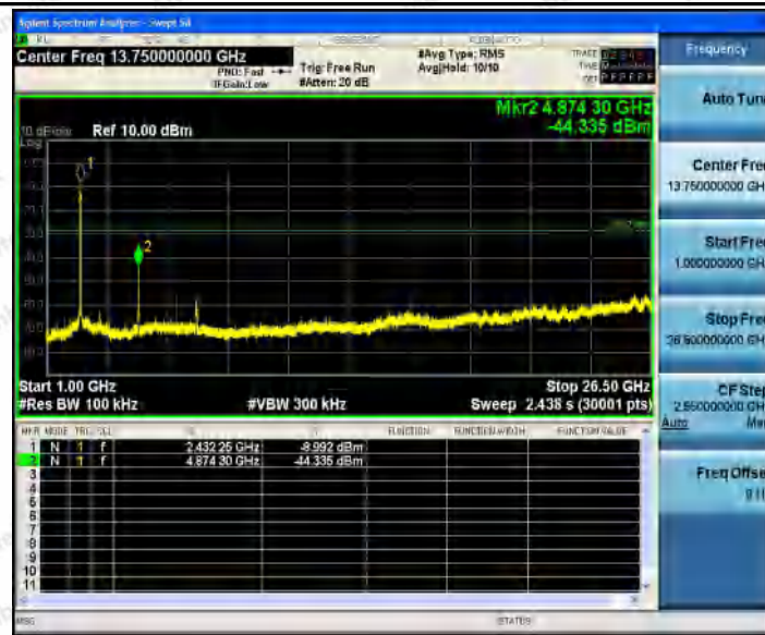
11N40_Ant2_2437_0~Reference
