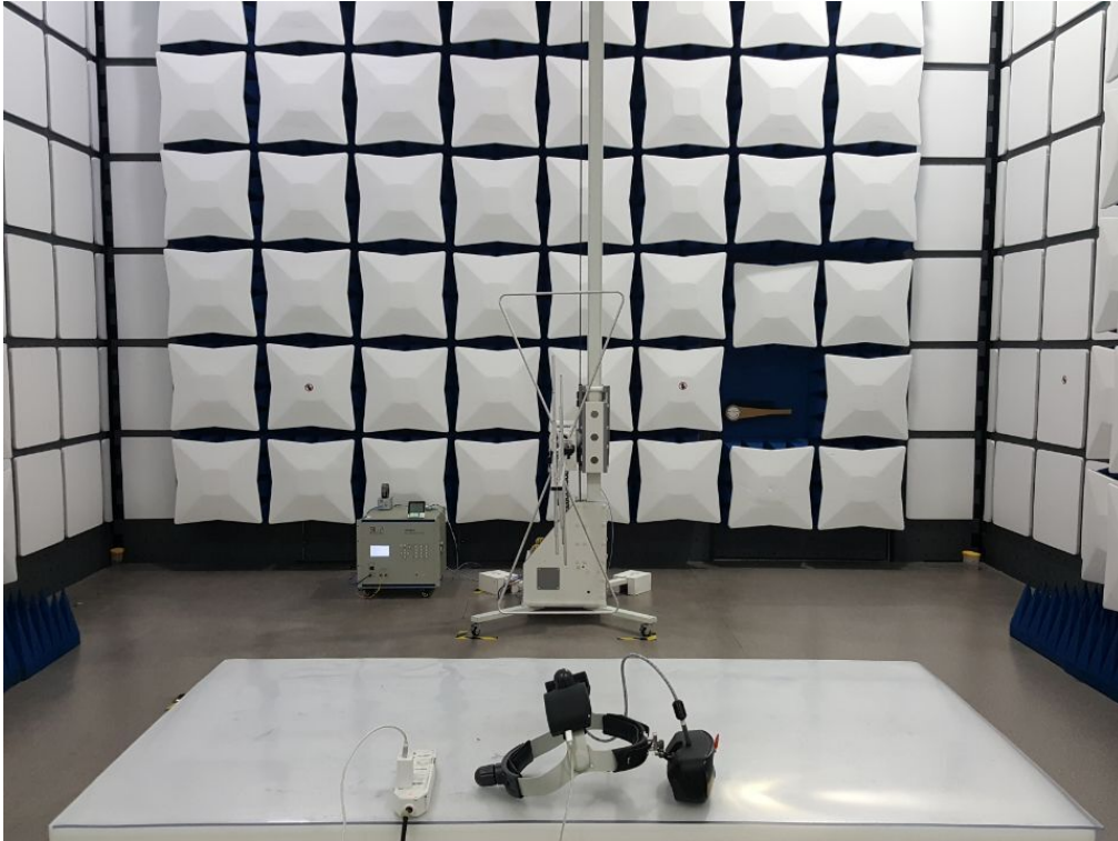
Radiated Emissions: Above 1000MHz
