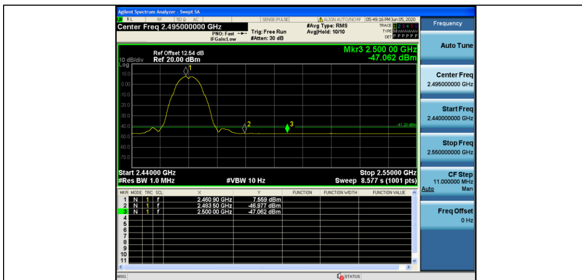
11B_Ant1_High_2462_AV
