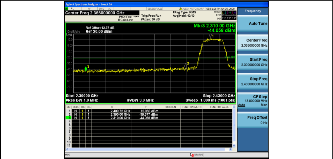
11G_Ant1_Low_2412_Peak
