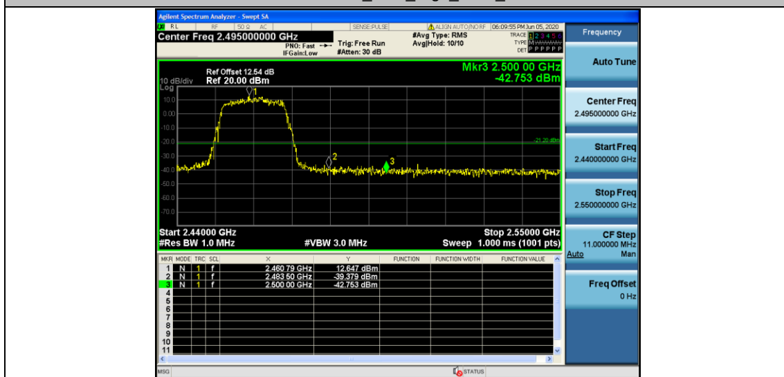
11N20MIMO_Ant1_High_2462_Peak
