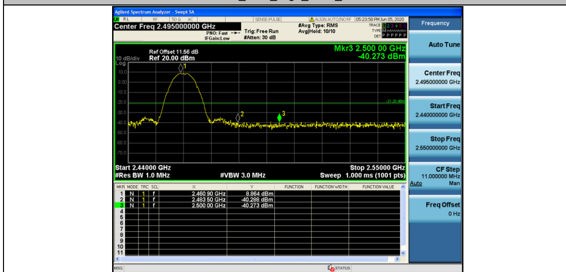
11B_Ant0_High_2462_Peak
