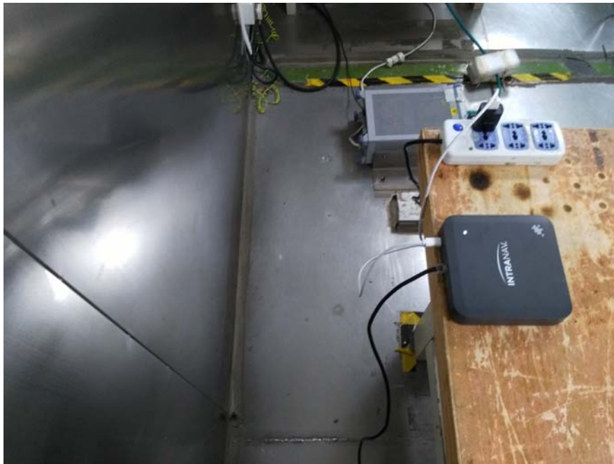
Conducted Emissions - Side View (Type-c)
