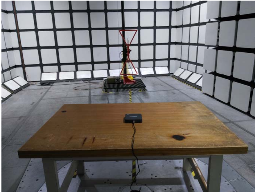
Radiated Emissions View (Below 1 GHz, POE)
