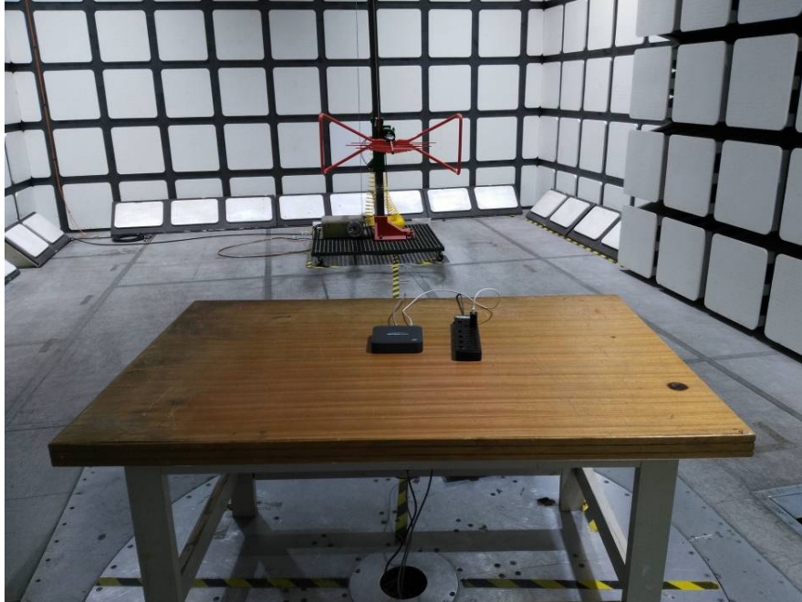
Radiated Emissions View (Below 1 GHz, Type-c)
