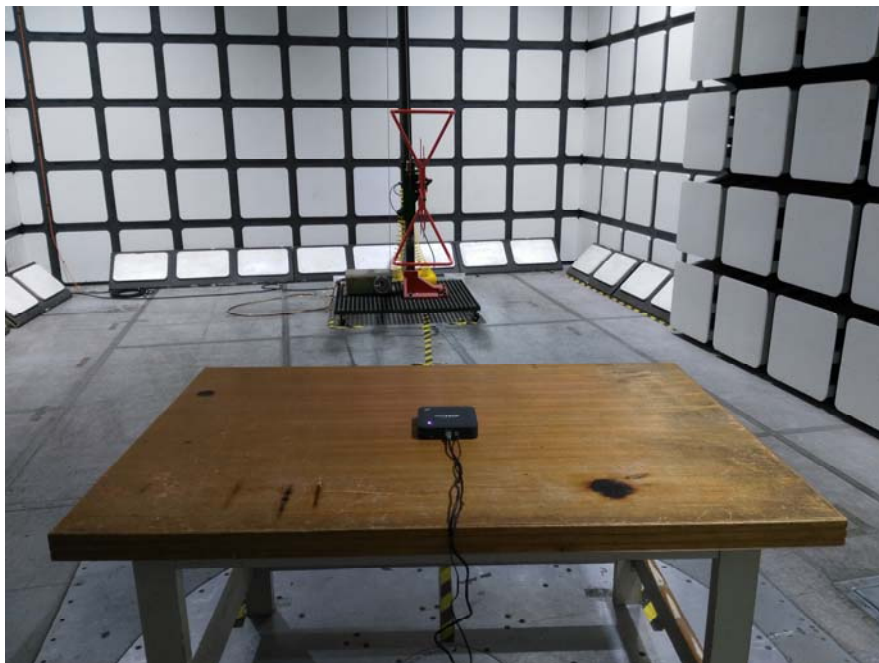
Radiated Emissions View (Below 1 GHz, DC port)
