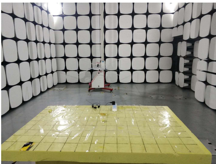
Test Photo
