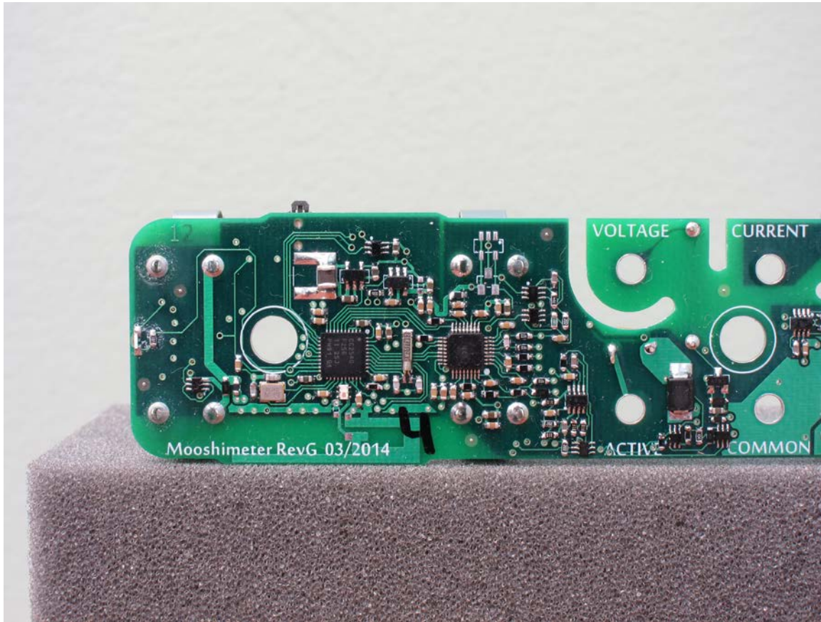
PCB Rear
