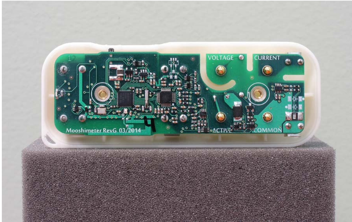
PCB Rear
