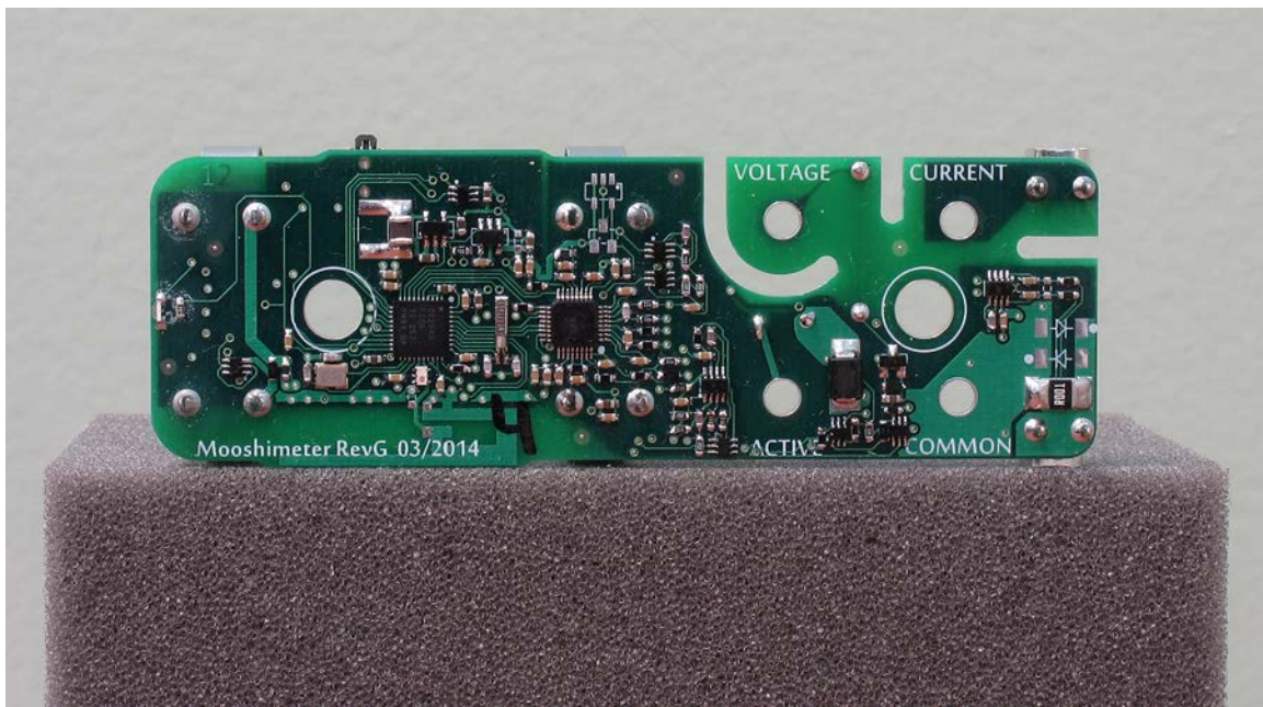
PCB Rear
