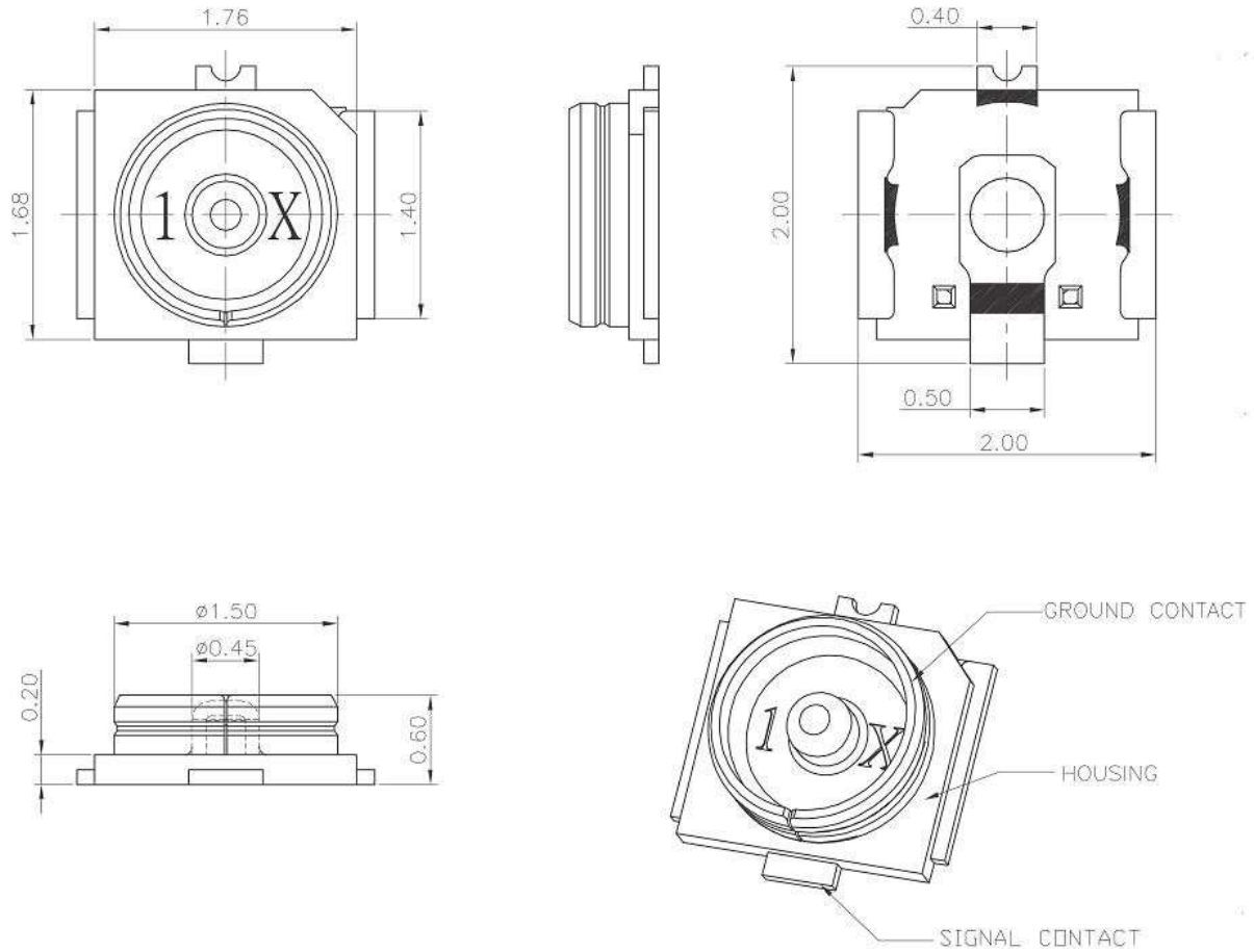
Figure 7-3 RF connector
