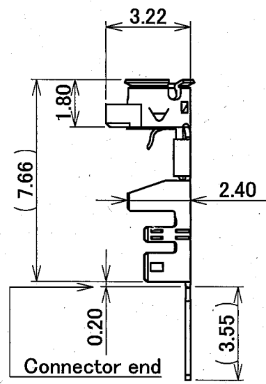
Part No. 20351-111R-37 20351-112R-37 For semi auto termination machine (without notch)
