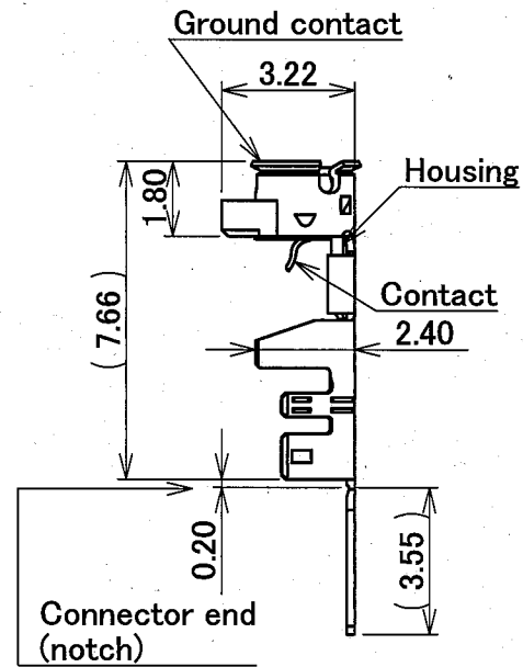
Part No. 20351-101R-37 20351-102R-37 For hand tool (with notch)
