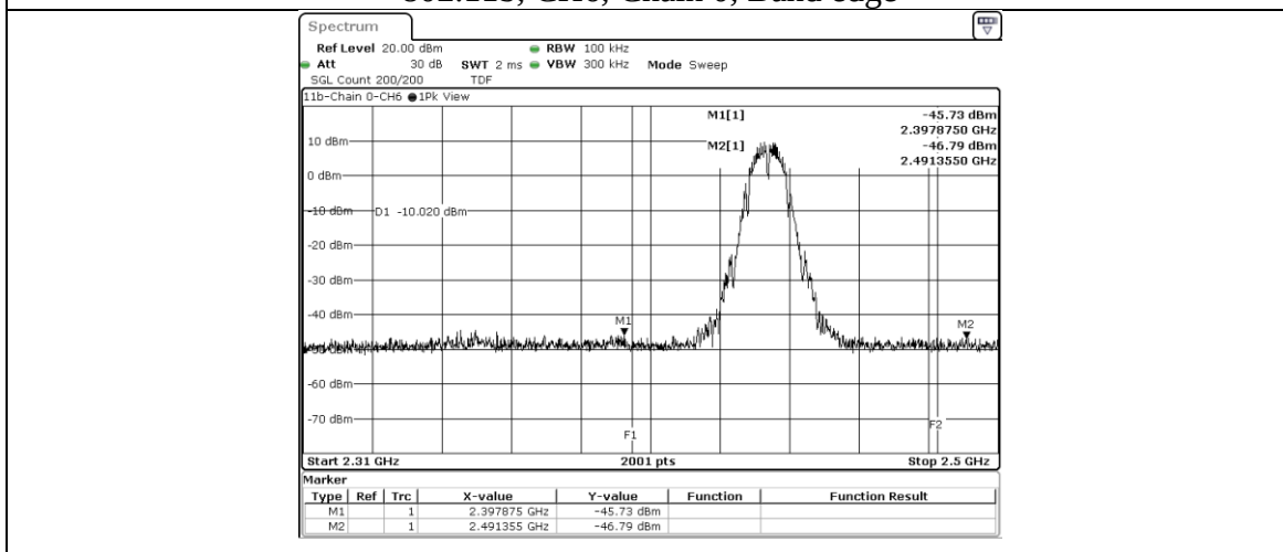
802.11b, CH6, Chain 0, Band edge
