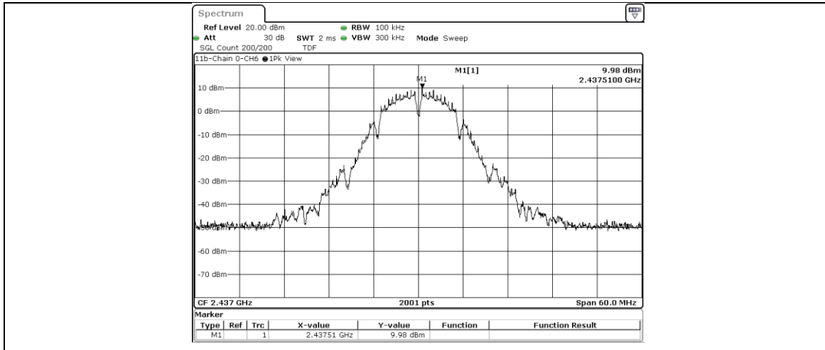
802.11b, CH6, Chain 0, Conducted Emission
