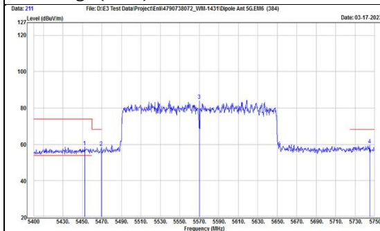
TX, 802.11ax(HE160) (Ch 114) Band Edge (Peak), Horizontal
