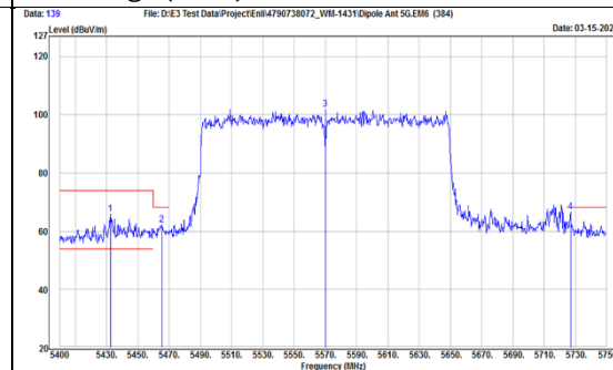
TX, 802.11ax(HE160) (Ch 114) Band Edge (Peak), Vertical
