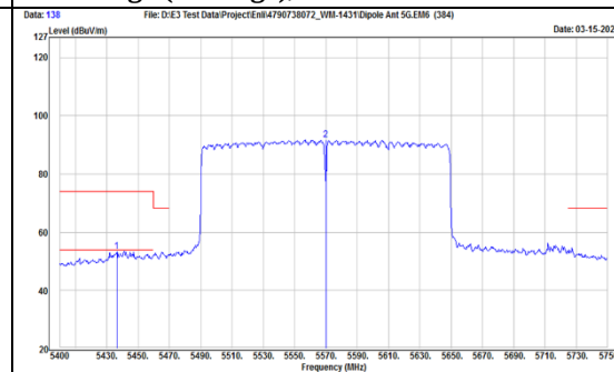
TX, 802.11ax(HE160) (Ch 114) Band Edge (Peak), Vertical
