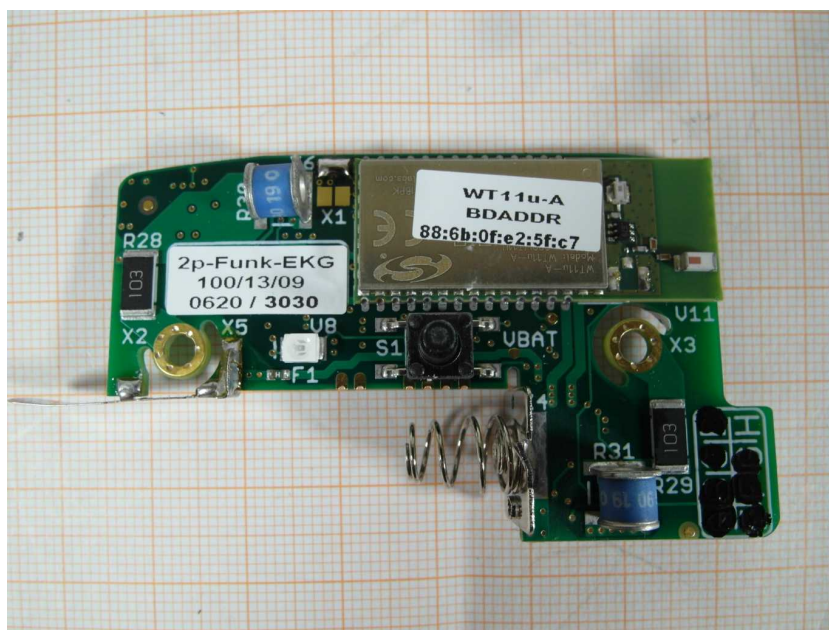
Photo 2: PCB front side view
