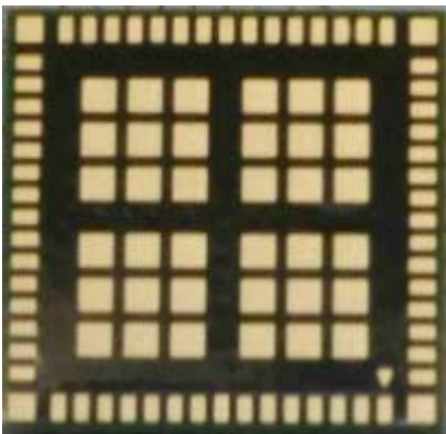
Figure 9.2 – Bottom View
