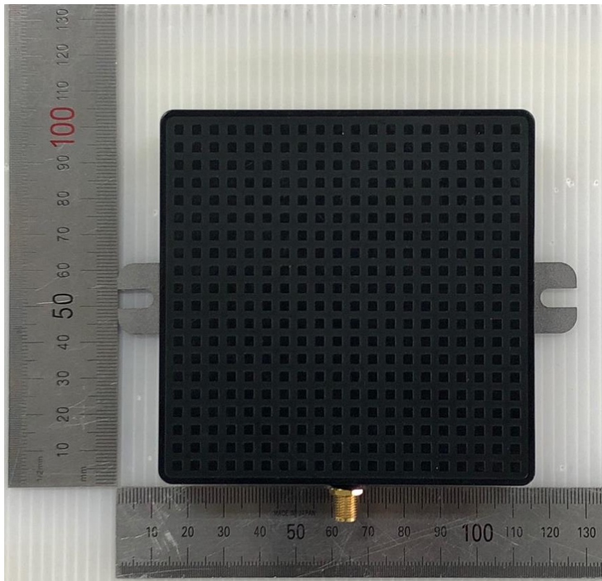
RFID Antenna 6 (M/N: MNFA1010-900L)
