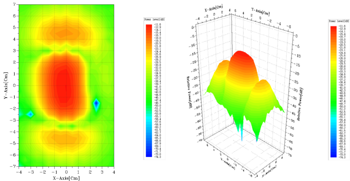
2D and 3D Power distribution at Z=2 cm from Radome
