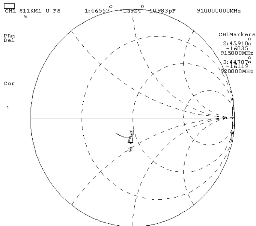
AP44-RFID-UHF Ant Smith chart
