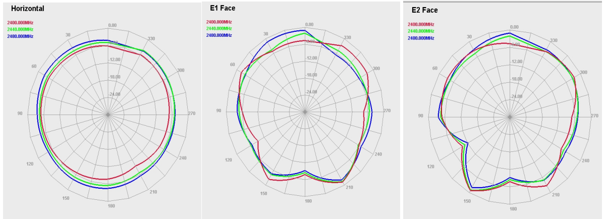
Antenna Field Strength Diagram 2D Diagram
