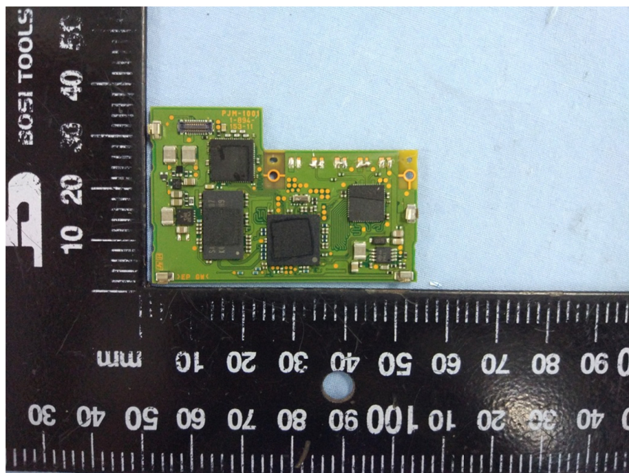
Solder Board-Component View 30
