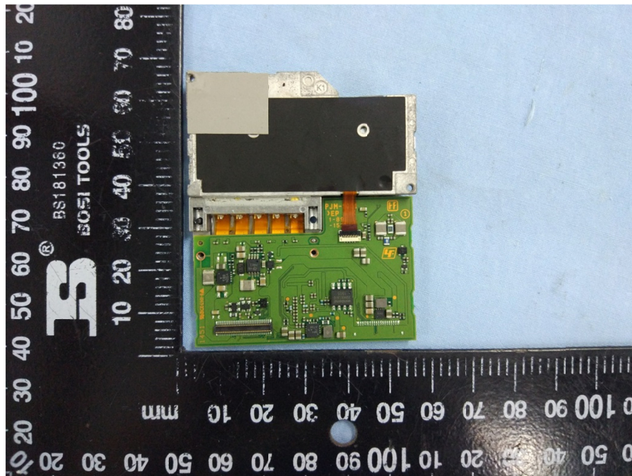
Solder Board-Component View 29
