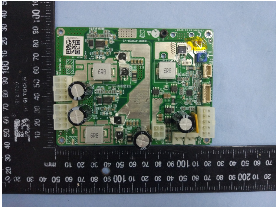
Solder Board-Component View 33
