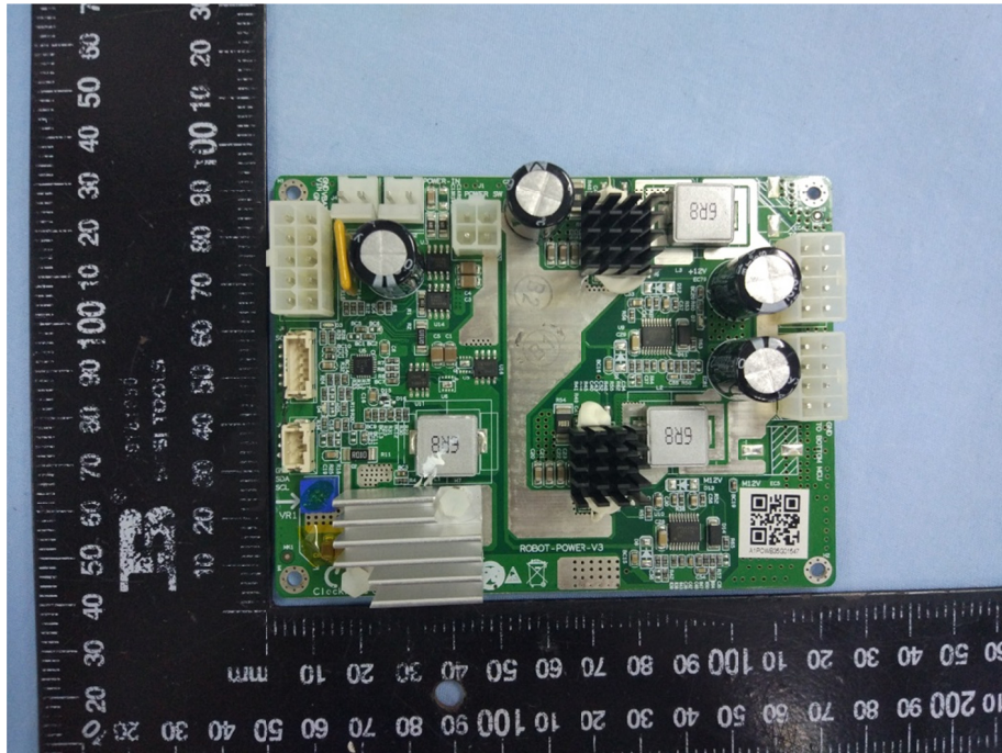
Solder Board-Component View 31
