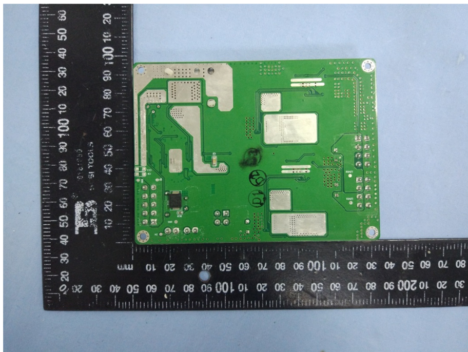
Solder Board-Component View 32
