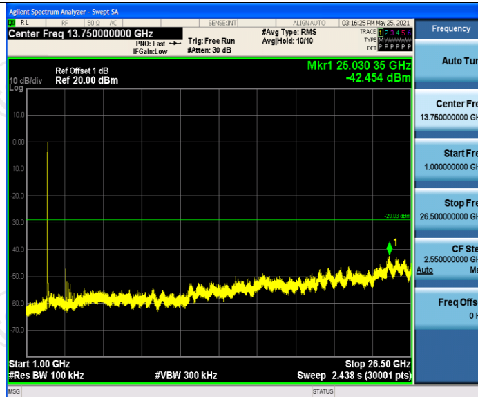
11G Ant1_2437_0-Reference
