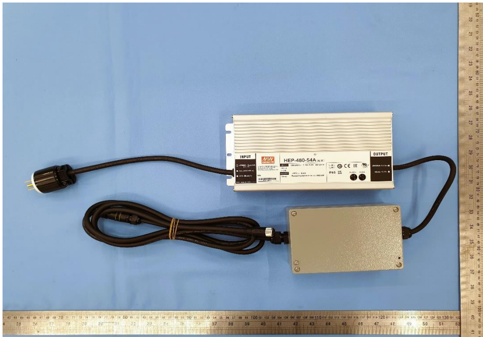
EUT Photo (23)
