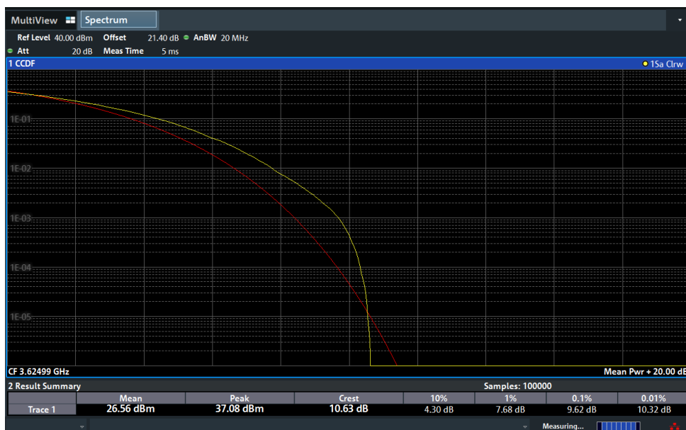
10 MHz_641666_3.1_CCDF_Ant2
