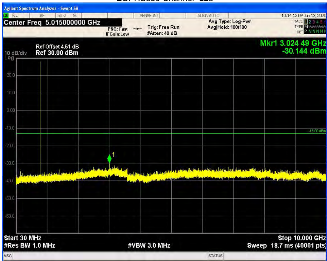
EGPRS850 Channel=251
