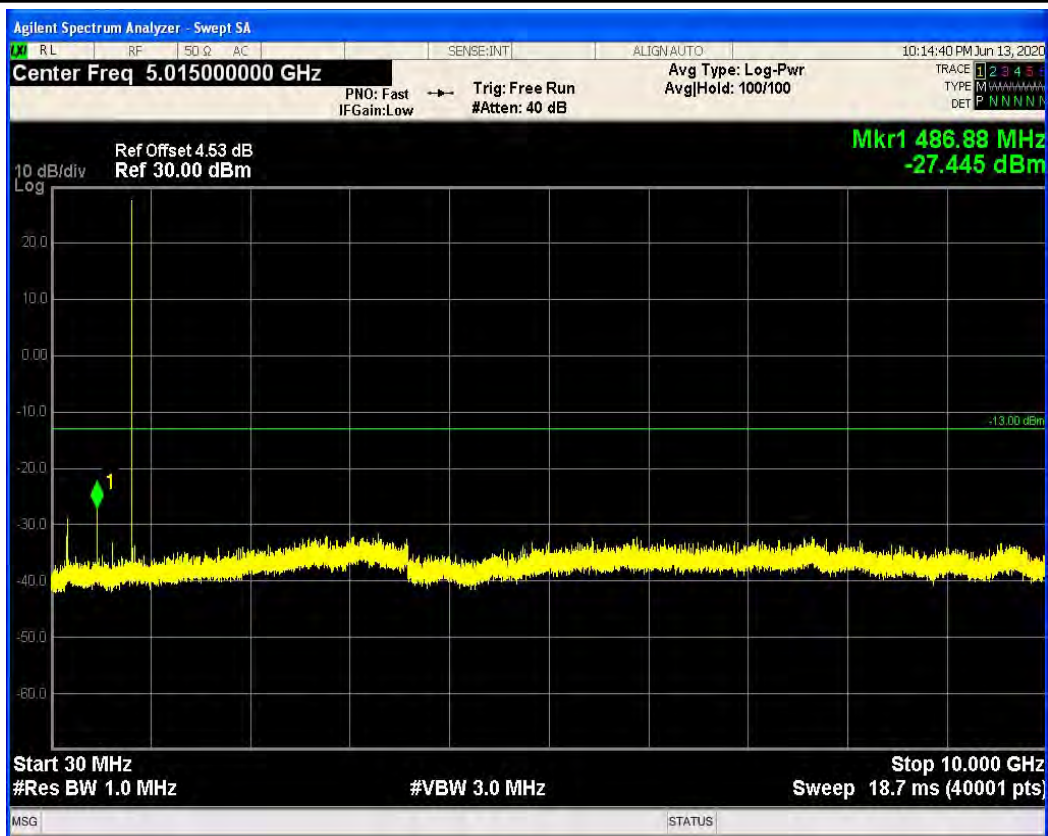
EGPRS850 Channel=128
