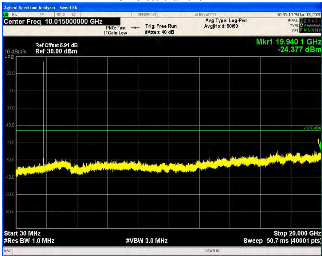
EGPRS1900 Channel=661
