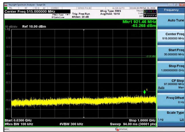
30MHz-1GHz
