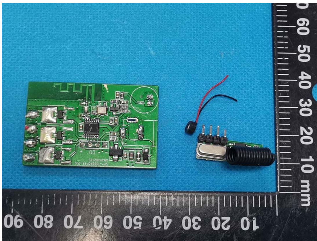
RC Receiver Board
