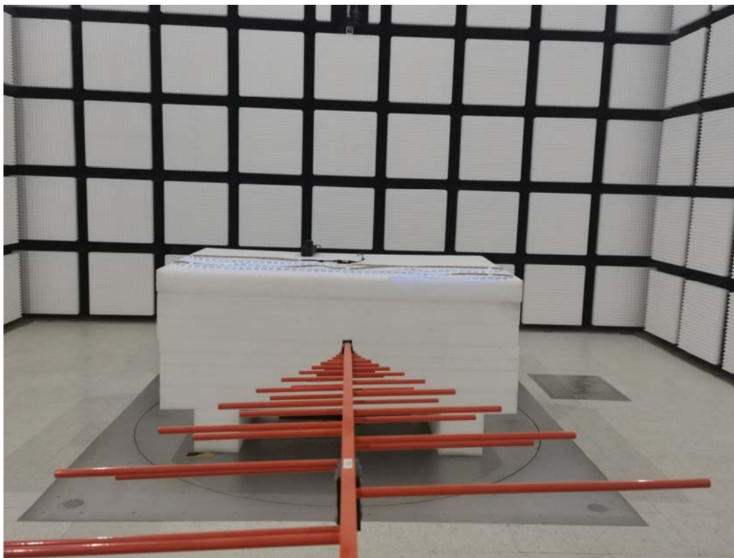
Radiated Emission Below 1GHz View Model: NTS22A-RGB-US-NF
