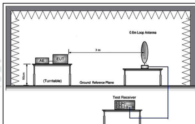
Figure 1. Below 30MHz
