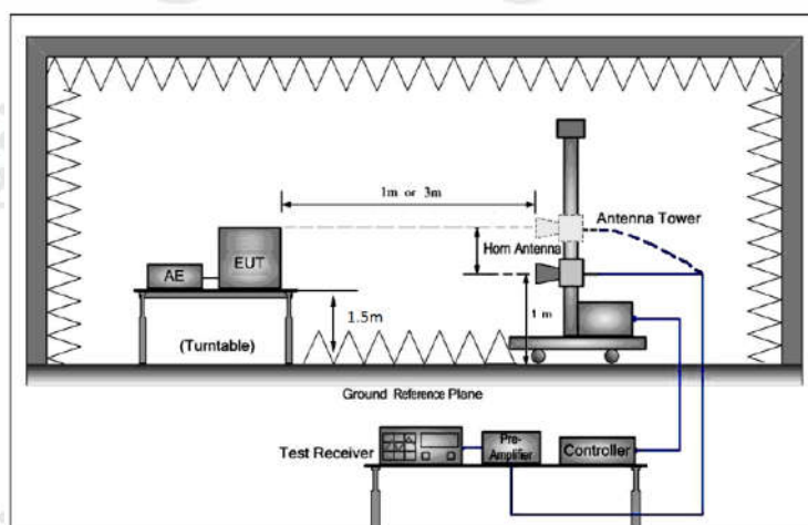
Figure 3. Above 1 GHz
