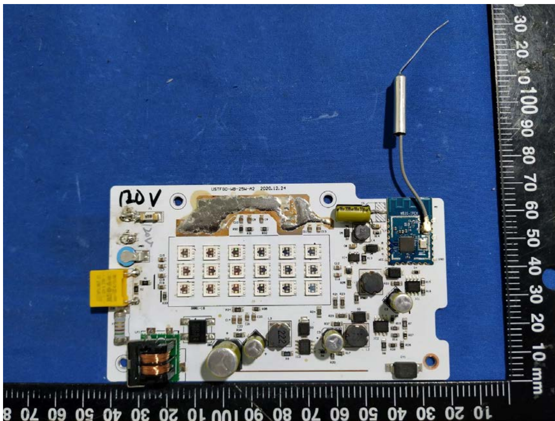
WIFI Antenna
