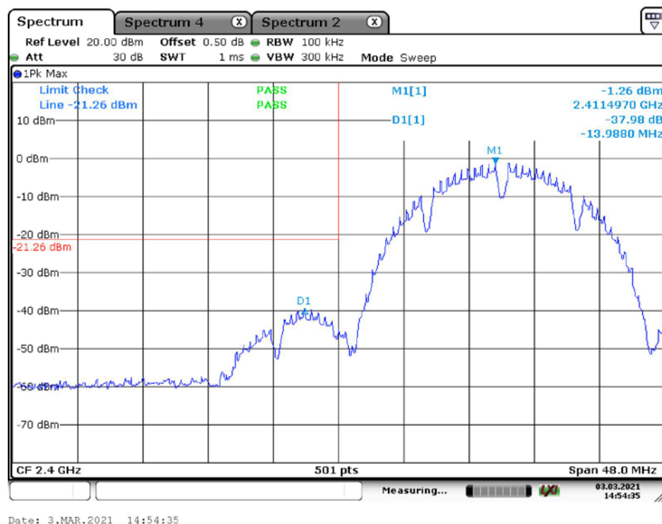
802.11b: Band Edge, Left Side
