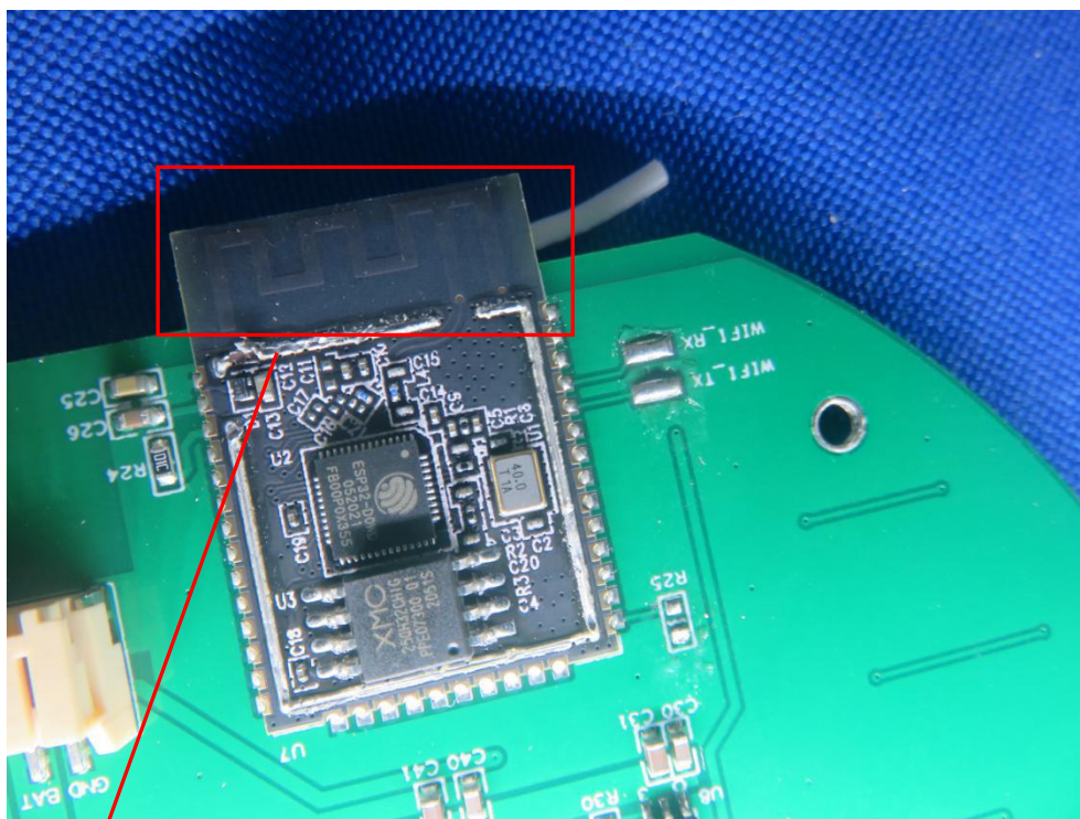
WIFI ANT
