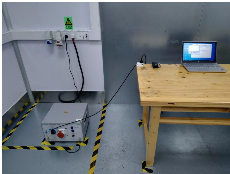
Conducted Emission
