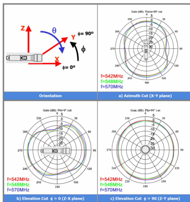
Radiation Pattern
