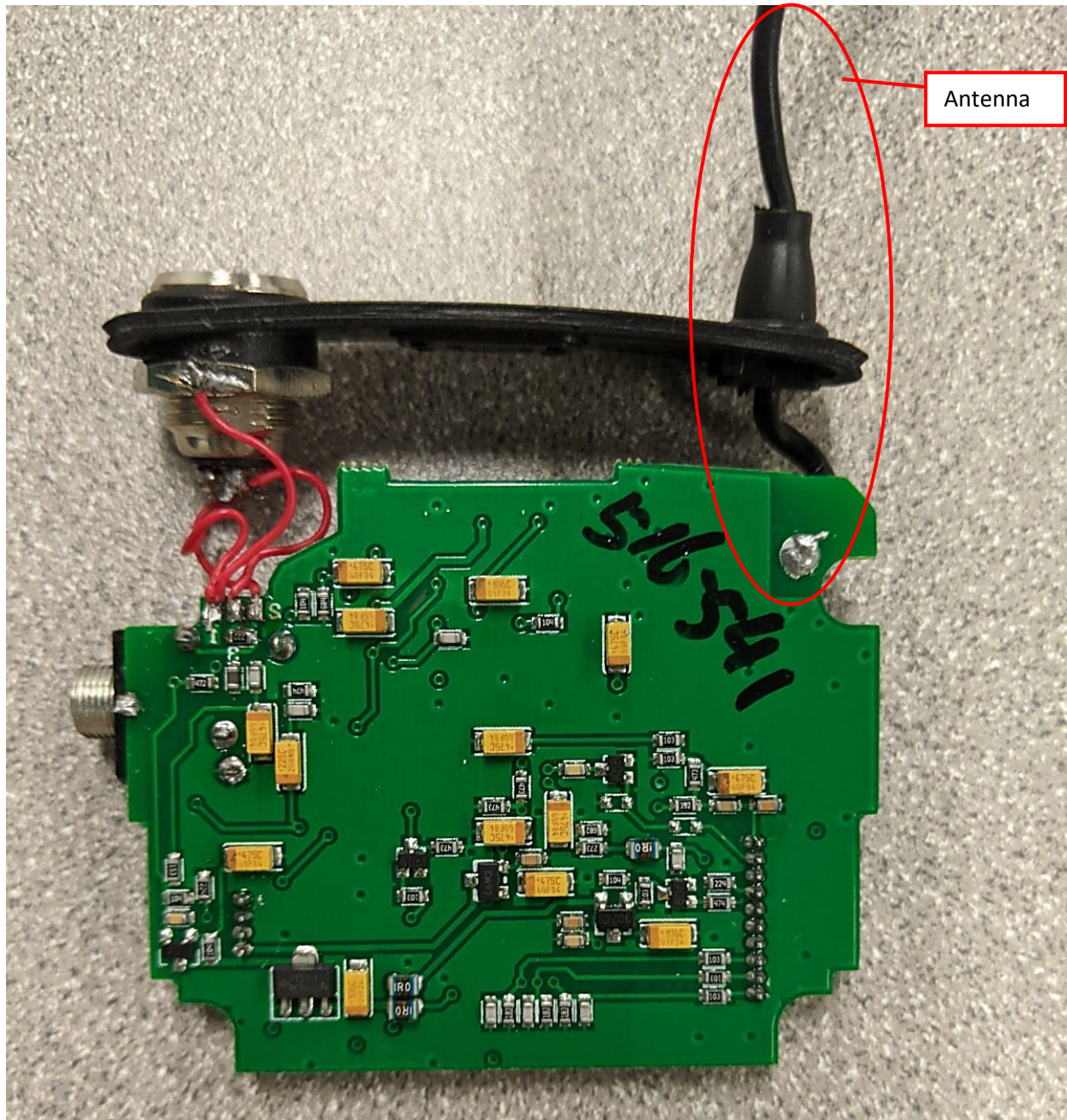
RF PCB Back
