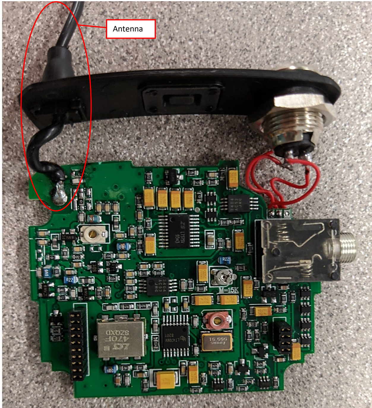
RF PCB Front
