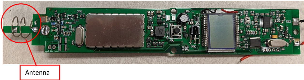
PCB front, Shield removed
