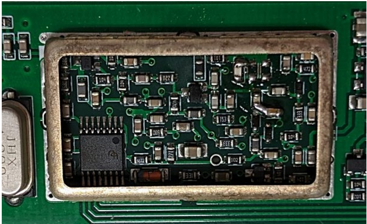
PCB Back
