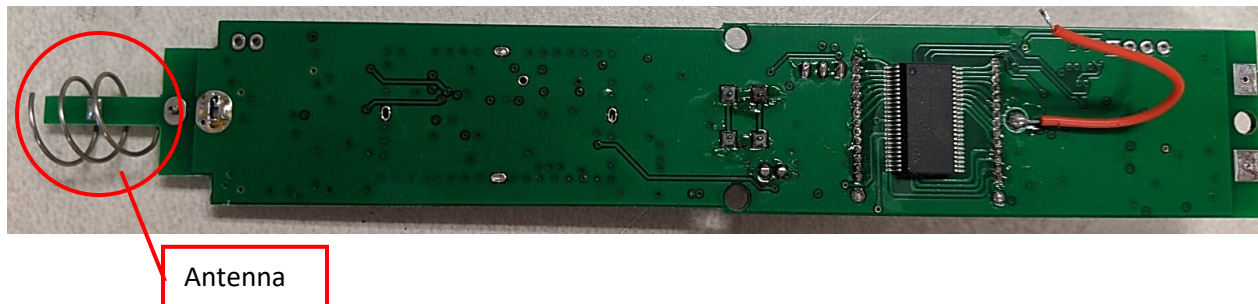
PCB Back
