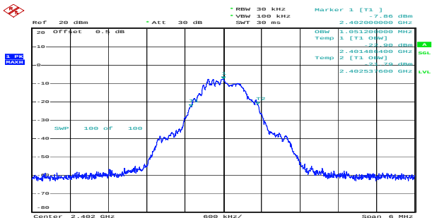
Low 1.051MHz
