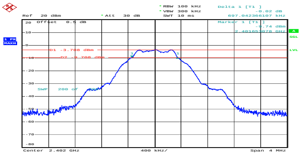
Low 0.697MHz
