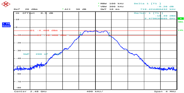
High 0.719MHz
