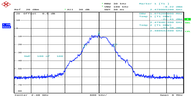
High 1.075MHz
