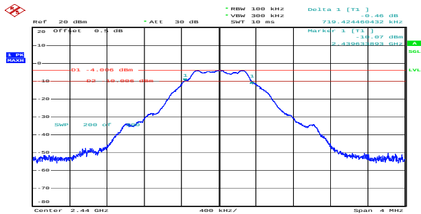
Middle 0.719MHz
