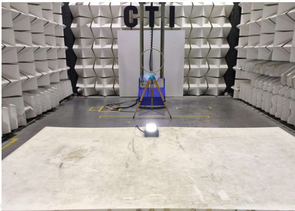
Radiated spurious emission Test Setup-1(Below 30MHz)
