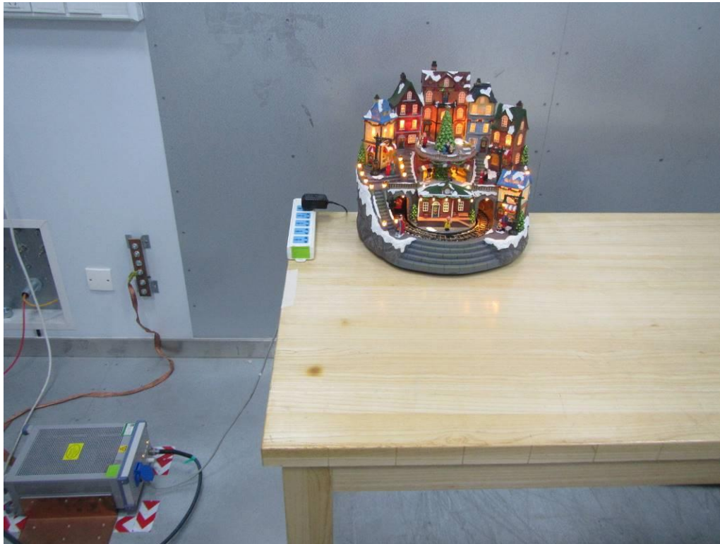
Conducted Emissions test setup photo
