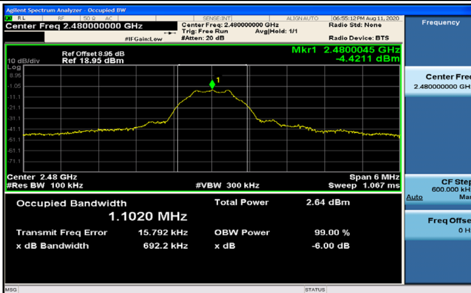
6dB Bandwidth_BLE_2480
