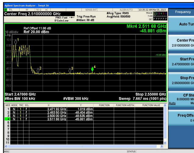
DH5-Ant1-High-Hop_2480-1.02
